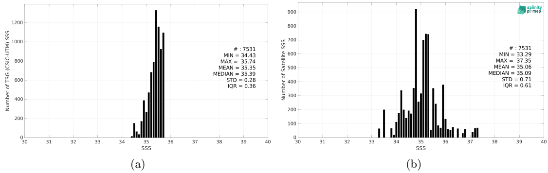
Figure 2: Histograms of SSS from TSG (CSIC-UTM) (a) and SMOS SSS L2Q v331 - With FLAG (CMEMS-CATDS-CPDC) (b) considering all match-up pairs per bins of 0.1 over the South Pacific Ocean Pi-MEP region and for the full satellite product period.
