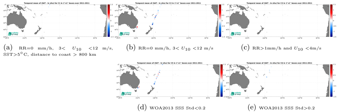
Figure 12: Temporal mean gridded over spatial boxes of size 1^{\circ}\times 1^{\circ} of \Delta\text{SSS} (SMOS SSS L2Q v331 - With FLAG (CMEMS-CATDS-CPDC) - TSG (CSIC-UTM)) for 5 different subdatasets corresponding to:RR=0 mm/h, 3 < U_{10} < 12 m/s, SST >5^{\circ}\text{C} , distance to coast > 800 km (a), RR=0 mm/h, 3 < U_{10} < 12 m/s (b), RR >1 mm/h and U_{10} < 4 m/s (c), WOA2013 SSS Std <0.2 (d), WOA2013 SSS Std >0.2 (e).
