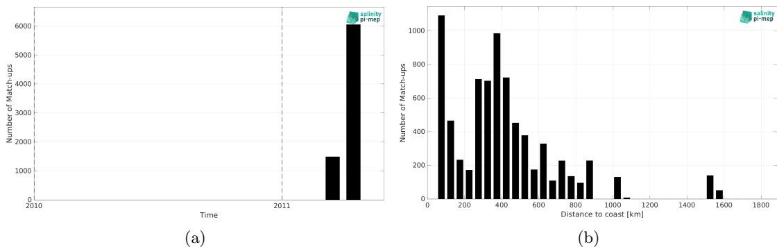
Figure 1: Number of match-ups between TSG (CSIC-UTM) and SMOS SSS L2Q v331 - With FLAG (CMEMS-CATDS-CPDC) SSS as a function of time (a) and as function of the distance to coast (b) over the South Pacific Ocean Pi-MEP region and for the full satellite product period.
