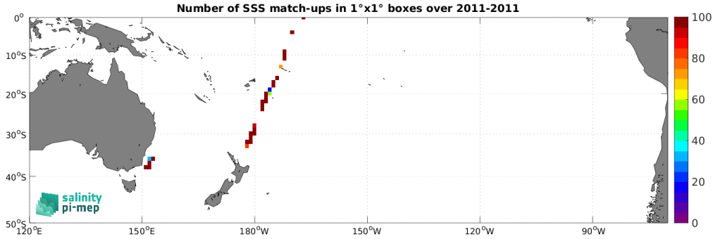
Figure 4: Number of SSS match-ups between TSG (CSIC-UTM) SSS and the SMOS SSS L2Q v331 - With FLAG (CMEMS-CATDS-CPDC) SSS product for the South Pacific Ocean Pi-MEP region over 1^\circ \times 1^\circ boxes and for the full satellite product period.
