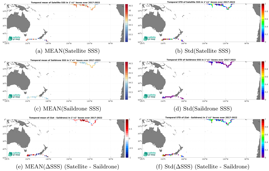
Figure 7: Temporal mean (left) and Std (right) of SSS from SMOS SSS L2Q v331 - With FLAG (CMEMS-CATDS-CPDC) (top), Saildrone (middle), and of \Delta SSS (Satellite - Saildrone). Only match-up pairs are used to generate these maps.
