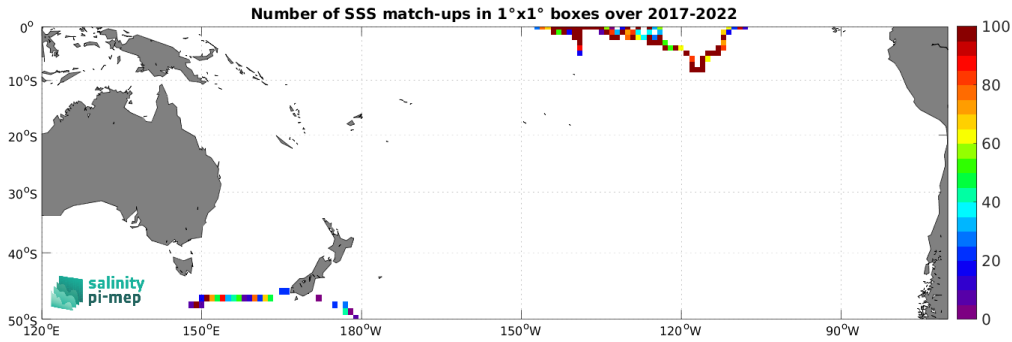
Figure 5: Number of SSS match-ups between Saildrone SSS and the SMOS SSS L2Q v331 - With FLAG (CMEMS-CATDS-CPDC) SSS product for the South Pacific Ocean Pi-MEP region over 1^\circ \times 1^\circ boxes and for the full satellite product period.
