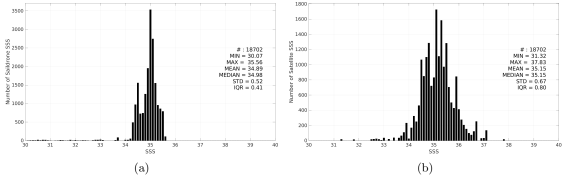
Figure 3: Histograms of SSS from Saildrone (a) and SMOS SSS L2Q v331 - With FLAG (CMEMS-CATDS-CPDC) (b) considering all match-up pairs per bins of 0.1 over the South Pacific Ocean Pi-MEP region and for the full satellite product period.
