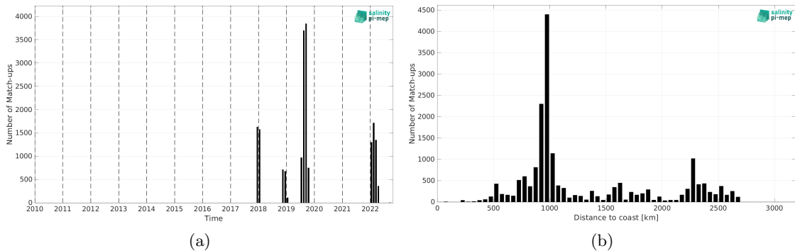
Figure 2: Number of match-ups between Saildrone and SMOS SSS L2Q v331 - With FLAG (CMEMS-CATDS-CPDC) SSS as a function of time (a) and as function of the distance to coast (b) over the South Pacific Ocean Pi-MEP region and for the full satellite product period.
