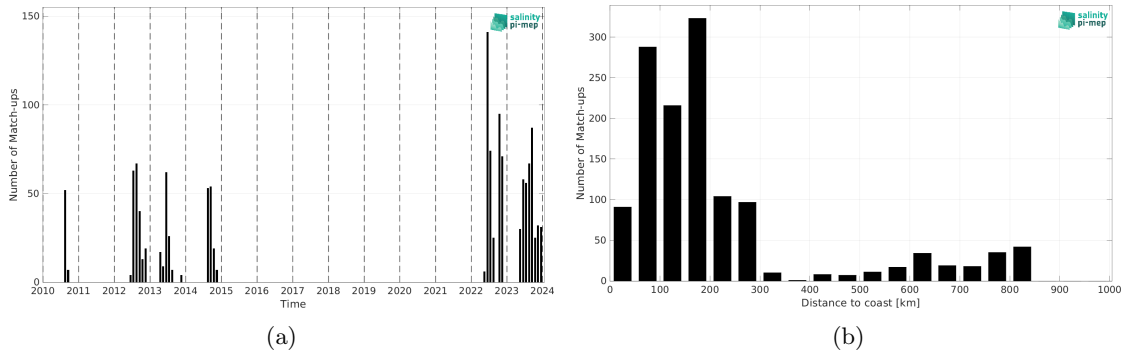
Figure 2: Number of match-ups between Marine mammals and SMOS SSS L2Q v331 - With FLAG (CMEMS-CATDS-CPDC) SSS as a function of time (a) and as function of the distance to coast (b) over the South Pacific Ocean Pi-MEP region and for the full satellite product period.
