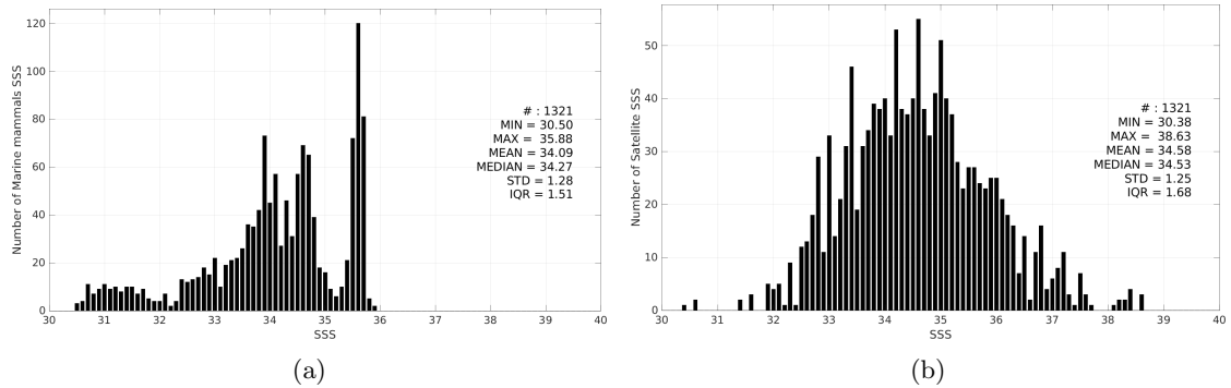
Figure 3: Histograms of SSS from Marine mammals (a) and SMOS SSS L2Q v331 - With FLAG (CMEMS-CATDS-CPDC) (b) considering all match-up pairs per bins of 0.1 over the South Pacific Ocean Pi-MEP region and for the full satellite product period.
