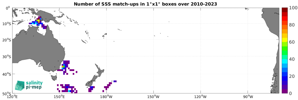
Figure 5: Number of SSS match-ups between Marine mammals SSS and the SMOS SSS L2Q v331 - With FLAG (CMEMS-CATDS-CPDC) SSS product for the South Pacific Ocean Pi-MEP region over 1^\circ \times 1^\circ boxes and for the full satellite product period.
