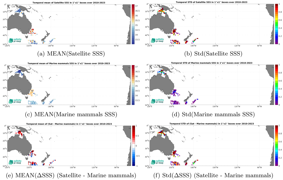
Figure 7: Temporal mean (left) and Std (right) of SSS from SMOS SSS L2Q v331 - With FLAG (CMEMS-CATDS-CPDC) (top), Marine mammals (middle), and of \Delta SSS (Satellite - Marine mammals). Only match-up pairs are used to generate these maps.
