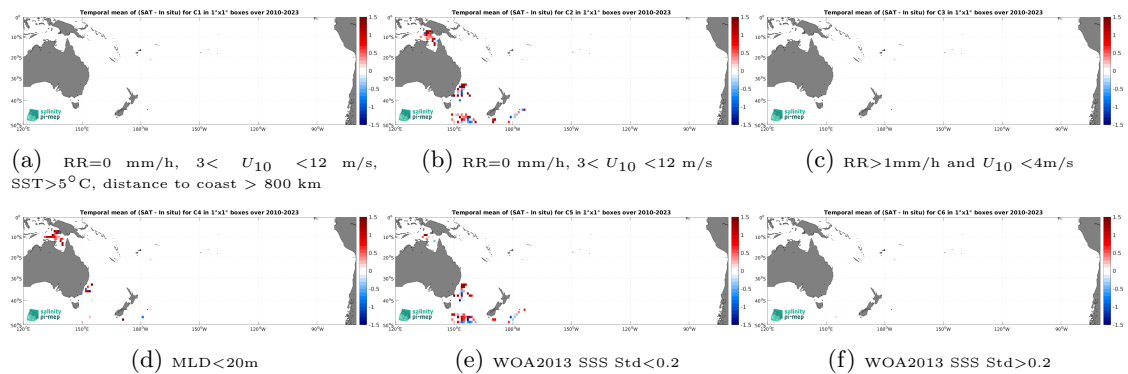
Figure 14: Temporal mean gridded over spatial boxes of size 1^\circ \times 1^\circ of \Delta SSS (SMOS SSS L2Q v331 - With FLAG (CMEMS-CATDS-CPDC) - Marine mammals) for 6 different subdatasets corresponding to:RR=0 mm/h, 3 < U_{10} < 12 m/s, SST >5^\circ C, distance to coast > 800 km (a), RR=0 mm/h, 3 < U_{10} < 12 m/s (b), RR >1 mm/h and U_{10} < 4 m/s (c),MLD <20 m (d),WOA2013 SSS Std <0.2 (e),WOA2013 SSS Std >0.2 (f).
