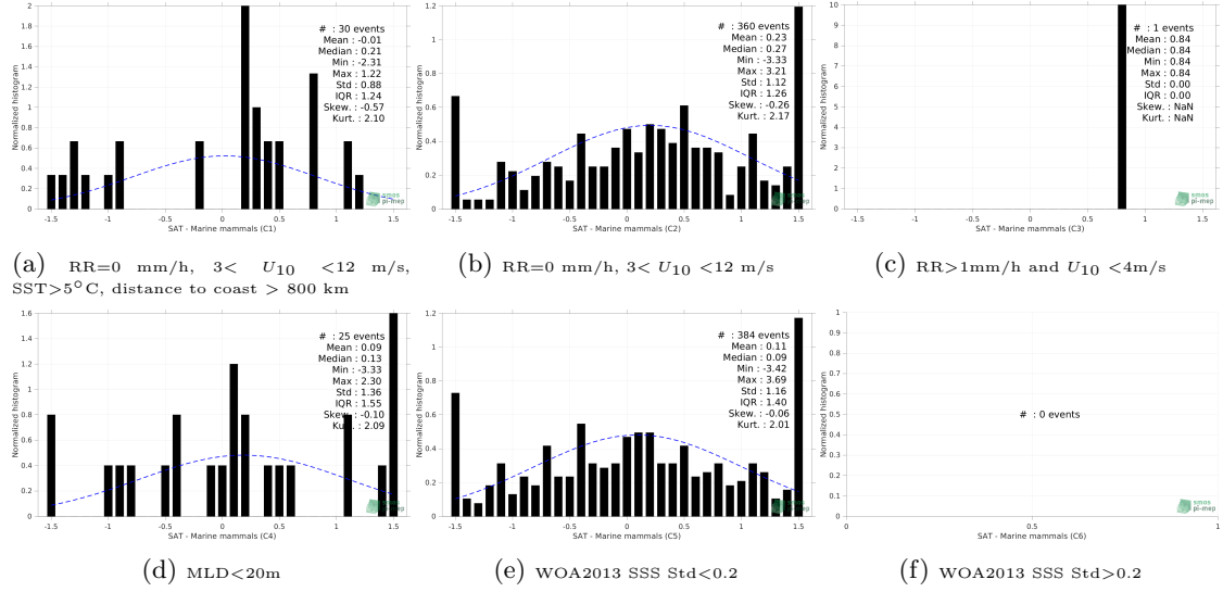
Figure 13: Normalized histogram of \Delta\text{SSS} (SMOS SSS L2Q v331 - With FLAG (CMEMS-CATDS-CPDC) - Marine mammals) for 6 different subdatasets corresponding to: RR=0 mm/h, 3 < U_{10} < 12 m/s, SST > 5^\circ\text{C} , distance to coast > 800 km (a), RR=0 mm/h, 3 < U_{10} < 12 m/s (b), RR > 1\text{mm/h} and U_{10} < 4\text{m/s} (c), MLD < 20\text{m} (d), WOA2013 SSS Std < 0.2 (e), WOA2013 SSS Std > 0.2 (f).
