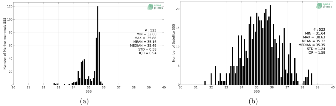
Figure 2: Histograms of SSS from Marine mammals (a) and SMOS SSS L2Q v331 - With FLAG (CMEMS-CATDS-CPDC) (b) considering all match-up pairs per bins of 0.1 over the South Pacific Ocean Pi-MEP region and for the full satellite product period.
