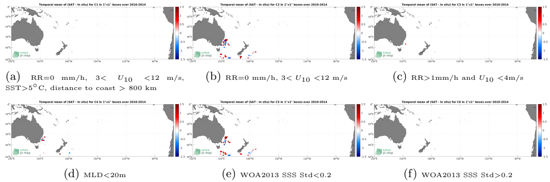
Figure 12: Temporal mean gridded over spatial boxes of size 1^{\circ}\times 1^{\circ} of \Delta\text{SSS} (SMOS SSS L2Q v331 - With FLAG (CMEMS-CATDS-CPDC) - Marine mammals) for 6 different subdatasets corresponding to:RR=0 mm/h, 3 < U_{10} < 12 m/s, SST >5^{\circ}\text{C} , distance to coast > 800 km (a), RR=0 mm/h, 3 < U_{10} < 12 m/s (b), RR >1 mm/h and U_{10} < 4 m/s (c),MLD <20 m (d),WOA2013 SSS Std <0.2 (e),WOA2013 SSS Std >0.2 (f).
