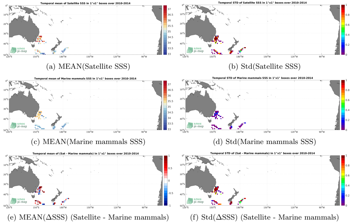
Figure 6: Temporal mean (left) and Std (right) of SSS from SMOS SSS L2Q v331 - With FLAG (CMEMS-CATDS-CPDC) (top), Marine mammals (middle), and of \Delta SSS (Satellite - Marine mammals). Only match-up pairs are used to generate these maps.
