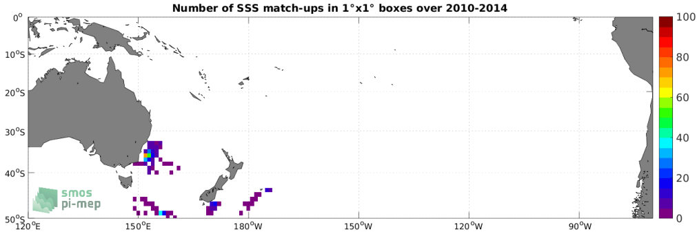
Figure 4: Number of SSS match-ups between Marine mammals SSS and the SMOS SSS L2Q v331 - With FLAG (CMEMS-CATDS-CPDC) SSS product for the South Pacific Ocean Pi-MEP region over 1^\circ \times 1^\circ boxes and for the full satellite product period.
