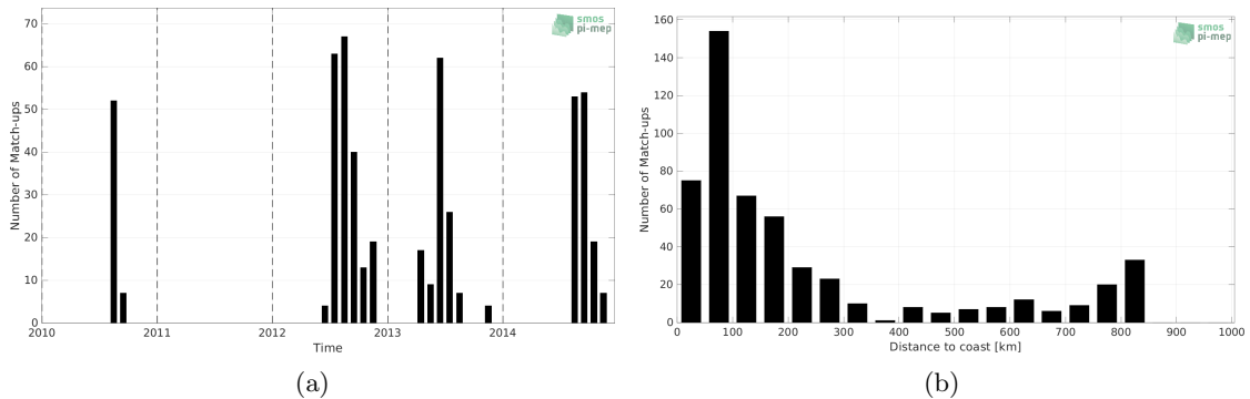
Figure 1: Number of match-ups between Marine mammals and SMOS SSS L2Q v331 - With FLAG (CMEMS-CATDS-CPDC) SSS as a function of time (a) and as function of the distance to coast (b) over the South Pacific Ocean Pi-MEP region and for the full satellite product period.
