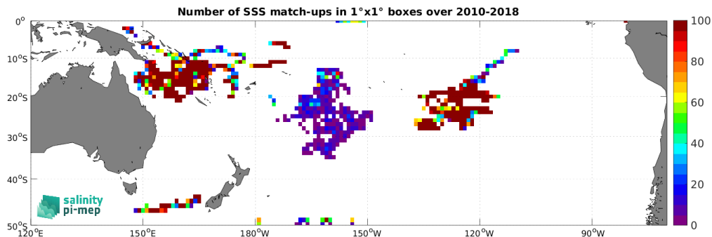
Figure 4: Number of SSS match-ups between Surface drifters SSS and the SMOS SSS L2Q v331 - With FLAG (CMEMS-CATDS-CPDC) SSS product for the South Pacific Ocean Pi-MEP region over 1^\circ \times 1^\circ boxes and for the full satellite product period.
