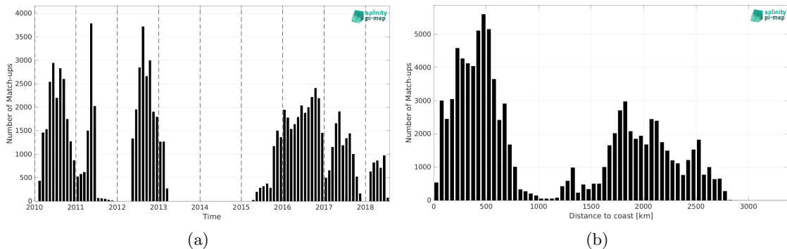
Figure 2: Number of match-ups between Surface drifters and SMOS SSS L2Q v331 - With FLAG (CMEMS-CATDS-CPDC) SSS as a function of time (a) and as function of the distance to coast (b) over the South Pacific Ocean Pi-MEP region and for the full satellite product period.
