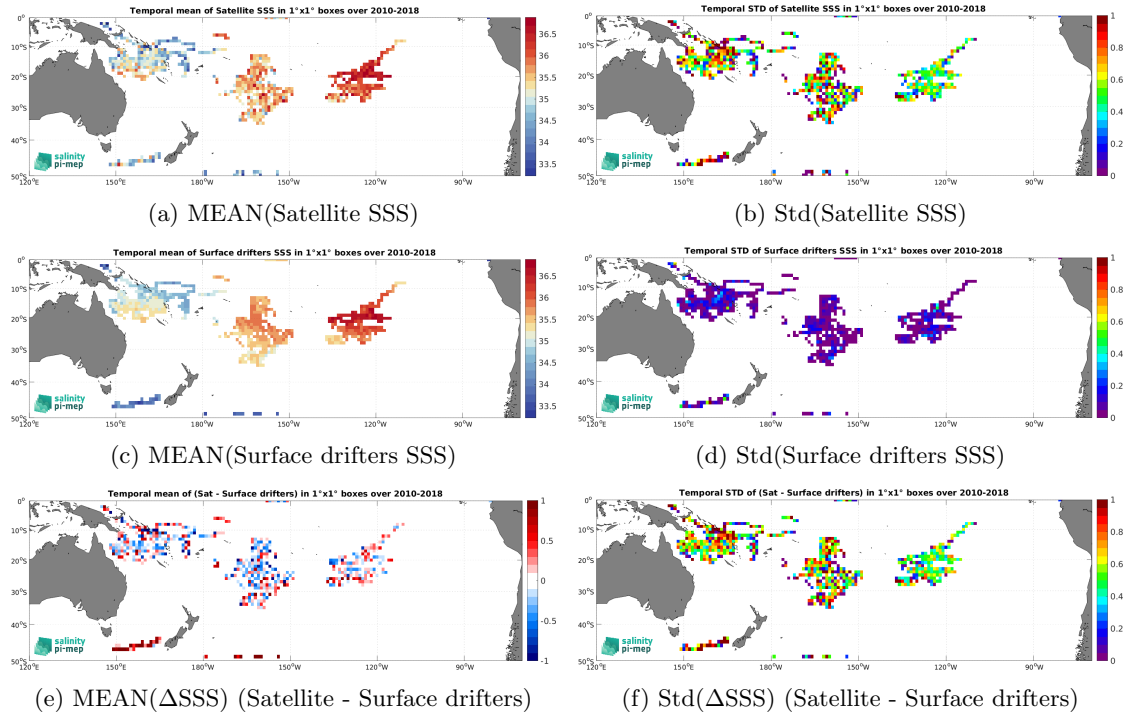
Figure 6: Temporal mean (left) and Std (right) of SSS from SMOS SSS L2Q v331 - With FLAG (CMEMS-CATDS-CPDC) (top), Surface drifters (middle), and of \Delta SSS (Satellite - Surface drifters). Only match-up pairs are used to generate these maps.
