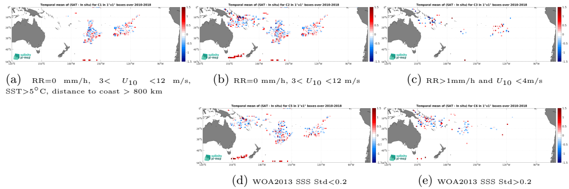
Figure 13: Temporal mean gridded over spatial boxes of size 1^\circ \times 1^\circ of \Delta SSS (SMOS SSS L2Q v331 - With FLAG (CMEMS-CATDS-CPDC) - Surface drifters) for 5 different subdatasets corresponding to:RR=0 mm/h, 3 < U_{10} < 12 m/s, SST >5^\circ\text{C} , distance to coast > 800 km (a), RR=0 mm/h, 3 < U_{10} < 12 m/s (b), RR >1 mm/h and U_{10} < 4 m/s (c), WOA2013 SSS Std <0.2 (d), WOA2013 SSS Std >0.2 (e).
