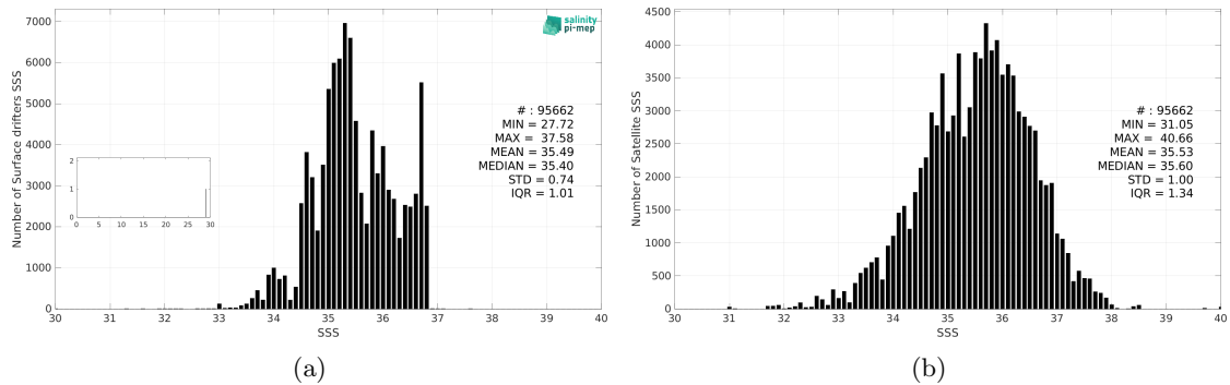
Figure 3: Histograms of SSS from Surface drifters (a) and SMOS SSS L2Q v331 - With FLAG (CMEMS-CATDS-CPDC) (b) considering all match-up pairs per bins of 0.1 over the South Pacific Ocean Pi-MEP region and for the full satellite product period.
