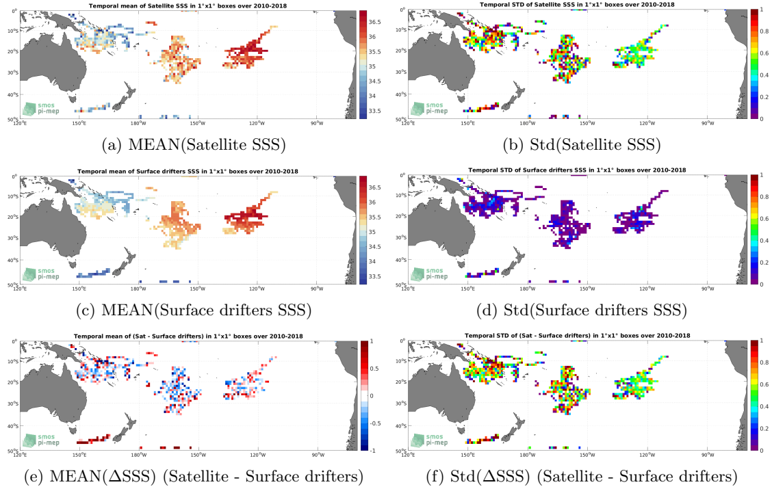
Figure 5: Temporal mean (left) and Std (right) of SSS from SMOS SSS L2Q v331 - With FLAG (CMEMS-CATDS-CPDC) (top), Surface drifters (middle), and of \Delta SSS (Satellite - Surface drifters). Only match-up pairs are used to generate these maps.
