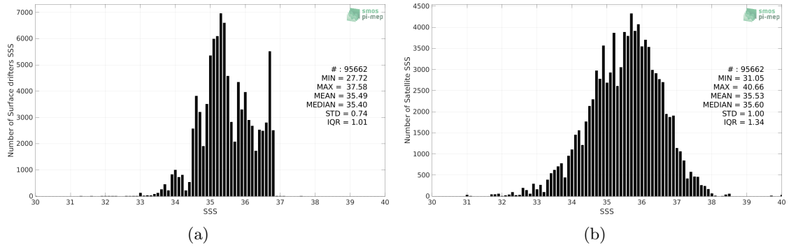
Figure 2: Histograms of SSS from Surface drifters (a) and SMOS SSS L2Q v331 - With FLAG (CMEMS-CATDS-CPDC) (b) considering all match-up pairs per bins of 0.1 over the South Pacific Ocean Pi-MEP region and for the full satellite product period.
