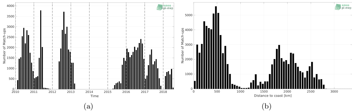
Figure 1: Number of match-ups between Surface drifters and SMOS SSS L2Q v331 - With FLAG (CMEMS-CATDS-CPDC) SSS as a function of time (a) and as function of the distance to coast (b) over the South Pacific Ocean Pi-MEP region and for the full satellite product period.
