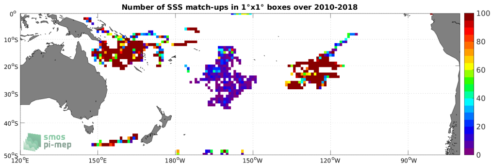
Figure 3: Number of SSS match-ups between Surface drifters SSS and the SMOS SSS L2Q v331 - With FLAG (CMEMS-CATDS-CPDC) SSS product for the South Pacific Ocean Pi-MEP region over 1^\circ \times 1^\circ boxes and for the full satellite product period.
