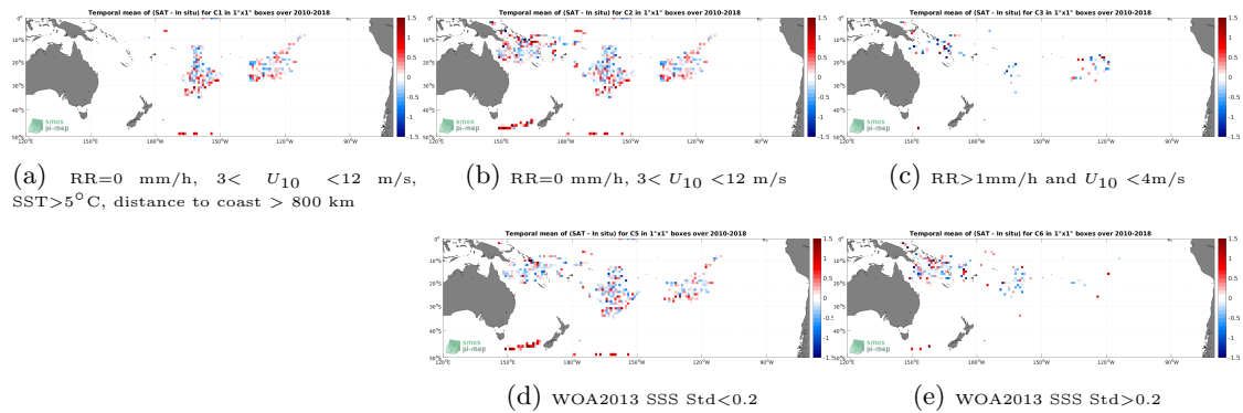
Figure 11: Temporal mean gridded over spatial boxes of size 1^\circ \times 1^\circ of \Delta SSS (SMOS SSS L2Q v331 - With FLAG (CMEMS-CATDS-CPDC) - Surface drifters) for 5 different subdatasets corresponding to:RR=0 mm/h, 3 < U_{10} < 12 m/s, SST >5^\circ C, distance to coast > 800 km (a), RR=0 mm/h, 3 < U_{10} < 12 m/s (b), RR >1 mm/h and U_{10} < 4 m/s (c), WOA2013 SSS Std <0.2 (d), WOA2013 SSS Std >0.2 (e).
