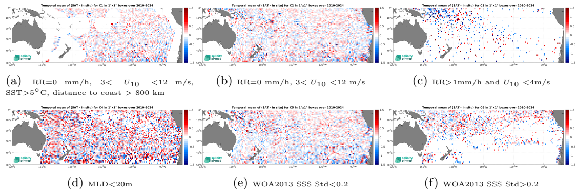
Figure 14: Temporal mean gridded over spatial boxes of size 1^\circ \times 1^\circ of \Delta SSS (SMOS SSS L2Q v331 - With FLAG (CMEMS-CATDS-CPDC) - Argo) for 6 different subdatasets corresponding to: RR=0 mm/h, 3 < U_{10} < 12 m/s, SST > 5°C, distance to coast > 800 km (a), RR=0 mm/h, 3 < U_{10} < 12 m/s (b), RR > 1mm/h and U_{10} < 4 m/s (c), MLD < 20m (d), WOA2013 SSS Std < 0.2 (e), WOA2013 SSS Std > 0.2 (f).
