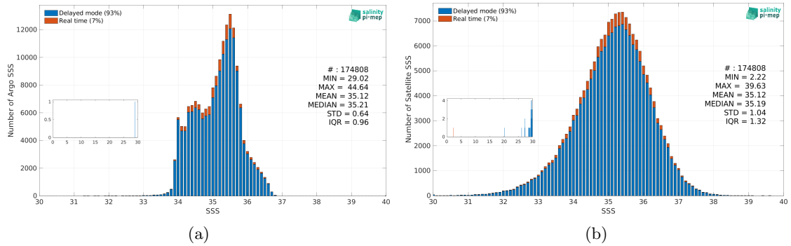
Figure 3: Histograms of SSS from Argo (a) and SMOS SSS L2Q v331 - With FLAG (CMEMS-CATDS-CPDC) (b) considering all match-up pairs per bins of 0.1 over the South Pacific Ocean Pi-MEP region and for the full satellite product period.
