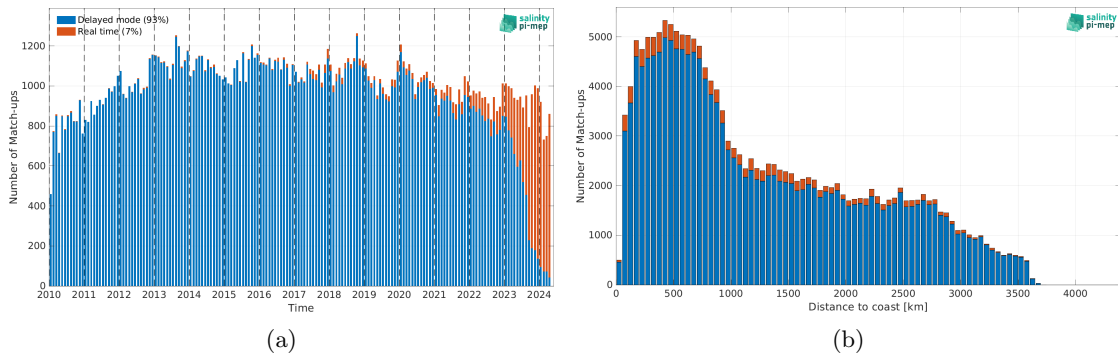
Figure 2: Number of match-ups between Argo and SMOS SSS L2Q v331 - With FLAG (CMEMS-CATDS-CPDC) SSS as a function of time (a) and as function of the distance to coast (b) over the South Pacific Ocean Pi-MEP region and for the full satellite product period.
