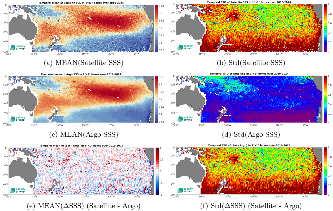
Figure 7: Temporal mean (left) and Std (right) of SSS from SMOS SSS L2Q v331 - With FLAG (CMEMS-CATDS-CPDC) (top), Argo (middle), and of \Delta SSS (Satellite - Argo). Only match-up pairs are used to generate these maps.
