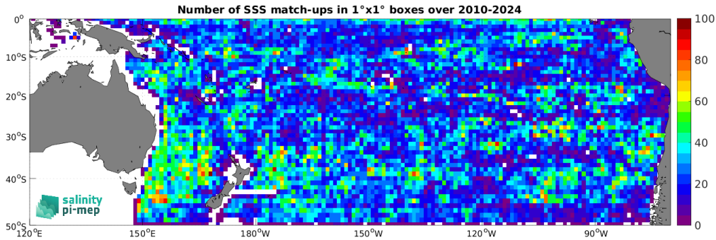
Figure 5: Number of SSS match-ups between Argo SSS and the SMOS SSS L2Q v331 - With FLAG (CMEMS-CATDS-CPDC) SSS product for the South Pacific Ocean Pi-MEP region over 1^\circ \times 1^\circ boxes and for the full satellite product period.
