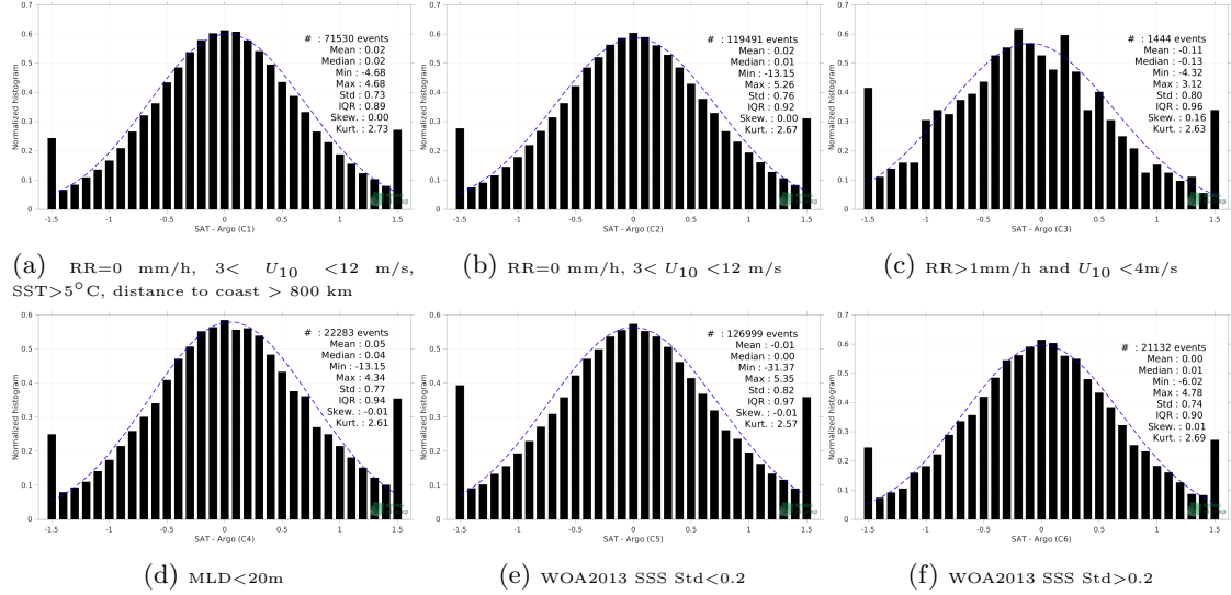
Figure 13: Normalized histogram of \Delta SSS (SMOS SSS L2Q v331 - With FLAG (CMEMS-CATDS-CPDC) - Argo) for 6 different subdatasets corresponding to: RR=0 mm/h, 3 < U_{10} < 12 m/s, SST > 5°C, distance to coast > 800 km (a), RR=0 mm/h, 3 < U_{10} < 12 m/s (b), RR > 1mm/h and U_{10} < 4 m/s (c), MLD < 20m (d), WOA2013 SSS Std < 0.2 (e), WOA2013 SSS Std > 0.2 (f).
