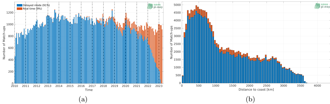
Figure 1: Number of match-ups between Argo and SMOS SSS L2Q v331 - With FLAG (CMEMS-CATDS-CPDC) SSS as a function of time (a) and as function of the distance to coast (b) over the South Pacific Ocean Pi-MEP region and for the full satellite product period.
