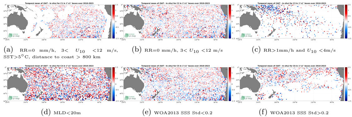
Figure 12: Temporal mean gridded over spatial boxes of size 1^\circ \times 1^\circ of \Delta SSS (SMOS SSS L2Q v331 - With FLAG (CMEMS-CATDS-CPDC) - Argo) for 6 different subdatasets corresponding to:RR=0 mm/h, 3 < U_{10} < 12 m/s, SST >5^\circ\text{C} , distance to coast > 800 km (a), RR=0 mm/h, 3 < U_{10} < 12 m/s (b), RR >1 mm/h and U_{10} < 4 m/s (c),MLD <20 m (d),WOA2013 SSS Std <0.2 (e),WOA2013 SSS Std >0.2 (f).
