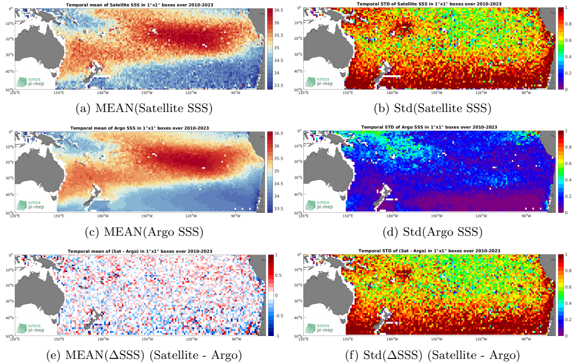
Figure 6: Temporal mean (left) and Std (right) of SSS from SMOS SSS L2Q v331 - With FLAG (CMEMS-CATDS-CPDC) (top), Argo (middle), and of \Delta SSS (Satellite - Argo). Only match-up pairs are used to generate these maps.
