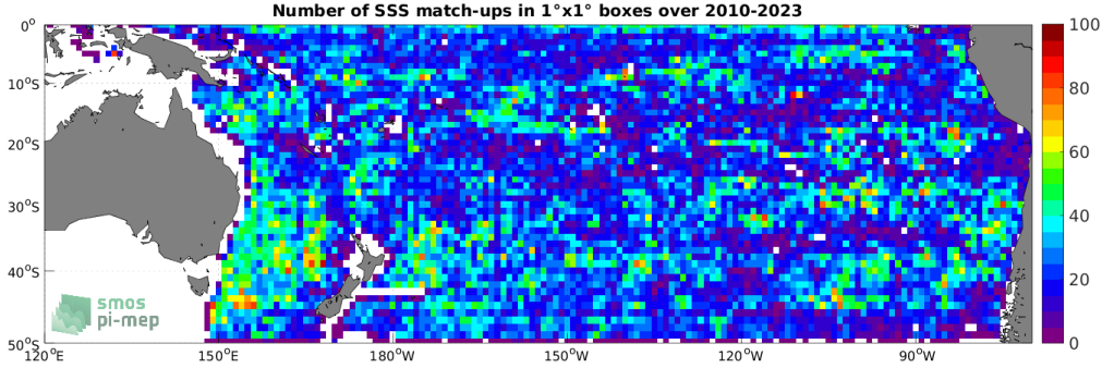
Figure 4: Number of SSS match-ups between Argo SSS and the SMOS SSS L2Q v331 - With FLAG (CMEMS-CATDS-CPDC) SSS product for the South Pacific Ocean Pi-MEP region over 1^\circ \times 1^\circ boxes and for the full satellite product period.
