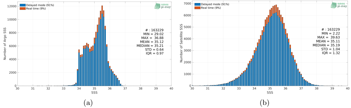
Figure 2: Histograms of SSS from Argo (a) and SMOS SSS L2Q v331 - With FLAG (CMEMS-CATDS-CPDC) (b) considering all match-up pairs per bins of 0.1 over the South Pacific Ocean Pi-MEP region and for the full satellite product period.
