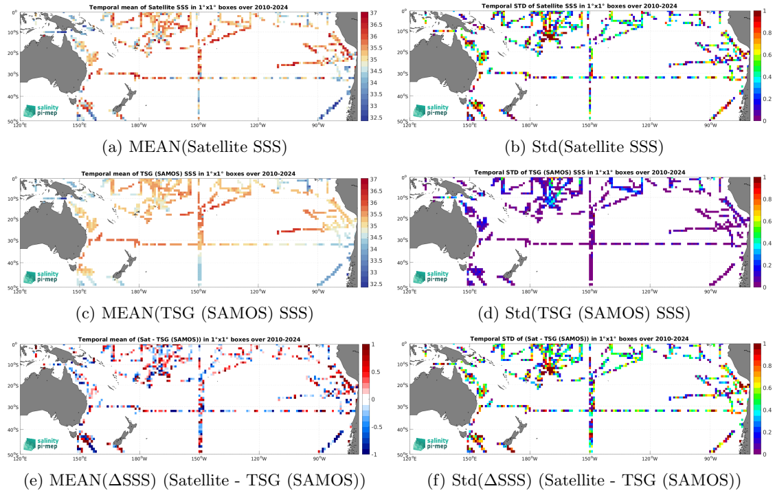
Figure 7: Temporal mean (left) and Std (right) of SSS from SMOS SSS L2Q v331 - No FLAG (CMEMS-CATDS-CPDC) (top), TSG (SAMOS) (middle), and of \Delta SSS (Satellite - TSG (SAMOS)). Only match-up pairs are used to generate these maps.
