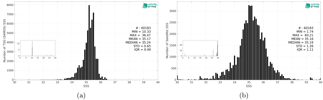
Figure 3: Histograms of SSS from TSG (SAMOS) (a) and SMOS SSS L2Q v331 - No FLAG (CMEMS-CATDS-CPDC) (b) considering all match-up pairs per bins of 0.1 over the South Pacific Ocean Pi-MEP region and for the full satellite product period.
