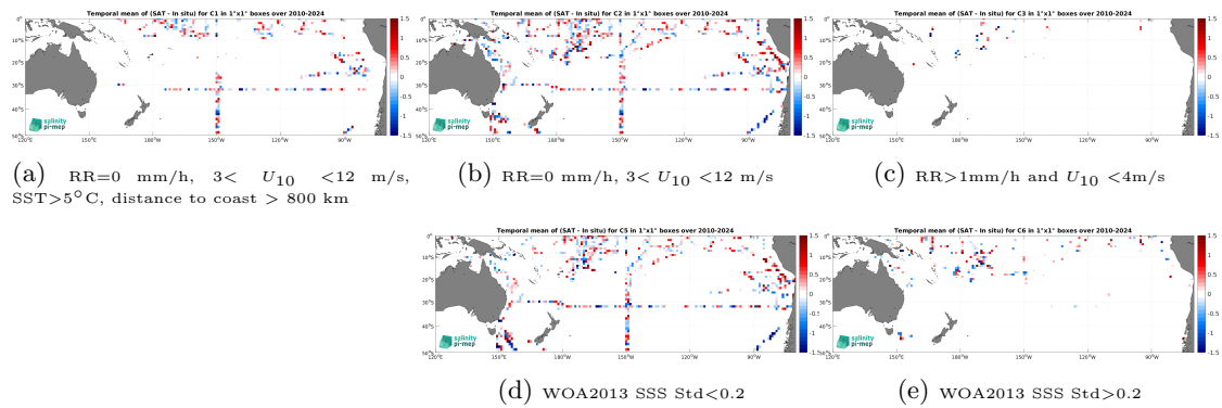
Figure 14: Temporal mean gridded over spatial boxes of size 1^\circ \times 1^\circ of \Delta SSS (SMOS SSS L2Q v331 - No FLAG (CMEMS-CATDS-CPDC) - TSG (SAMOS)) for 5 different subdatasets corresponding to:RR=0 mm/h, 3 < U_{10} < 12 m/s, SST>5°C, distance to coast > 800 km (a), RR=0 mm/h, 3 < U_{10} < 12 m/s (b), RR>1mm/h and U_{10} < 4 m/s (c), WOA2013 SSS Std<0.2 (d), WOA2013 SSS Std>0.2 (e).
