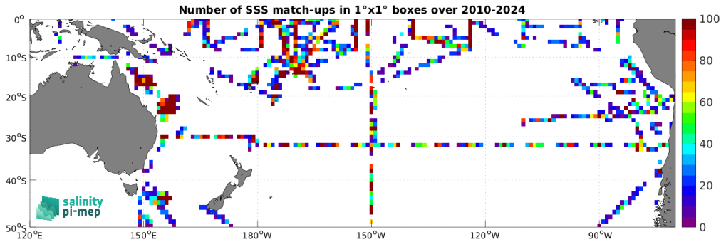
Figure 5: Number of SSS match-ups between TSG (SAMOS) SSS and the SMOS SSS L2Q v331 - No FLAG (CMEMS-CATDS-CPDC) SSS product for the South Pacific Ocean Pi-MEP region over 1^\circ \times 1^\circ boxes and for the full satellite product period.
