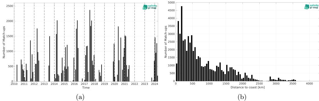
Figure 2: Number of match-ups between TSG (SAMOS) and SMOS SSS L2Q v331 - No FLAG (CMEMS-CATDS-CPDC) SSS as a function of time (a) and as function of the distance to coast (b) over the South Pacific Ocean Pi-MEP region and for the full satellite product period.
