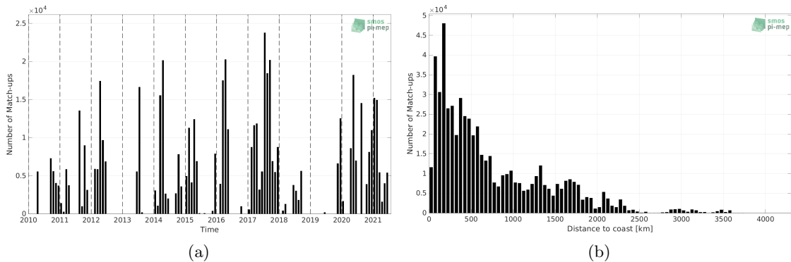
Figure 1: Number of match-ups between TSG (SAMOS) and SMOS SSS L2Q v331 - No FLAG (CMEMS-CATDS-CPDC) SSS as a function of time (a) and as function of the distance to coast (b) over the South Pacific Ocean Pi-MEP region and for the full satellite product period.
