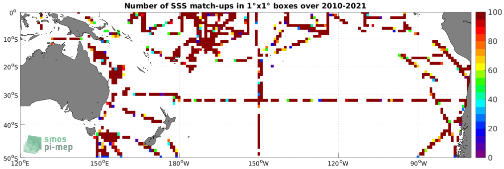
Figure 4: Number of SSS match-ups between TSG (SAMOS) SSS and the SMOS SSS L2Q v331 - No FLAG (CMEMS-CATDS-CPDC) SSS product for the South Pacific Ocean Pi-MEP region over 1^\circ \times 1^\circ boxes and for the full satellite product period.
