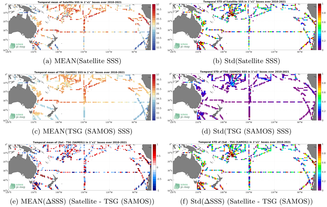
Figure 6: Temporal mean (left) and Std (right) of SSS from SMOS SSS L2Q v331 - No FLAG (CMEMS-CATDS-CPDC) (top), TSG (SAMOS) (middle), and of \Delta SSS (Satellite - TSG (SAMOS)). Only match-up pairs are used to generate these maps.
