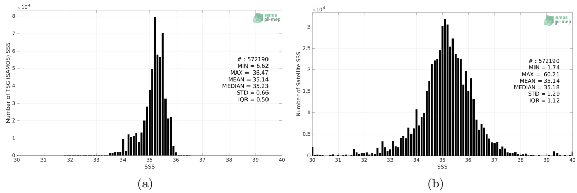
Figure 2: Histograms of SSS from TSG (SAMOS) (a) and SMOS SSS L2Q v331 - No FLAG (CMEMS-CATDS-CPDC) (b) considering all match-up pairs per bins of 0.1 over the South Pacific Ocean Pi-MEP region and for the full satellite product period.
