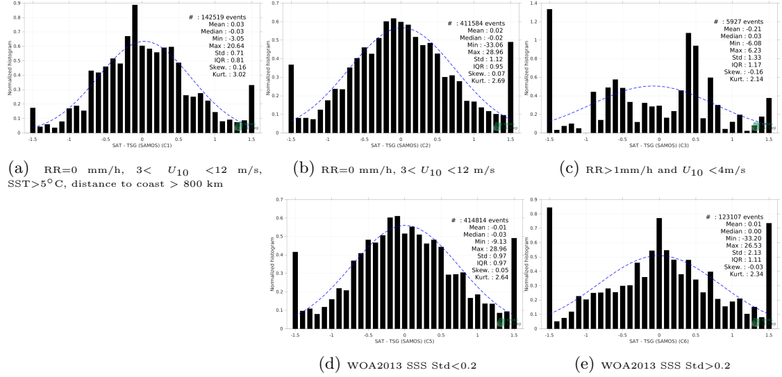
Figure 13: Normalized histogram of \Delta SSS (SMOS SSS L2Q v331 - No FLAG (CMEMS-CATDS-CPDC) - TSG (SAMOS)) for 5 different subdatasets corresponding to: RR=0 mm/h, 3 < U_{10} < 12 m/s, SST >5^{\circ} C, distance to coast > 800 km (a), RR=0 mm/h, 3 < U_{10} < 12 m/s (b), RR >1 mm/h and U_{10} < 4 m/s (c), WOA2013 SSS Std <0.2 (d), WOA2013 SSS Std >0.2 (e).
