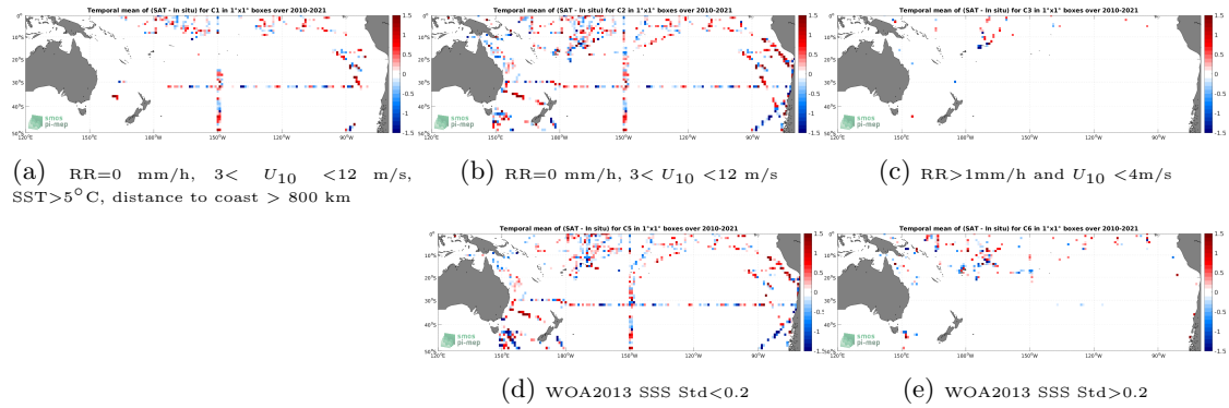
Figure 12: Temporal mean gridded over spatial boxes of size 1^\circ \times 1^\circ of \Delta SSS (SMOS SSS L2Q v331 - No FLAG (CMEMS-CATDS-CPDC) - TSG (SAMOS)) for 5 different subdatasets corresponding to:RR=0 mm/h, 3 < U_{10} < 12 m/s, SST >5^\circ C, distance to coast > 800 km (a), RR=0 mm/h, 3 < U_{10} < 12 m/s (b), RR >1 mm/h and U_{10} < 4 m/s (c), WOA2013 SSS Std <0.2 (d), WOA2013 SSS Std >0.2 (e).
