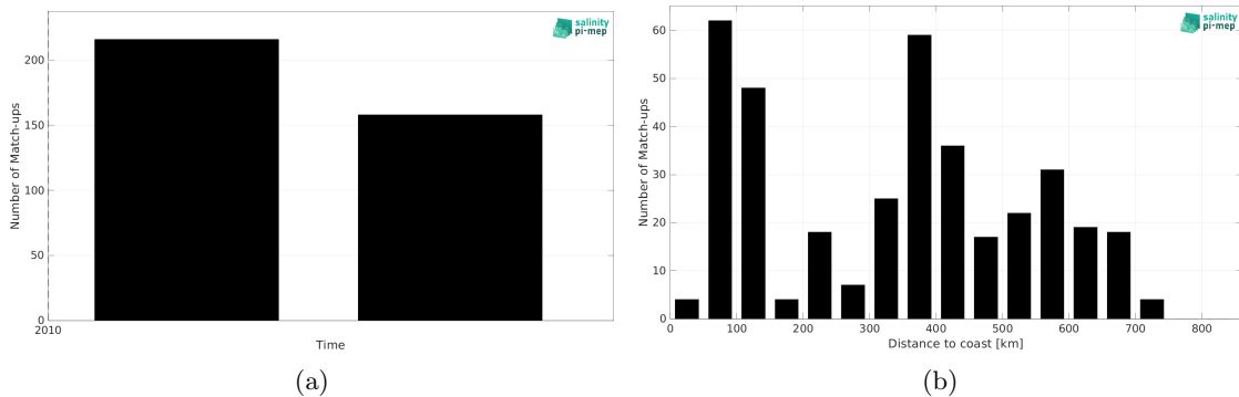
Figure 2: Number of match-ups between TSG (Polarstern) and SMOS SSS L2Q v331 - No FLAG (CMEMS-CATDS-CPDC) SSS as a function of time (a) and as function of the distance to coast (b) over the South Pacific Ocean Pi-MEP region and for the full satellite product period.
