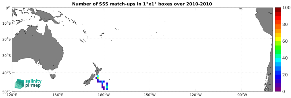
Figure 5: Number of SSS match-ups between TSG (Polarstern) SSS and the SMOS SSS L2Q v331 - No FLAG (CMEMS-CATDS-CPDC) SSS product for the South Pacific Ocean Pi-MEP region over 1^\circ \times 1^\circ boxes and for the full satellite product period.
