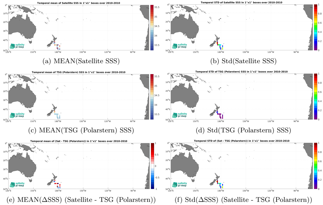
Figure 7: Temporal mean (left) and Std (right) of SSS from SMOS SSS L2Q v331 - No FLAG (CMEMS-CATDS-CPDC) (top), TSG (Polarstern) (middle), and of \Delta SSS (Satellite - TSG (Polarstern)). Only match-up pairs are used to generate these maps.
