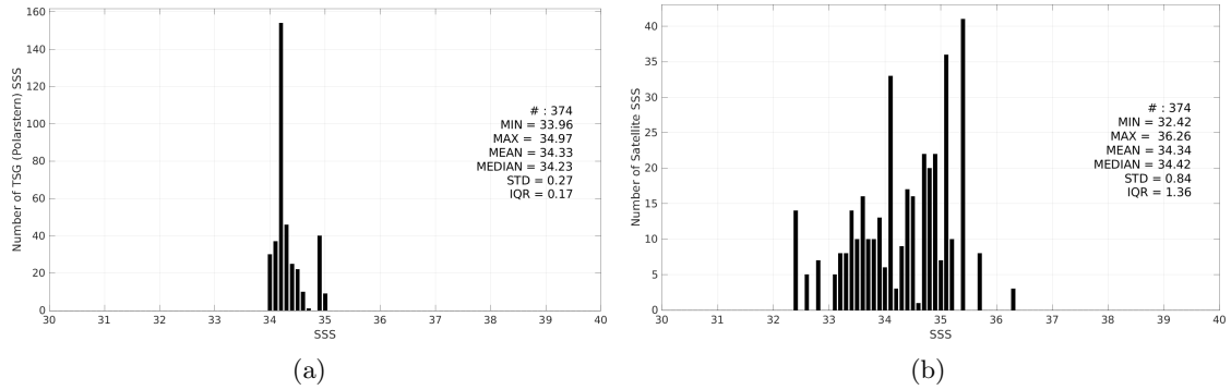
Figure 3: Histograms of SSS from TSG (Polarstern) (a) and SMOS SSS L2Q v331 - No FLAG (CMEMS-CATDS-CPDC) (b) considering all match-up pairs per bins of 0.1 over the South Pacific Ocean Pi-MEP region and for the full satellite product period.
