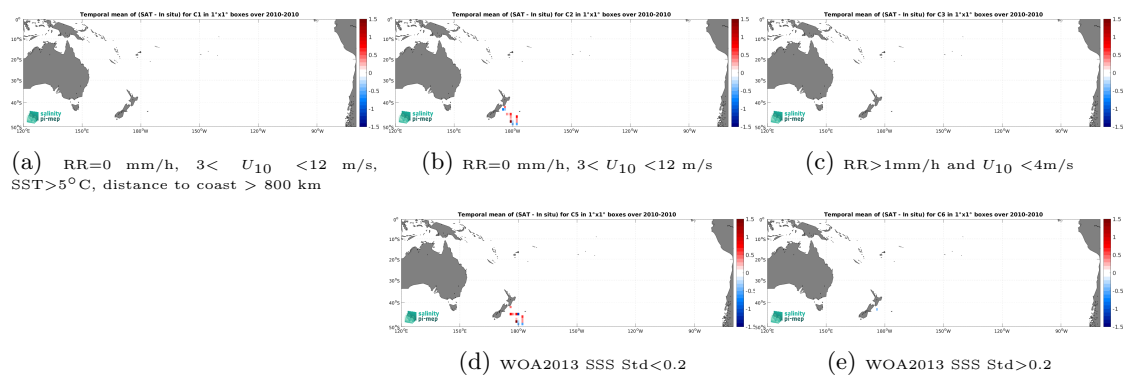
Figure 14: Temporal mean gridded over spatial boxes of size 1^\circ \times 1^\circ of \Delta\text{SSS} (SMOS SSS L2Q v331 - No FLAG (CMEMS-CATDS-CPDC) - TSG (Polarstern)) for 5 different subdatasets corresponding to:RR=0 mm/h, 3 < U_{10} < 12 m/s, SST>5°C, distance to coast > 800 km (a), RR=0 mm/h, 3 < U_{10} < 12 m/s (b), RR>1mm/h and U_{10} < 4 m/s (c), WOA2013 SSS Std<0.2 (d), WOA2013 SSS Std>0.2 (e).
