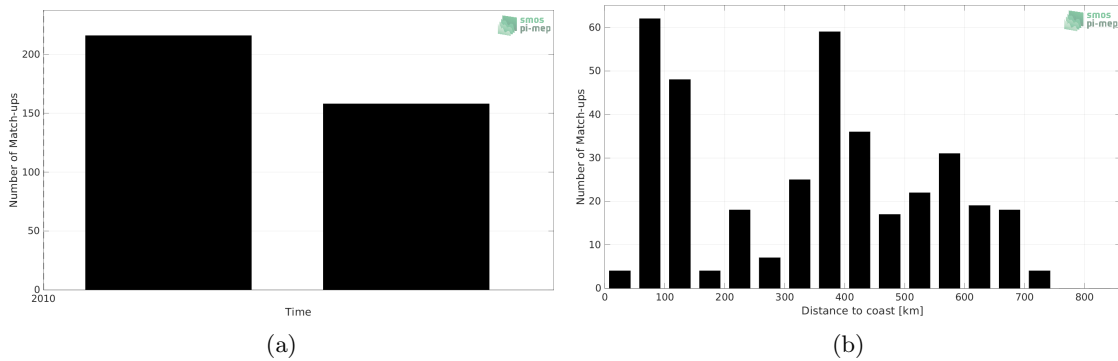
Figure 1: Number of match-ups between TSG (Polarstern) and SMOS SSS L2Q v331 - No FLAG (CMEMS-CATDS-CPDC) SSS as a function of time (a) and as function of the distance to coast (b) over the South Pacific Ocean Pi-MEP region and for the full satellite product period.
