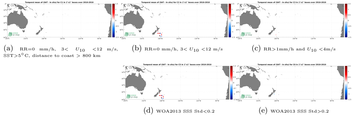
Figure 12: Temporal mean gridded over spatial boxes of size 1^{\circ}\times 1^{\circ} of \Delta\text{SSS} (SMOS SSS L2Q v331 - No FLAG (CMEMS-CATDS-CPDC) - TSG (Polarstern)) for 5 different subdatasets corresponding to:RR=0 mm/h, 3 < U_{10} < 12 m/s, SST >5^{\circ}\text{C} , distance to coast > 800 km (a), RR=0 mm/h, 3 < U_{10} < 12 m/s (b), RR >1 mm/h and U_{10} < 4 m/s (c), WOA2013 SSS Std <0.2 (d), WOA2013 SSS Std >0.2 (e).
