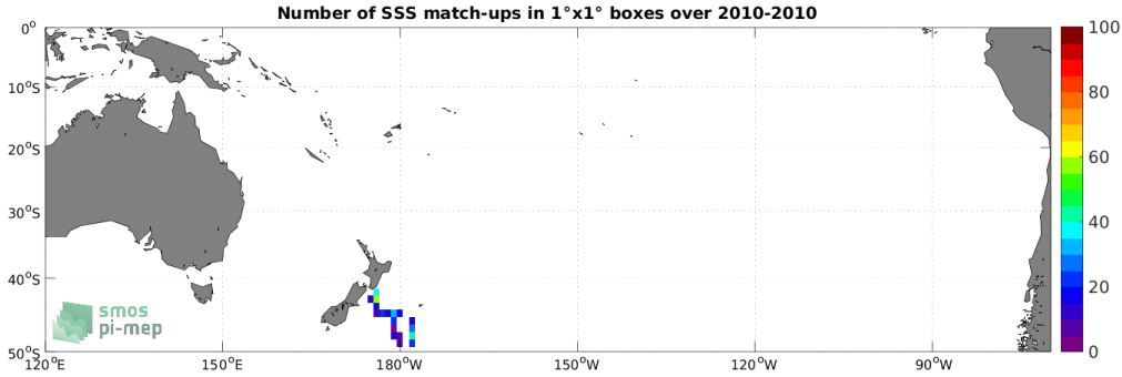
Figure 4: Number of SSS match-ups between TSG (Polarstern) SSS and the SMOS SSS L2Q v331 - No FLAG (CMEMS-CATDS-CPDC) SSS product for the South Pacific Ocean Pi-MEP region over 1^\circ \times 1^\circ boxes and for the full satellite product period.
