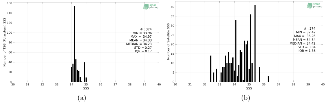
Figure 2: Histograms of SSS from TSG (Polarstern) (a) and SMOS SSS L2Q v331 - No FLAG (CMEMS-CATDS-CPDC) (b) considering all match-up pairs per bins of 0.1 over the South Pacific Ocean Pi-MEP region and for the full satellite product period.
