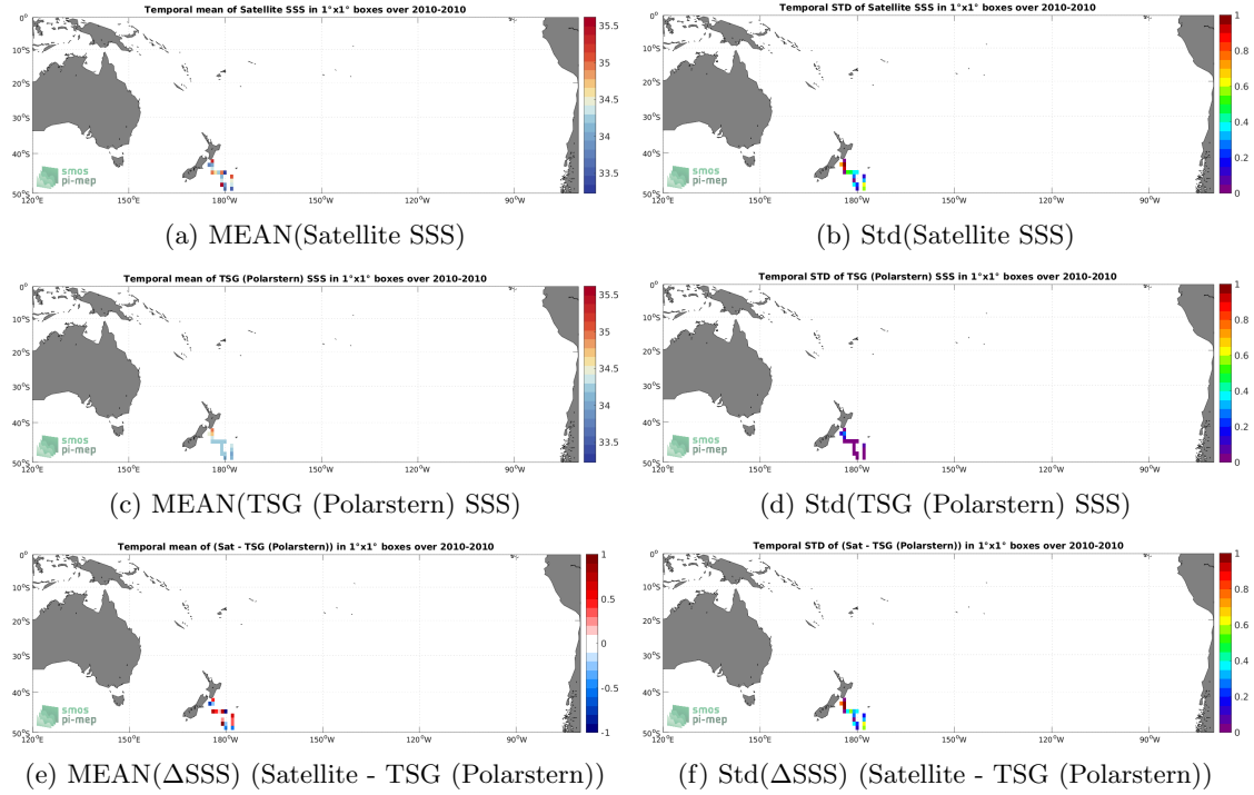
Figure 6: Temporal mean (left) and Std (right) of SSS from SMOS SSS L2Q v331 - No FLAG (CMEMS-CATDS-CPDC) (top), TSG (Polarstern) (middle), and of \Delta SSS (Satellite - TSG (Polarstern)). Only match-up pairs are used to generate these maps.
