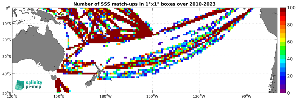
Figure 5: Number of SSS match-ups between TSG (LEGOS-DM) SSS and the SMOS SSS L2Q v331 - No FLAG (CMEMS-CATDS-CPDC) SSS product for the South Pacific Ocean Pi-MEP region over 1^\circ \times 1^\circ boxes and for the full satellite product period.
