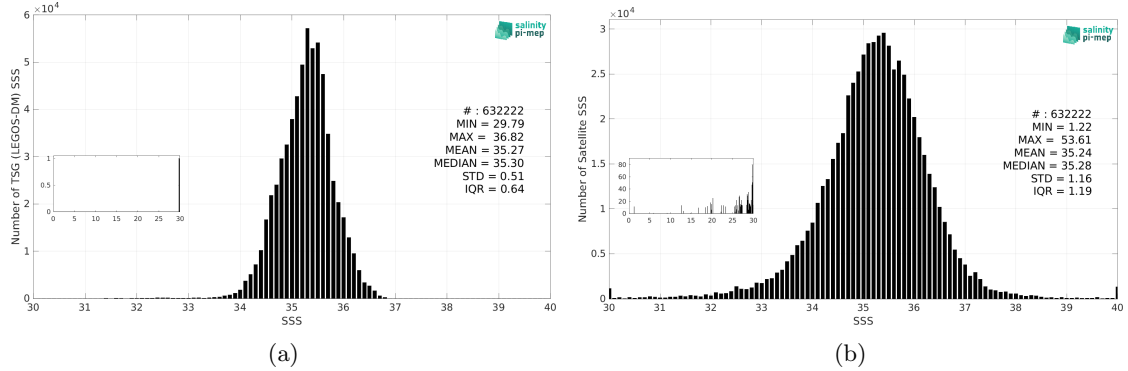
Figure 3: Histograms of SSS from TSG (LEGOS-DM) (a) and SMOS SSS L2Q v331 - No FLAG (CMEMS-CATDS-CPDC) (b) considering all match-up pairs per bins of 0.1 over the South Pacific Ocean Pi-MEP region and for the full satellite product period.
