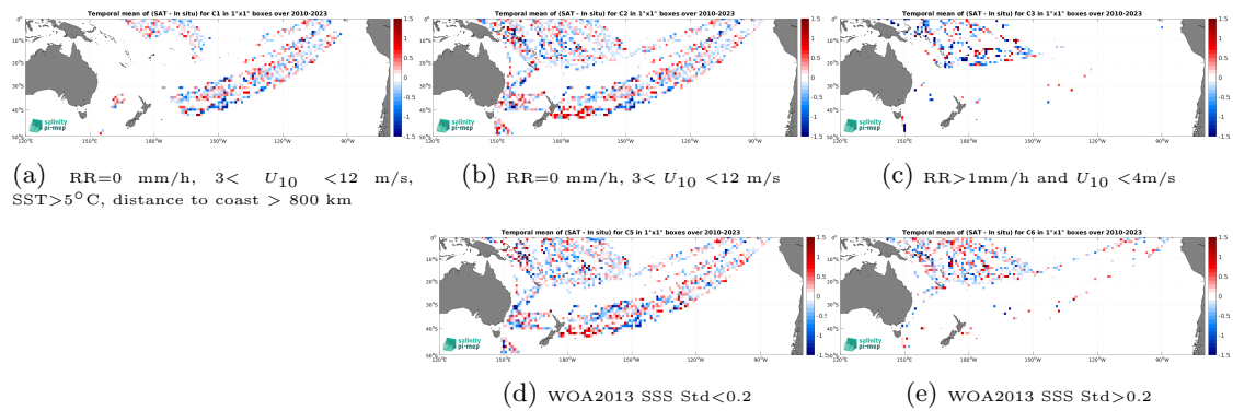
Figure 14: Temporal mean gridded over spatial boxes of size 1^\circ \times 1^\circ of \Delta SSS (SMOS SSS L2Q v331 - No FLAG (CMEMS-CATDS-CPDC) - TSG (LEGOS-DM)) for 5 different subdatasets corresponding to:RR=0 mm/h, 3 < U_{10} < 12 m/s, SST >5^\circ\text{C} , distance to coast > 800 km (a), RR=0 mm/h, 3 < U_{10} < 12 m/s (b), RR >1 mm/h and U_{10} < 4 m/s (c), WOA2013 SSS Std <0.2 (d), WOA2013 SSS Std >0.2 (e).
