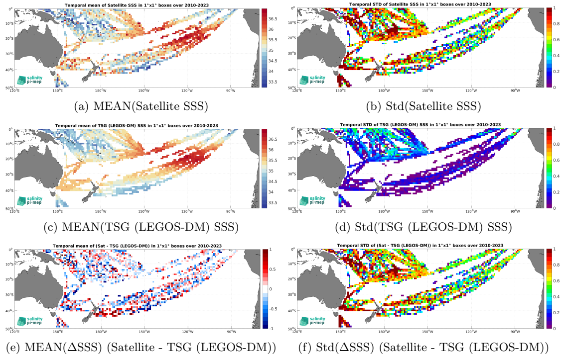
Figure 7: Temporal mean (left) and Std (right) of SSS from SMOS SSS L2Q v331 - No FLAG (CMEMS-CATDS-CPDC) (top), TSG (LEGOS-DM) (middle), and of \Delta SSS (Satellite - TSG (LEGOS-DM)). Only match-up pairs are used to generate these maps.
