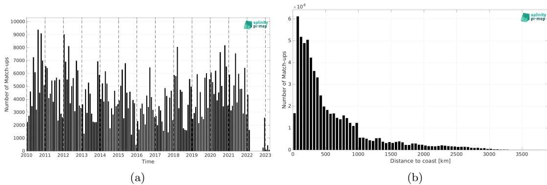
Figure 2: Number of match-ups between TSG (LEGOS-DM) and SMOS SSS L2Q v331 - No FLAG (CMEMS-CATDS-CPDC) SSS as a function of time (a) and as function of the distance to coast (b) over the South Pacific Ocean Pi-MEP region and for the full satellite product period.
