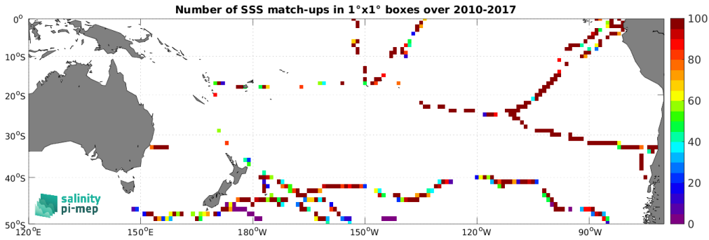
Figure 5: Number of SSS match-ups between TSG (GOSUD-Sailing-ship) SSS and the SMOS SSS L2Q v331 - No FLAG (CMEMS-CATDS-CPDC) SSS product for the South Pacific Ocean Pi-MEP region over 1^\circ \times 1^\circ boxes and for the full satellite product period.
