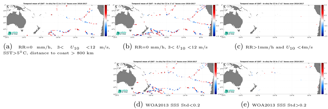
Figure 14: Temporal mean gridded over spatial boxes of size 1^\circ \times 1^\circ of \Delta\text{SSS} (SMOS SSS L2Q v331 - No FLAG (CMEMS-CATDS-CPDC) - TSG (GOSUD-Sailing-ship)) for 5 different sub-datasets corresponding to:RR=0 mm/h, 3 < U_{10} < 12 m/s, SST >5^\circ\text{C} , distance to coast > 800 km (a), RR=0 mm/h, 3 < U_{10} < 12 m/s (b), RR >1 mm/h and U_{10} < 4 m/s (c), WOA2013 SSS Std <0.2 (d), WOA2013 SSS Std >0.2 (e).
