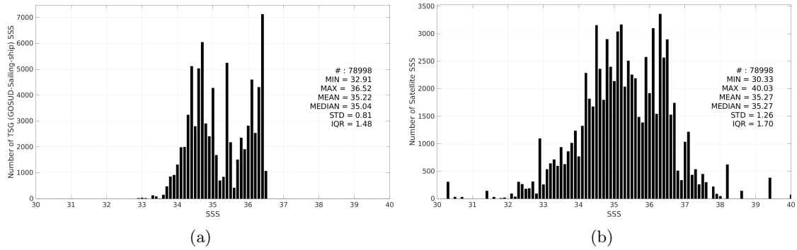
Figure 3: Histograms of SSS from TSG (GOSUD-Sailing-ship) (a) and SMOS SSS L2Q v331 - No FLAG (CMEMS-CATDS-CPDC) (b) considering all match-up pairs per bins of 0.1 over the South Pacific Ocean Pi-MEP region and for the full satellite product period.
