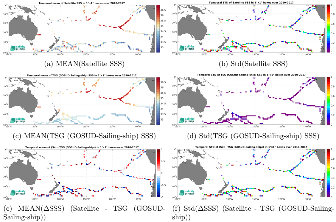
Figure 6: Temporal mean (left) and Std (right) of SSS from SMOS SSS L2Q v331 - No FLAG (CMEMS-CATDS-CPDC) (top), TSG (GOSUD-Sailing-ship) (middle), and of \Delta SSS (Satellite - TSG (GOSUD-Sailing-ship)). Only match-up pairs are used to generate these maps.
