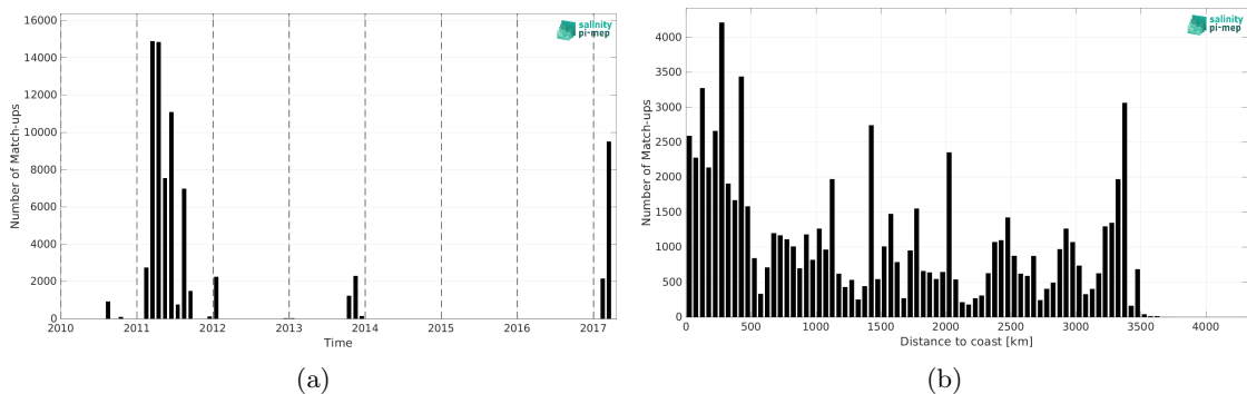
Figure 1: Number of match-ups between TSG (GOSUD-Sailing-ship) and SMOS SSS L2Q v331 - No FLAG (CMEMS-CATDS-CPDC) SSS as a function of time (a) and as function of the distance to coast (b) over the South Pacific Ocean Pi-MEP region and for the full satellite product period.
