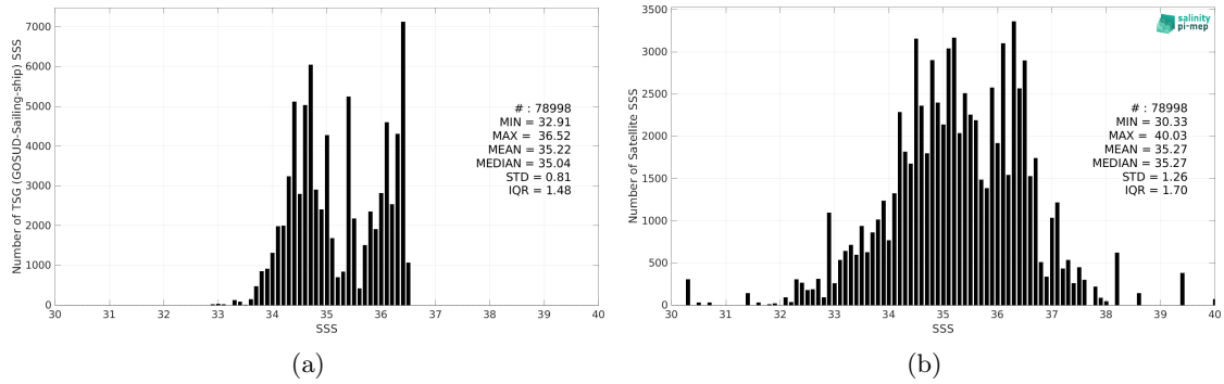
Figure 2: Histograms of SSS from TSG (GOSUD-Sailing-ship) (a) and SMOS SSS L2Q v331 - No FLAG (CMEMS-CATDS-CPDC) (b) considering all match-up pairs per bins of 0.1 over the South Pacific Ocean Pi-MEP region and for the full satellite product period.
