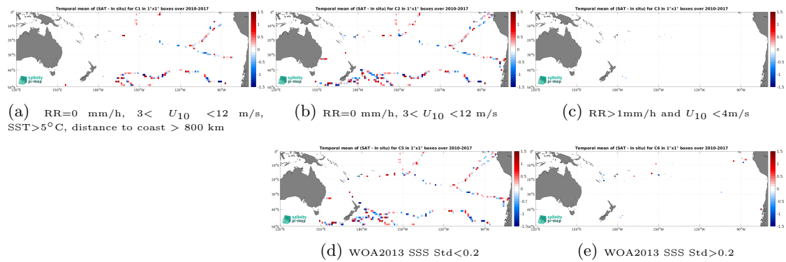
Figure 12: Temporal mean gridded over spatial boxes of size 1^\circ \times 1^\circ of \Delta\text{SSS} (SMOS SSS L2Q v331 - No FLAG (CMEMS-CATDS-CPDC) - TSG (GOSUD-Sailing-ship)) for 5 different sub-datasets corresponding to:RR=0 mm/h, 3 < U_{10} < 12 m/s, SST>5°C, distance to coast > 800 km (a), RR=0 mm/h, 3 < U_{10} < 12 m/s (b), RR>1mm/h and U_{10} < 4 m/s (c), WOA2013 SSS Std<0.2 (d), WOA2013 SSS Std>0.2 (e).
