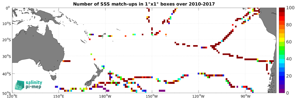
Figure 4: Number of SSS match-ups between TSG (GOSUD-Sailing-ship) SSS and the SMOS SSS L2Q v331 - No FLAG (CMEMS-CATDS-CPDC) SSS product for the South Pacific Ocean Pi-MEP region over 1^\circ \times 1^\circ boxes and for the full satellite product period.
