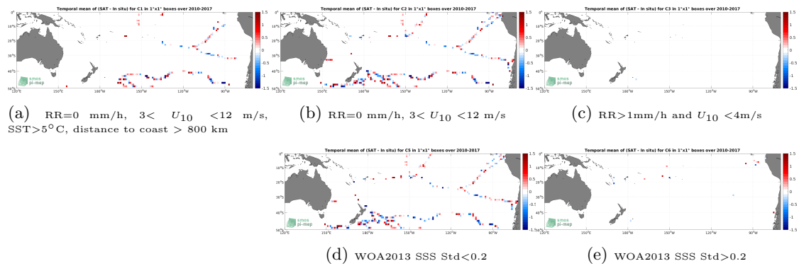
Figure 12: Temporal mean gridded over spatial boxes of size 1^\circ \times 1^\circ of \Delta SSS (SMOS SSS L2Q v331 - No FLAG (CMEMS-CATDS-CPDC) - TSG (GOSUD-Sailing-ship)) for 5 different sub-datasets corresponding to:RR=0 mm/h, 3 < U_{10} < 12 m/s, SST >5^\circ\text{C} , distance to coast > 800 km (a), RR=0 mm/h, 3 < U_{10} < 12 m/s (b), RR >1 mm/h and U_{10} < 4 m/s (c), WOA2013 SSS Std <0.2 (d), WOA2013 SSS Std >0.2 (e).
