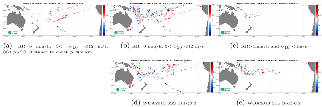
Figure 14: Temporal mean gridded over spatial boxes of size 1^\circ \times 1^\circ of \Delta SSS (SMOS SSS L2Q v331 - No FLAG (CMEMS-CATDS-CPDC) - TSG (GOSUD-Research-vessel)) for 5 different subdatasets corresponding to:RR=0 mm/h, 3 < U_{10} < 12 m/s, SST >5^\circ C, distance to coast > 800 km (a), RR=0 mm/h, 3 < U_{10} < 12 m/s (b), RR >1 mm/h and U_{10} < 4 m/s (c), WOA2013 SSS Std <0.2 (d), WOA2013 SSS Std >0.2 (e).
