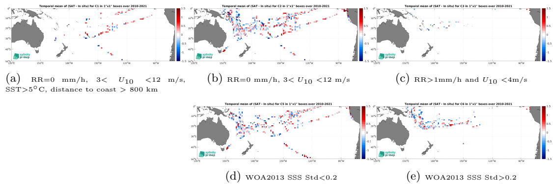
Figure 12: Temporal mean gridded over spatial boxes of size 1^\circ \times 1^\circ of \Delta\text{SSS} (SMOS SSS L2Q v331 - No FLAG (CMEMS-CATDS-CPDC) - TSG (GOSUD-Research-vessel)) for 5 different subdatasets corresponding to:RR=0 mm/h, 3 < U_{10} < 12 m/s, SST>5°C, distance to coast > 800 km (a), RR=0 mm/h, 3 < U_{10} < 12 m/s (b), RR>1mm/h and U_{10} < 4 m/s (c), WOA2013 SSS Std<0.2 (d), WOA2013 SSS Std>0.2 (e).
