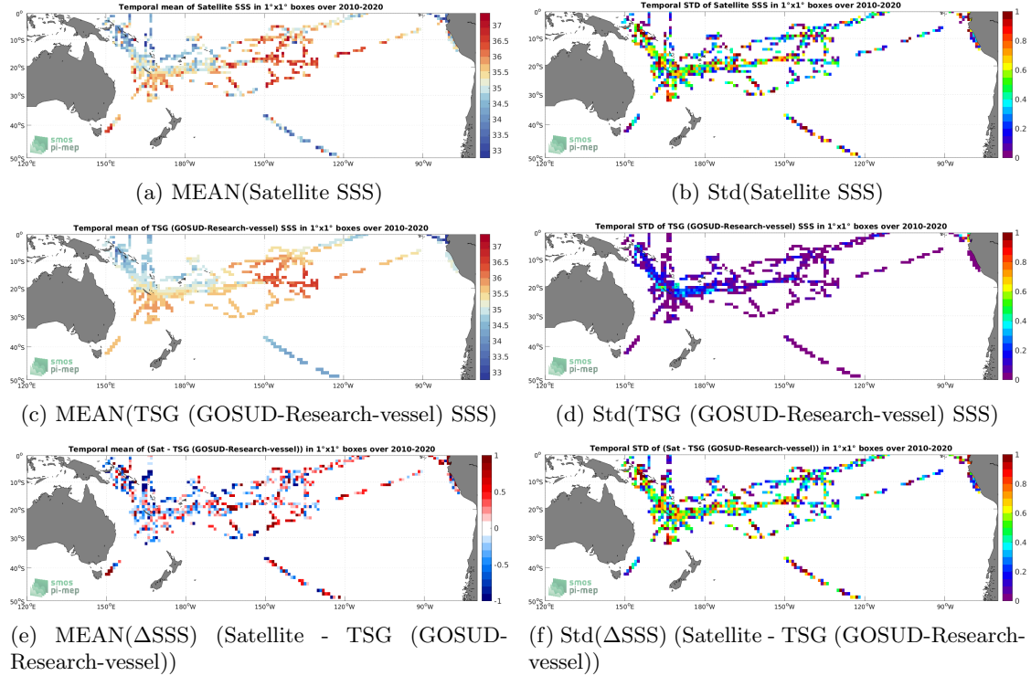
Figure 6: Temporal mean (left) and Std (right) of SSS from SMOS SSS L2Q v331 - No FLAG (CMEMS-CATDS-CPDC) (top), TSG (GOSUD-Research-vessel) (middle), and of \Delta SSS (Satellite - TSG (GOSUD-Research-vessel)). Only match-up pairs are used to generate these maps.
