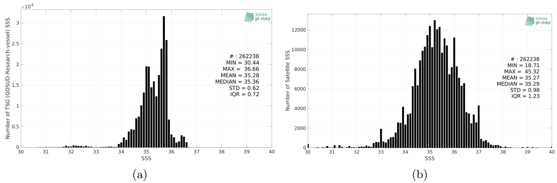
Figure 2: Histograms of SSS from TSG (GOSUD-Research-vessel) (a) and SMOS SSS L2Q v331 - No FLAG (CMEMS-CATDS-CPDC) (b) considering all match-up pairs per bins of 0.1 over the South Pacific Ocean Pi-MEP region and for the full satellite product period.
