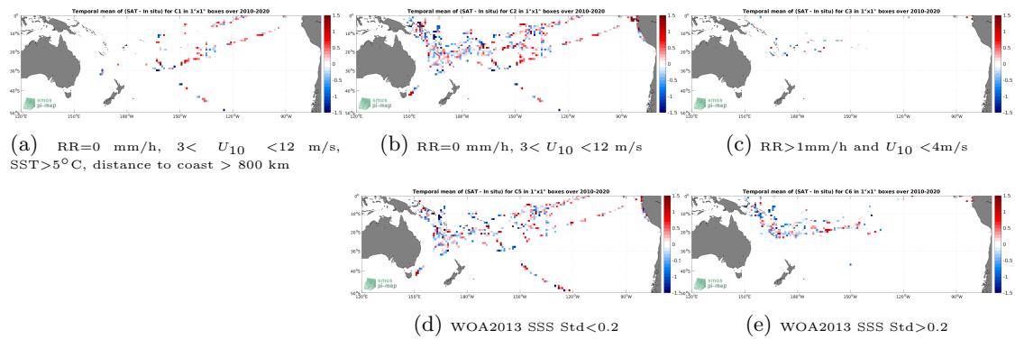
Figure 12: Temporal mean gridded over spatial boxes of size 1^\circ \times 1^\circ of \Delta SSS (SMOS SSS L2Q v331 - No FLAG (CMEMS-CATDS-CPDC) - TSG (GOSUD-Research-vessel)) for 5 different subdatasets corresponding to:RR=0 mm/h, 3 < U_{10} < 12 m/s, SST >5^\circ C, distance to coast > 800 km (a), RR=0 mm/h, 3 < U_{10} < 12 m/s (b), RR >1 mm/h and U_{10} < 4 m/s (c), WOA2013 SSS Std <0.2 (d), WOA2013 SSS Std >0.2 (e).
