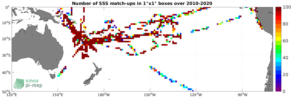
Figure 4: Number of SSS match-ups between TSG (GOSUD-Research-vessel) SSS and the SMOS SSS L2Q v331 - No FLAG (CMEMS-CATDS-CPDC) SSS product for the South Pacific Ocean Pi-MEP region over 1^\circ \times 1^\circ boxes and for the full satellite product period.
