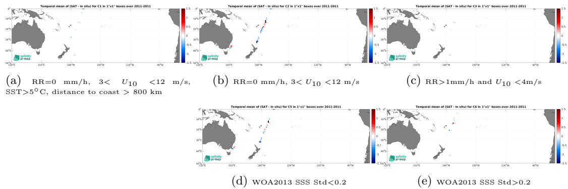
Figure 14: Temporal mean gridded over spatial boxes of size 1^\circ \times 1^\circ of \Delta SSS (SMOS SSS L2Q v331 - No FLAG (CMEMS-CATDS-CPDC) - TSG (CSIC-UTM)) for 5 different subdatasets corresponding to:RR=0 mm/h, 3 < U_{10} < 12 m/s, SST >5^\circ C, distance to coast > 800 km (a), RR=0 mm/h, 3 < U_{10} < 12 m/s (b), RR >1 mm/h and U_{10} < 4 m/s (c), WOA2013 SSS Std <0.2 (d), WOA2013 SSS Std >0.2 (e).
