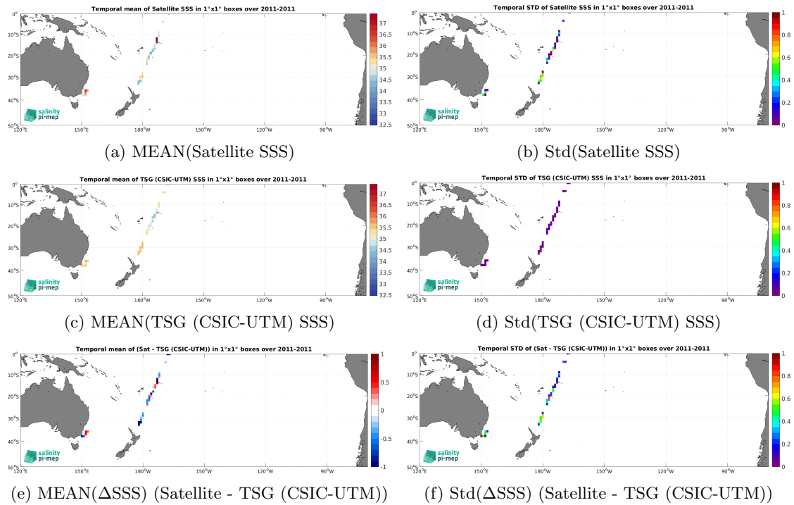
Figure 7: Temporal mean (left) and Std (right) of SSS from SMOS SSS L2Q v331 - No FLAG (CMEMS-CATDS-CPDC) (top), TSG (CSIC-UTM) (middle), and of \Delta SSS (Satellite - TSG (CSIC-UTM)). Only match-up pairs are used to generate these maps.
