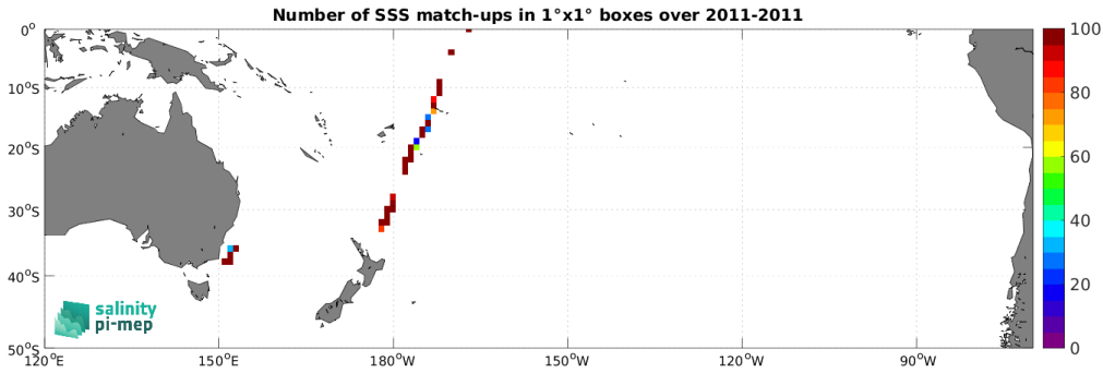
Figure 5: Number of SSS match-ups between TSG (CSIC-UTM) SSS and the SMOS SSS L2Q v331 - No FLAG (CMEMS-CATDS-CPDC) SSS product for the South Pacific Ocean Pi-MEP region over 1^\circ \times 1^\circ boxes and for the full satellite product period.
