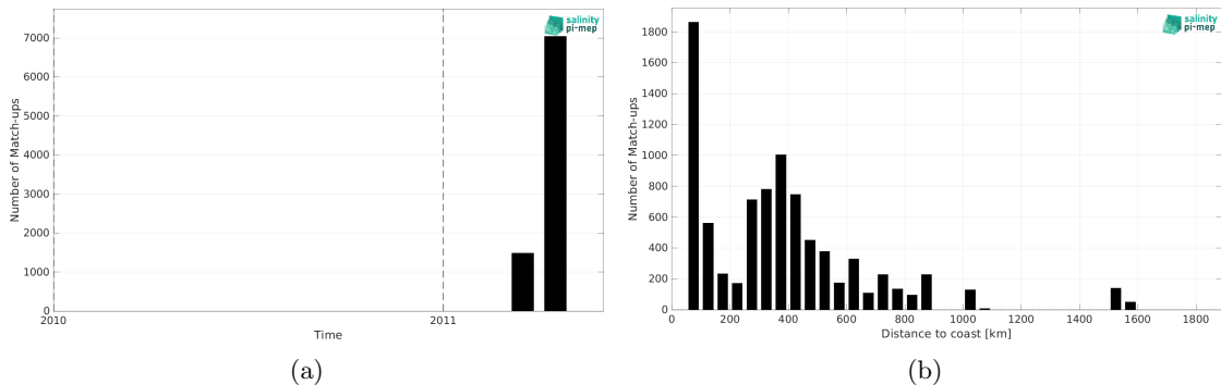
Figure 2: Number of match-ups between TSG (CSIC-UTM) and SMOS SSS L2Q v331 - No FLAG (CMEMS-CATDS-CPDC) SSS as a function of time (a) and as function of the distance to coast (b) over the South Pacific Ocean Pi-MEP region and for the full satellite product period.
