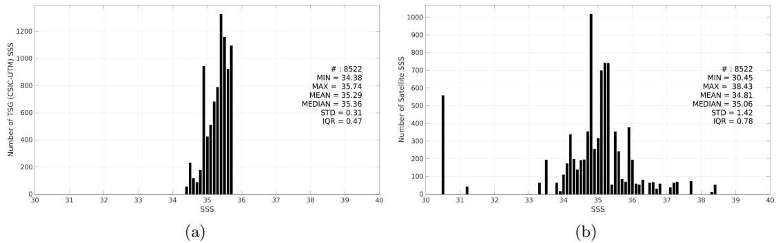
Figure 3: Histograms of SSS from TSG (CSIC-UTM) (a) and SMOS SSS L2Q v331 - No FLAG (CMEMS-CATDS-CPDC) (b) considering all match-up pairs per bins of 0.1 over the South Pacific Ocean Pi-MEP region and for the full satellite product period.
