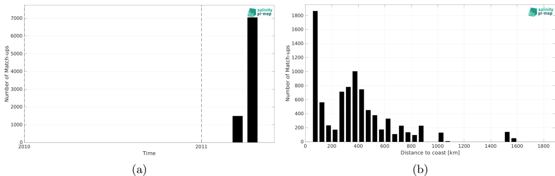
Figure 1: Number of match-ups between TSG (CSIC-UTM) and SMOS SSS L2Q v331 - No FLAG (CMEMS-CATDS-CPDC) SSS as a function of time (a) and as function of the distance to coast (b) over the South Pacific Ocean Pi-MEP region and for the full satellite product period.
