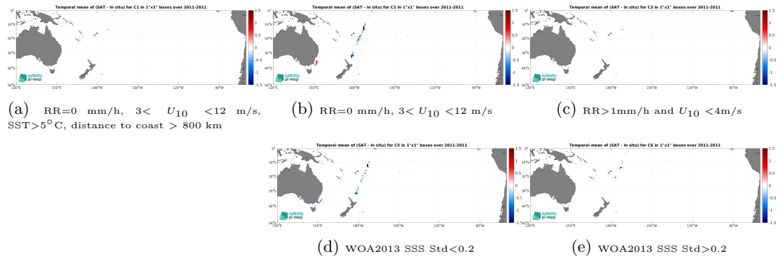
Figure 12: Temporal mean gridded over spatial boxes of size 1^{\circ}\times 1^{\circ} of \Delta\text{SSS} (SMOS SSS L2Q v331 - No FLAG (CMEMS-CATDS-CPDC) - TSG (CSIC-UTM)) for 5 different subdatasets corresponding to:RR=0 mm/h, 3 < U_{10} < 12 m/s, SST > 5^{\circ}\text{C} , distance to coast > 800 km (a), RR=0 mm/h, 3 < U_{10} < 12 m/s (b), RR > 1 mm/h and U_{10} < 4 m/s (c), WOA2013 SSS Std < 0.2 (d), WOA2013 SSS Std > 0.2 (e).
