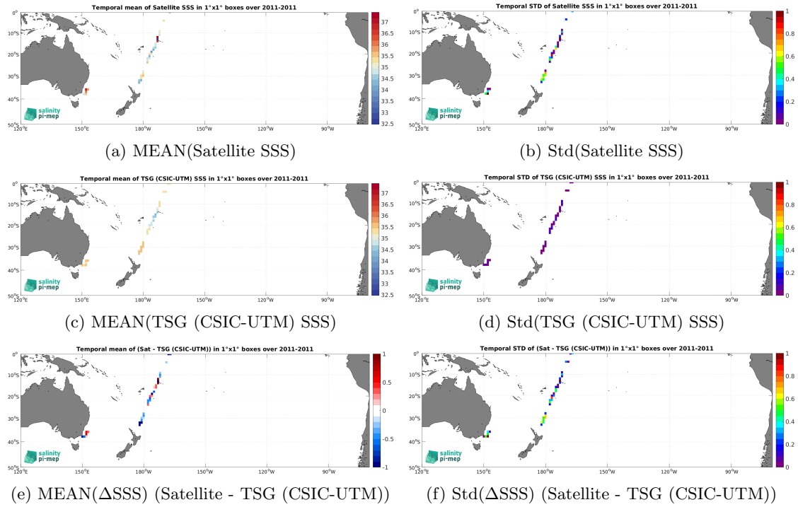
Figure 6: Temporal mean (left) and Std (right) of SSS from SMOS SSS L2Q v331 - No FLAG (CMEMS-CATDS-CPDC) (top), TSG (CSIC-UTM) (middle), and of \Delta SSS (Satellite - TSG (CSIC-UTM)). Only match-up pairs are used to generate these maps.
