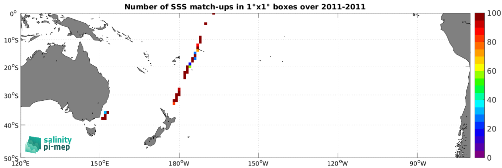
Figure 4: Number of SSS match-ups between TSG (CSIC-UTM) SSS and the SMOS SSS L2Q v331 - No FLAG (CMEMS-CATDS-CPDC) SSS product for the South Pacific Ocean Pi-MEP region over 1^\circ \times 1^\circ boxes and for the full satellite product period.
