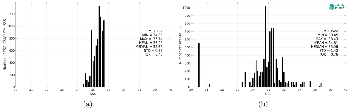
Figure 2: Histograms of SSS from TSG (CSIC-UTM) (a) and SMOS SSS L2Q v331 - No FLAG (CMEMS-CATDS-CPDC) (b) considering all match-up pairs per bins of 0.1 over the South Pacific Ocean Pi-MEP region and for the full satellite product period.
