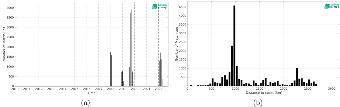
Figure 2: Number of match-ups between Saildrone and SMOS SSS L2Q v331 - No FLAG (CMEMS-CATDS-CPDC) SSS as a function of time (a) and as function of the distance to coast (b) over the South Pacific Ocean Pi-MEP region and for the full satellite product period.
