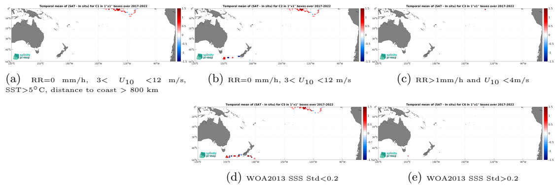
Figure 14: Temporal mean gridded over spatial boxes of size 1^\circ \times 1^\circ of \Delta SSS (SMOS SSS L2Q v331 - No FLAG (CMEMS-CATDS-CPDC) - Saildrone) for 5 different subdatasets corresponding to:RR=0 mm/h, 3 < U_{10} < 12 m/s, SST>5°C, distance to coast > 800 km (a), RR=0 mm/h, 3 < U_{10} < 12 m/s (b), RR>1mm/h and U_{10} < 4 m/s (c), WOA2013 SSS Std<0.2 (d), WOA2013 SSS Std>0.2 (e).
