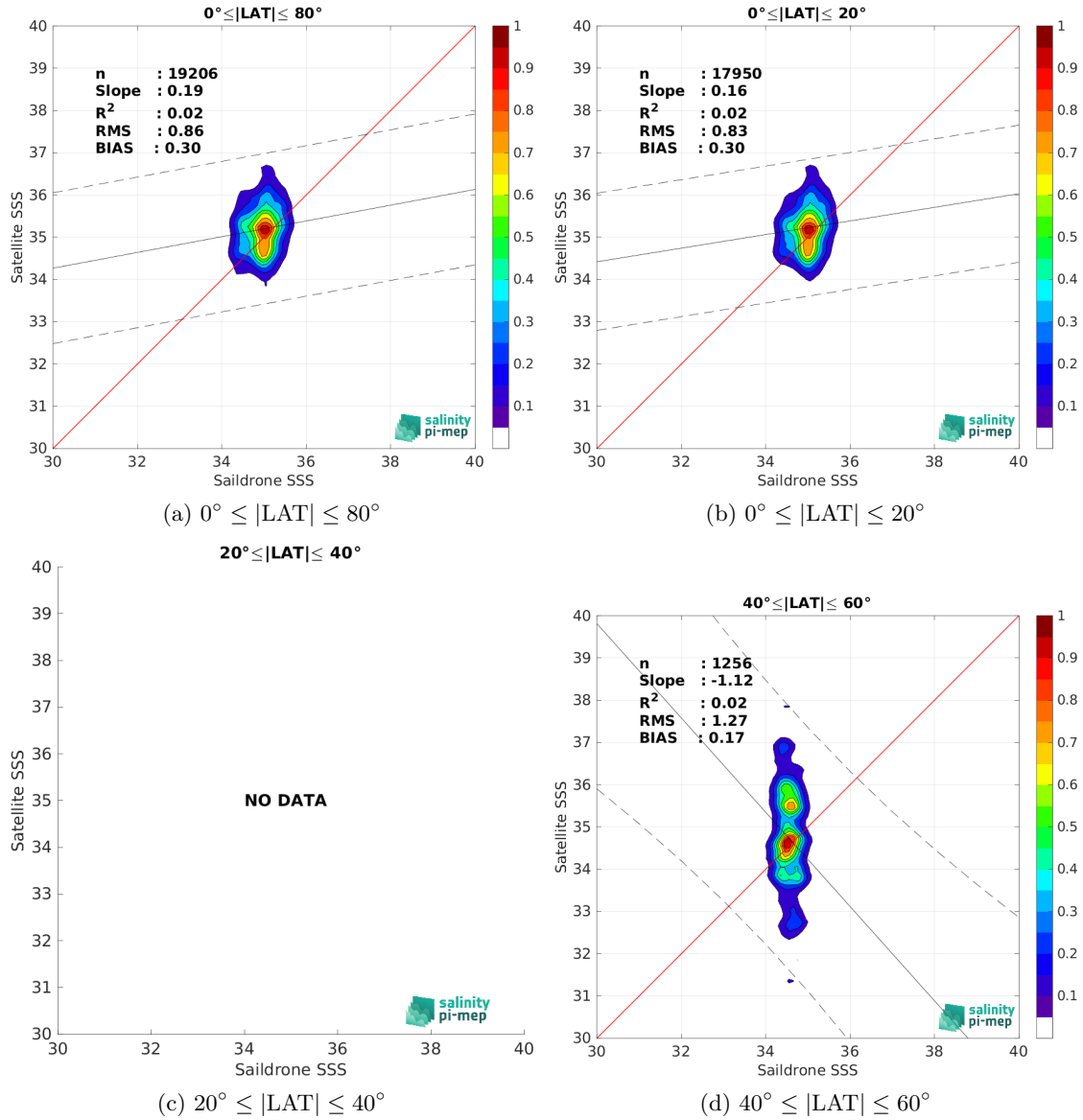
Figure 10: Contour maps of the concentration of SMOS SSS L2Q v331 - No FLAG (CMEMS-CATDS-CPDC) SSS (y-axis) versus Sailability SSS (x-axis) at match-up pairs for different latitude bands. For each plot, the red line shows x=y . The black thin and dashed lines indicate a linear fit through the data cloud and the \pm 95\% confidence levels, respectively. The number match-up pairs n , the slope and R^2 coefficient of the linear fit, the root mean square (RMS) and the mean bias between satellite and in situ data are indicated for each latitude band in each plots.
