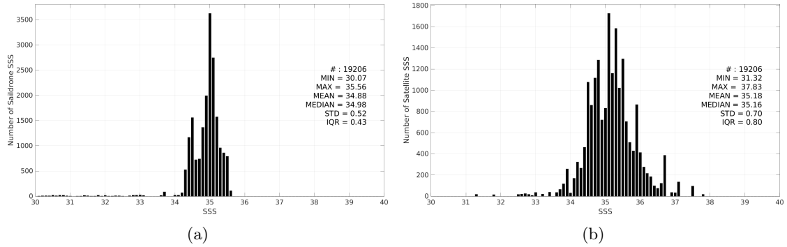
Figure 3: Histograms of SSS from Saildrone (a) and SMOS SSS L2Q v331 - No FLAG (CMEMS-CATDS-CPDC) (b) considering all match-up pairs per bins of 0.1 over the South Pacific Ocean Pi-MEP region and for the full satellite product period.
