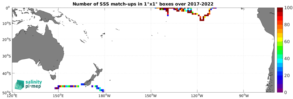
Figure 4: Number of SSS match-ups between Saildrone SSS and the SMOS SSS L2Q v331 - No FLAG (CMEMS-CATDS-CPDC) SSS product for the South Pacific Ocean Pi-MEP region over 1^\circ \times 1^\circ boxes and for the full satellite product period.
