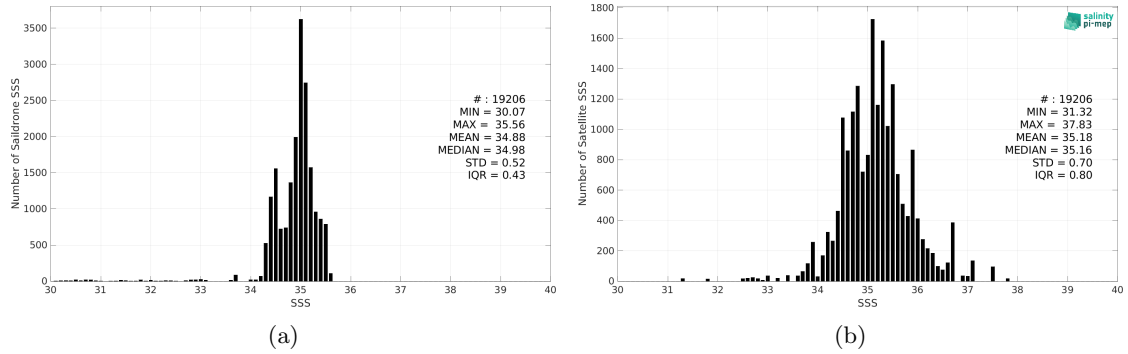
Figure 2: Histograms of SSS from Saildrone (a) and SMOS SSS L2Q v331 - No FLAG (CMEMS-CATDS-CPDC) (b) considering all match-up pairs per bins of 0.1 over the South Pacific Ocean Pi-MEP region and for the full satellite product period.
