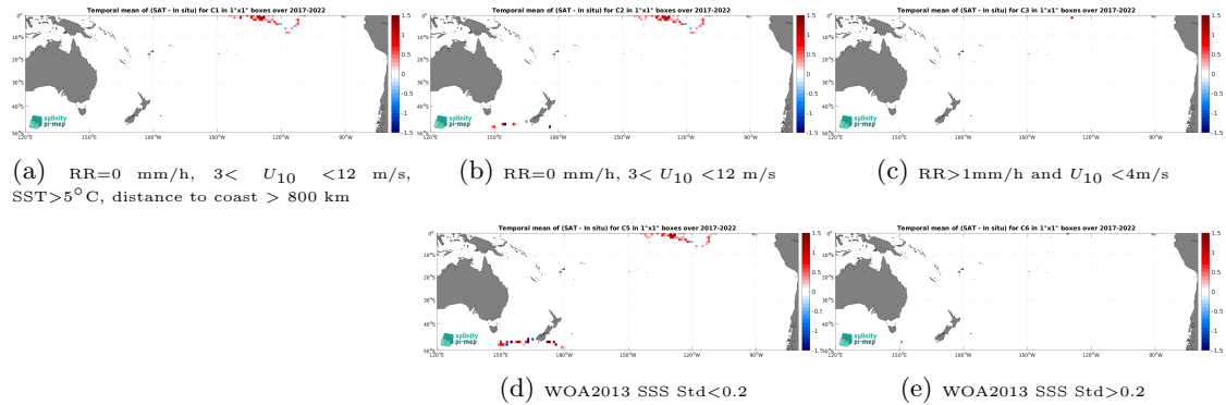
Figure 12: Temporal mean gridded over spatial boxes of size 1^\circ \times 1^\circ of \Delta SSS (SMOS SSS L2Q v331 - No FLAG (CMEMS-CATDS-CPDC) - Saildrone) for 5 different subdatasets corresponding to:RR=0 mm/h, 3 < U_{10} < 12 m/s, SST >5^\circ\text{C} , distance to coast > 800 km (a), RR=0 mm/h, 3 < U_{10} < 12 m/s (b), RR >1 mm/h and U_{10} < 4 m/s (c), WOA2013 SSS Std <0.2 (d), WOA2013 SSS Std >0.2 (e).
