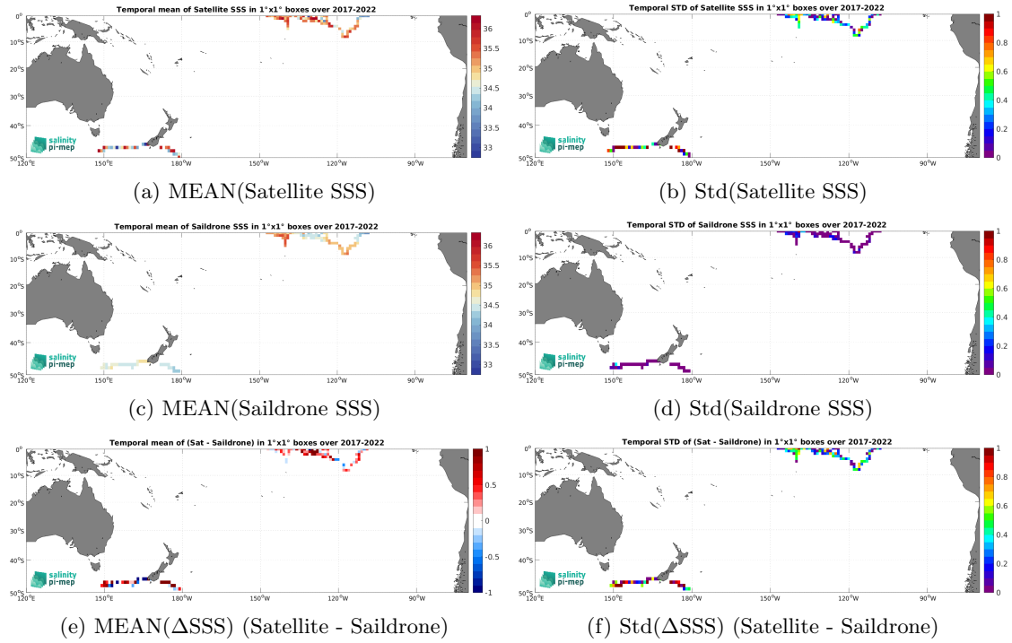
Figure 6: Temporal mean (left) and Std (right) of SSS from SMOS SSS L2Q v331 - No FLAG (CMEMS-CATDS-CPDC) (top), Saildrone (middle), and of \Delta SSS (Satellite - Saildrone). Only match-up pairs are used to generate these maps.
