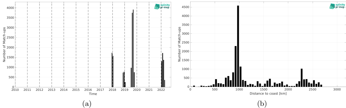
Figure 1: Number of match-ups between Saildrone and SMOS SSS L2Q v331 - No FLAG (CMEMS-CATDS-CPDC) SSS as a function of time (a) and as function of the distance to coast (b) over the South Pacific Ocean Pi-MEP region and for the full satellite product period.
