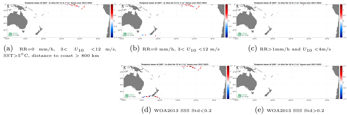
Figure 12: Temporal mean gridded over spatial boxes of size 1^\circ \times 1^\circ of \Delta SSS (SMOS SSS L2Q v331 - No FLAG (CMEMS-CATDS-CPDC) - Sairdrone) for 5 different subdatasets corresponding to:RR=0 mm/h, 3 < U_{10} < 12 m/s, SST >5^\circ C, distance to coast > 800 km (a), RR=0 mm/h, 3 < U_{10} < 12 m/s (b), RR >1 mm/h and U_{10} < 4 m/s (c), WOA2013 SSS Std <0.2 (d), WOA2013 SSS Std >0.2 (e).
