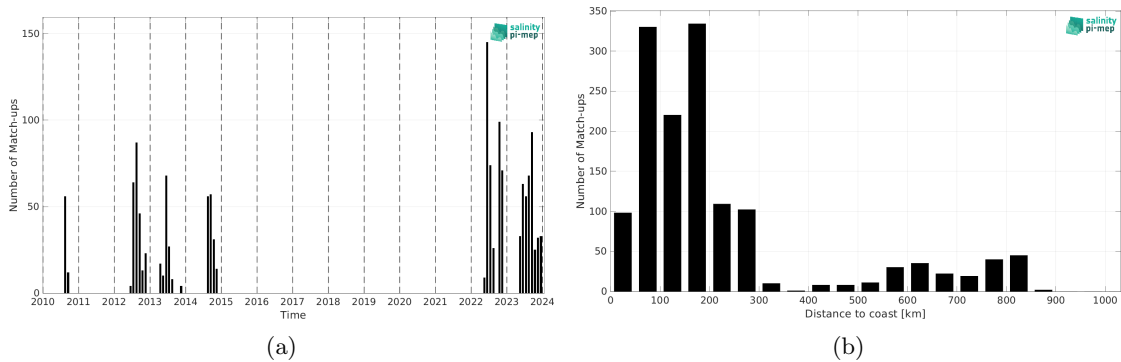
Figure 2: Number of match-ups between Marine mammals and SMOS SSS L2Q v331 - No FLAG (CMEMS-CATDS-CPDC) SSS as a function of time (a) and as function of the distance to coast (b) over the South Pacific Ocean Pi-MEP region and for the full satellite product period.
