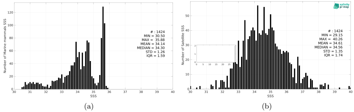
Figure 3: Histograms of SSS from Marine mammals (a) and SMOS SSS L2Q v331 - No FLAG (CMEMS-CATDS-CPDC) (b) considering all match-up pairs per bins of 0.1 over the South Pacific Ocean Pi-MEP region and for the full satellite product period.
