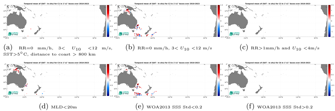
Figure 14: Temporal mean gridded over spatial boxes of size 1^\circ \times 1^\circ of \Delta SSS (SMOS SSS L2Q v331 - No FLAG (CMEMS-CATDS-CPDC) - Marine mammals) for 6 different subdatasets corresponding to:RR=0 mm/h, 3 < U_{10} < 12 m/s, SST>5°C, distance to coast > 800 km (a), RR=0 mm/h, 3 < U_{10} < 12 m/s (b), RR>1mm/h and U_{10} < 4 m/s (c),MLD<20m (d),WOA2013 SSS Std<0.2 (e),WOA2013 SSS Std>0.2 (f).
