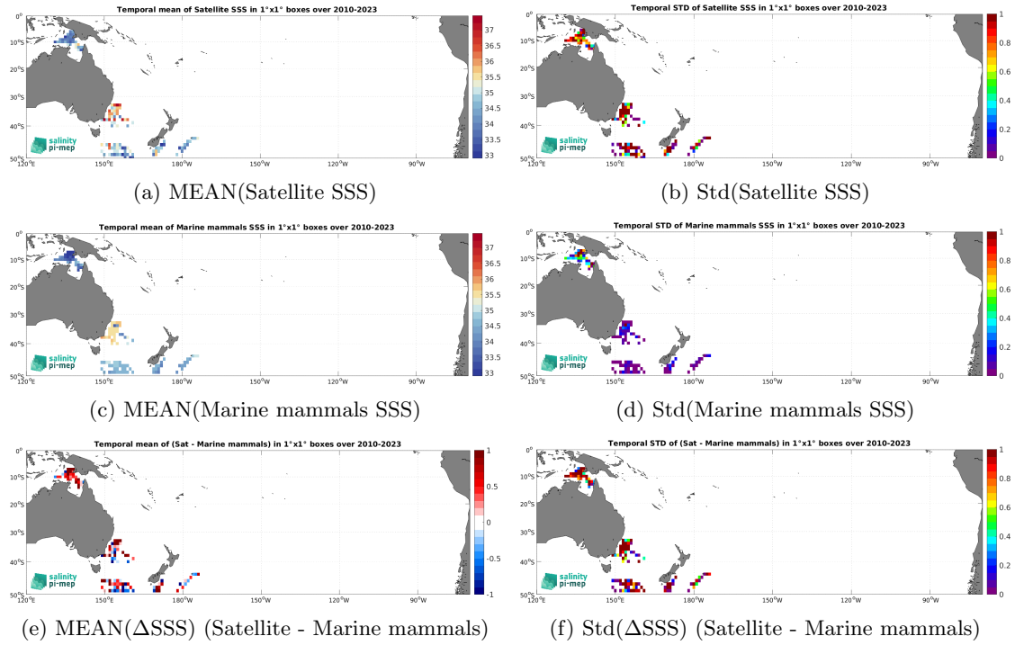
Figure 7: Temporal mean (left) and Std (right) of SSS from SMOS SSS L2Q v331 - No FLAG (CMEMS-CATDS-CPDC) (top), Marine mammals (middle), and of \Delta SSS (Satellite - Marine mammals). Only match-up pairs are used to generate these maps.
