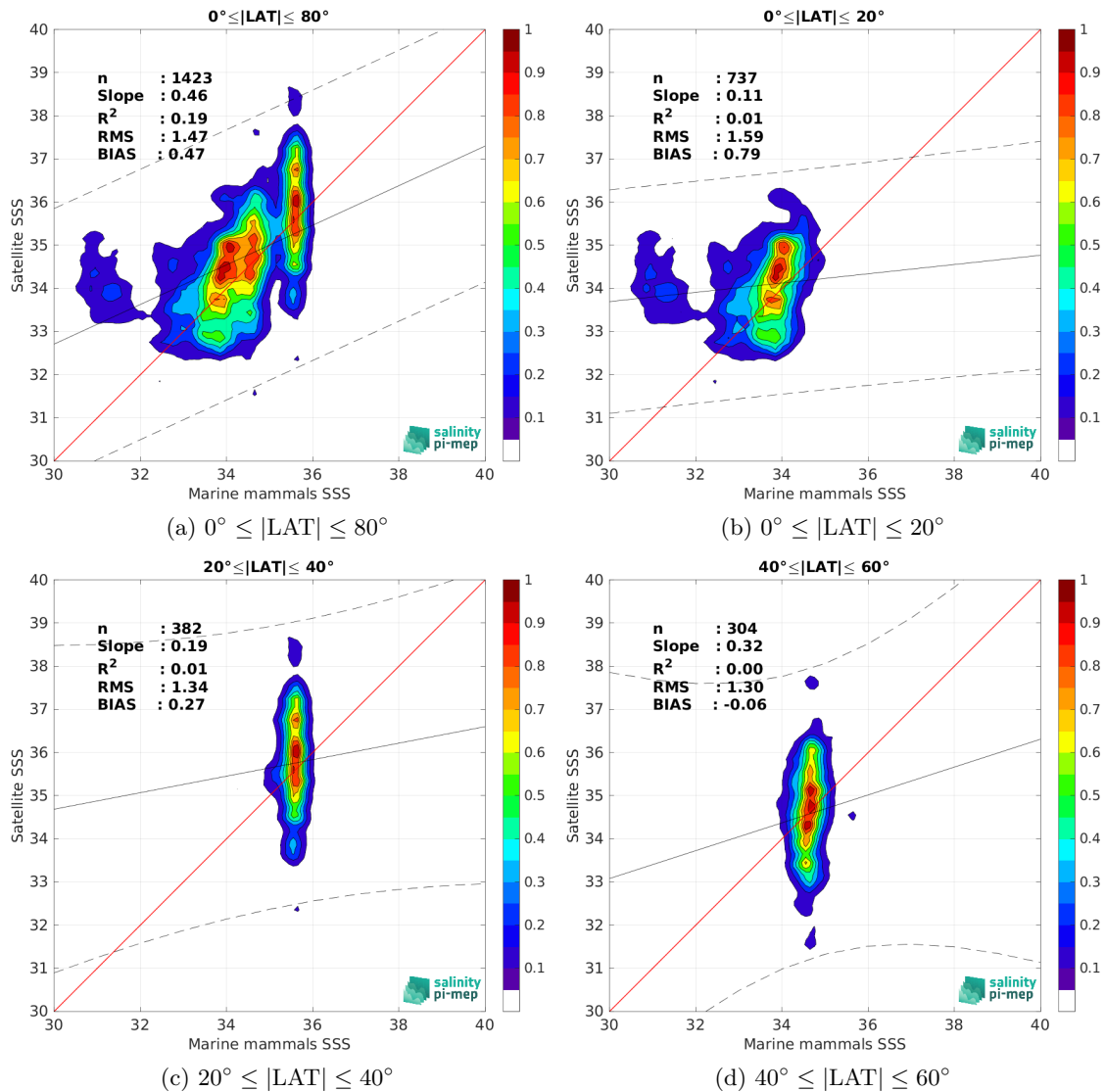
Figure 10: Contour maps of the concentration of SMOS SSS L2Q v331 - No FLAG (CMEMS-CATDS-CPDC) SSS (y-axis) versus Marine mammals SSS (x-axis) at match-up pairs for different latitude bands. For each plot, the red line shows x=y . The black thin and dashed lines indicate a linear fit through the data cloud and the \pm 95\% confidence levels, respectively. The number match-up pairs n , the slope and R^2 coefficient of the linear fit, the root mean square (RMS) and the mean bias between satellite and in situ data are indicated for each latitude band in each plots.
