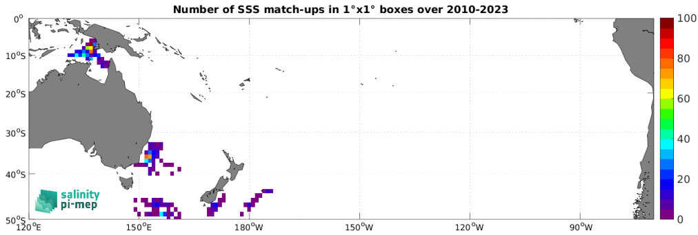
Figure 5: Number of SSS match-ups between Marine mammals SSS and the SMOS SSS L2Q v331 - No FLAG (CMEMS-CATDS-CPDC) SSS product for the South Pacific Ocean Pi-MEP region over 1^\circ \times 1^\circ boxes and for the full satellite product period.
