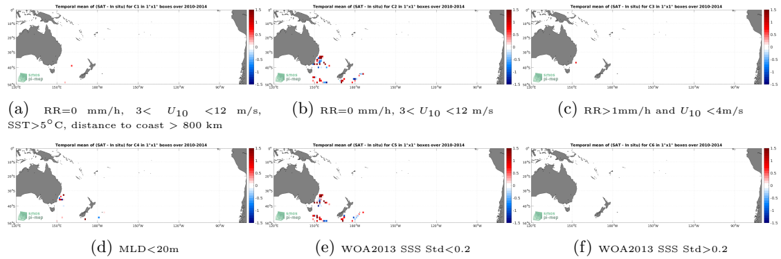
Figure 12: Temporal mean gridded over spatial boxes of size 1^{\circ}\times 1^{\circ} of \Delta\text{SSS} (SMOS SSS L2Q v331 - No FLAG (CMEMS-CATDS-CPDC) - Marine mammals) for 6 different subdatasets corresponding to:RR=0 mm/h, 3 < U_{10} < 12 m/s, SST >5^{\circ}\text{C} , distance to coast > 800 km (a), RR=0 mm/h, 3 < U_{10} < 12 m/s (b), RR >1 mm/h and U_{10} < 4 m/s (c),MLD <20 m (d),WOA2013 SSS Std <0.2 (e),WOA2013 SSS Std >0.2 (f).
