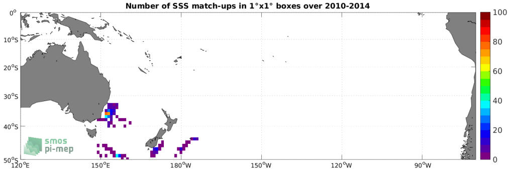
Figure 4: Number of SSS match-ups between Marine mammals SSS and the SMOS SSS L2Q v331 - No FLAG (CMEMS-CATDS-CPDC) SSS product for the South Pacific Ocean Pi-MEP region over 1^\circ \times 1^\circ boxes and for the full satellite product period.
