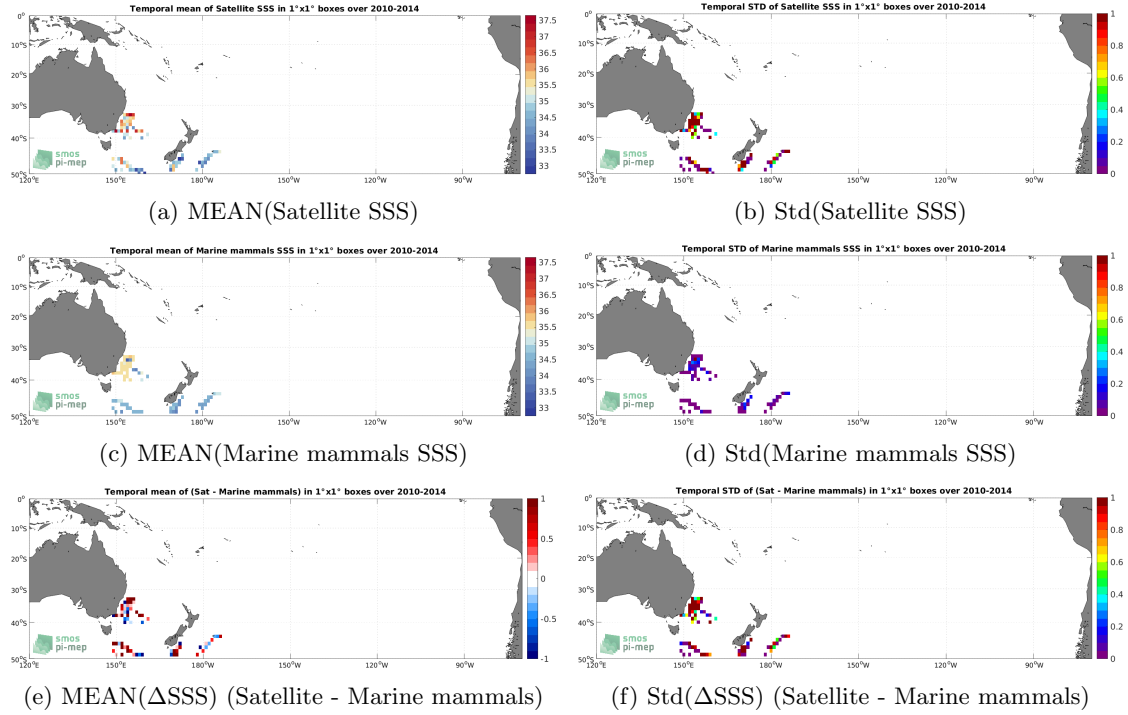
Figure 6: Temporal mean (left) and Std (right) of SSS from SMOS SSS L2Q v331 - No FLAG (CMEMS-CATDS-CPDC) (top), Marine mammals (middle), and of \Delta SSS (Satellite - Marine mammals). Only match-up pairs are used to generate these maps.
