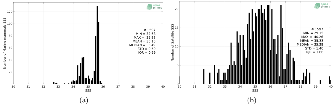
Figure 2: Histograms of SSS from Marine mammals (a) and SMOS SSS L2Q v331 - No FLAG (CMEMS-CATDS-CPDC) (b) considering all match-up pairs per bins of 0.1 over the South Pacific Ocean Pi-MEP region and for the full satellite product period.
