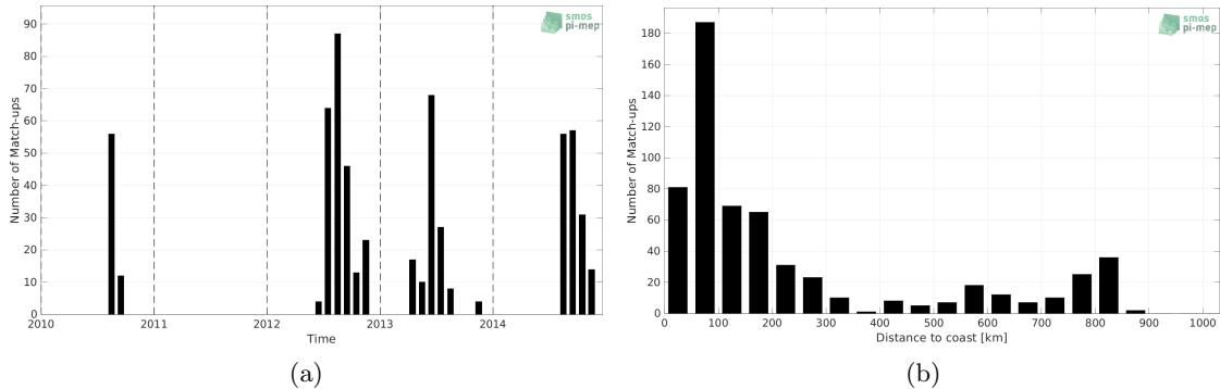
Figure 1: Number of match-ups between Marine mammals and SMOS SSS L2Q v331 - No FLAG (CMEMS-CATDS-CPDC) SSS as a function of time (a) and as function of the distance to coast (b) over the South Pacific Ocean Pi-MEP region and for the full satellite product period.
