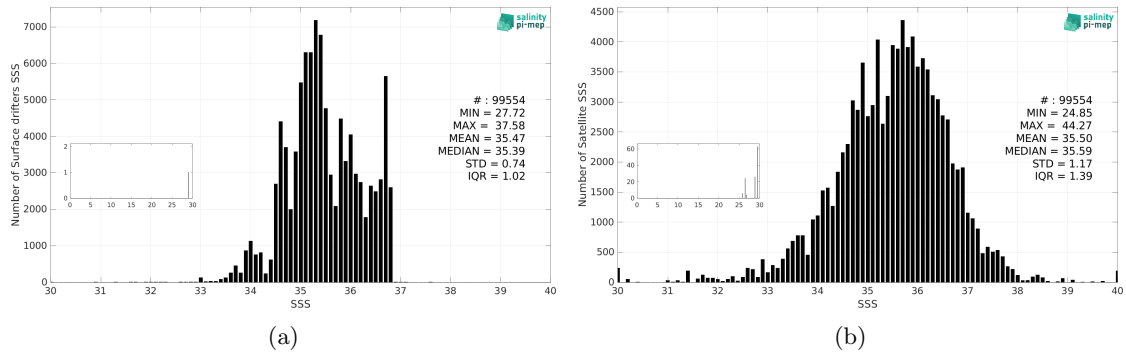
Figure 3: Histograms of SSS from Surface drifters (a) and SMOS SSS L2Q v331 - No FLAG (CMEMS-CATDS-CPDC) (b) considering all match-up pairs per bins of 0.1 over the South Pacific Ocean Pi-MEP region and for the full satellite product period.
