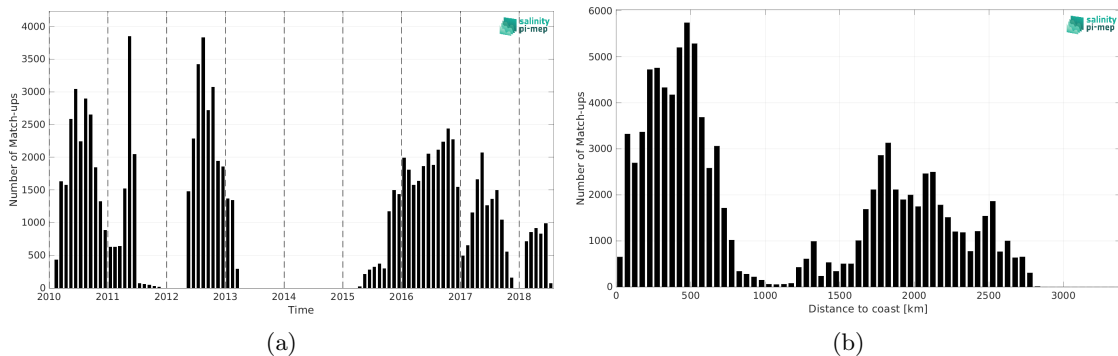
Figure 2: Number of match-ups between Surface drifters and SMOS SSS L2Q v331 - No FLAG (CMEMS-CATDS-CPDC) SSS as a function of time (a) and as function of the distance to coast (b) over the South Pacific Ocean Pi-MEP region and for the full satellite product period.
