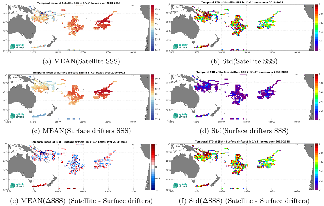
Figure 6: Temporal mean (left) and Std (right) of SSS from SMOS SSS L2Q v331 - No FLAG (CMEMS-CATDS-CPDC) (top), Surface drifters (middle), and of \Delta SSS (Satellite - Surface drifters). Only match-up pairs are used to generate these maps.
