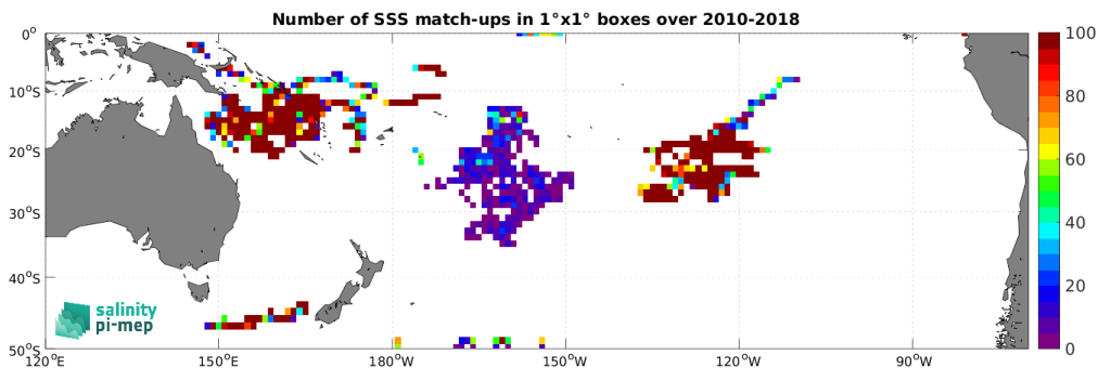
Figure 4: Number of SSS match-ups between Surface drifters SSS and the SMOS SSS L2Q v331 - No FLAG (CMEMS-CATDS-CPDC) SSS product for the South Pacific Ocean Pi-MEP region over 1^\circ \times 1^\circ boxes and for the full satellite product period.
