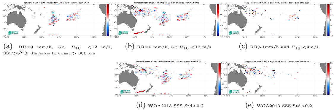
Figure 13: Temporal mean gridded over spatial boxes of size 1^\circ \times 1^\circ of \Delta SSS (SMOS SSS L2Q v331 - No FLAG (CMEMS-CATDS-CPDC) - Surface drifters) for 5 different subdatasets corresponding to:RR=0 mm/h, 3 < U_{10} < 12 m/s, SST >5^\circ C, distance to coast > 800 km (a), RR=0 mm/h, 3 < U_{10} < 12 m/s (b), RR >1 mm/h and U_{10} < 4 m/s (c), WOA2013 SSS Std <0.2 (d), WOA2013 SSS Std >0.2 (e).
