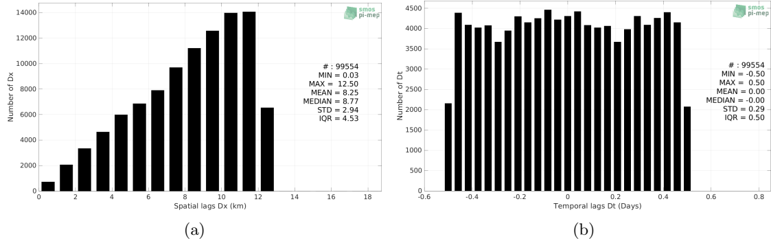
Figure 4: Histograms of the spatial (a) and temporal (b) lags between the location/time of the Surface drifters measurement and the date of the corresponding SMOS SSS L2Q v331 - No FLAG (CMEMS-CATDS-CPDC) SSS pixel.
