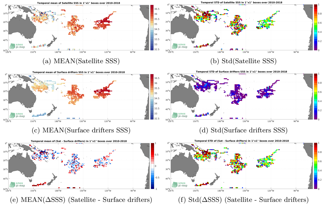
Figure 5: Temporal mean (left) and Std (right) of SSS from SMOS SSS L2Q v331 - No FLAG (CMEMS-CATDS-CPDC) (top), Surface drifters (middle), and of \Delta SSS (Satellite - Surface drifters). Only match-up pairs are used to generate these maps.
