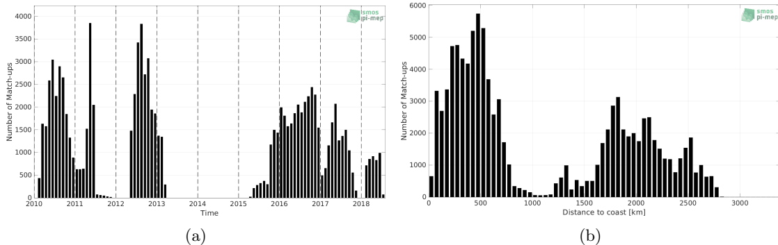
Figure 1: Number of match-ups between Surface drifters and SMOS SSS L2Q v331 - No FLAG (CMEMS-CATDS-CPDC) SSS as a function of time (a) and as function of the distance to coast (b) over the South Pacific Ocean Pi-MEP region and for the full satellite product period.
