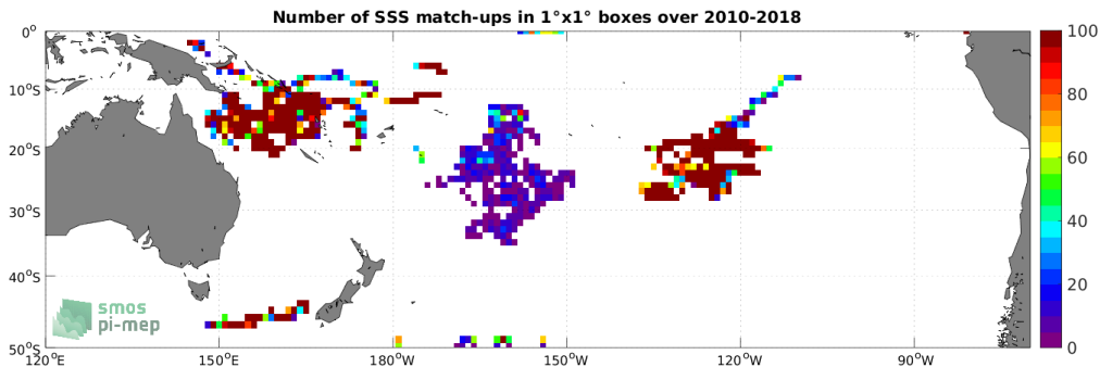
Figure 3: Number of SSS match-ups between Surface drifters SSS and the SMOS SSS L2Q v331 - No FLAG (CMEMS-CATDS-CPDC) SSS product for the South Pacific Ocean Pi-MEP region over 1^\circ \times 1^\circ boxes and for the full satellite product period.
