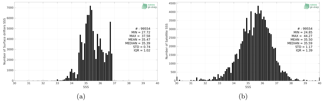
Figure 2: Histograms of SSS from Surface drifters (a) and SMOS SSS L2Q v331 - No FLAG (CMEMS-CATDS-CPDC) (b) considering all match-up pairs per bins of 0.1 over the South Pacific Ocean Pi-MEP region and for the full satellite product period.
