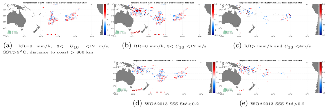
Figure 11: Temporal mean gridded over spatial boxes of size 1^\circ \times 1^\circ of \Delta SSS (SMOS SSS L2Q v331 - No FLAG (CMEMS-CATDS-CPDC) - Surface drifters) for 5 different subdatasets corresponding to:RR=0 mm/h, 3 < U_{10} < 12 m/s, SST >5^\circ C, distance to coast > 800 km (a), RR=0 mm/h, 3 < U_{10} < 12 m/s (b), RR >1 mm/h and U_{10} < 4 m/s (c), WOA2013 SSS Std <0.2 (d), WOA2013 SSS Std >0.2 (e).
