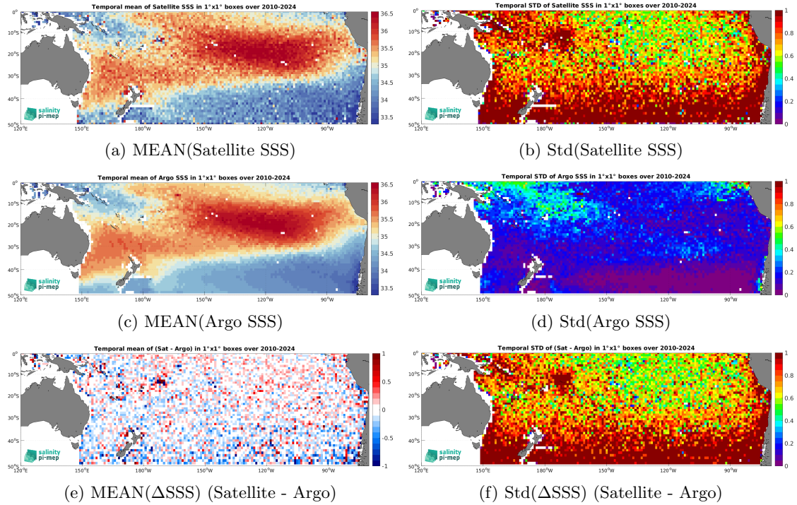
Figure 7: Temporal mean (left) and Std (right) of SSS from SMOS SSS L2Q v331 - No FLAG (CMEMS-CATDS-CPDC) (top), Argo (middle), and of \Delta SSS (Satellite - Argo). Only match-up pairs are used to generate these maps.
