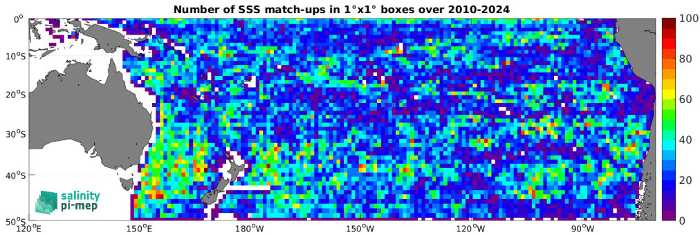
Figure 5: Number of SSS match-ups between Argo SSS and the SMOS SSS L2Q v331 - No FLAG (CMEMS-CATDS-CPDC) SSS product for the South Pacific Ocean Pi-MEP region over 1^\circ \times 1^\circ boxes and for the full satellite product period.
