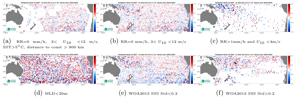
Figure 14: Temporal mean gridded over spatial boxes of size 1^\circ \times 1^\circ of \Delta SSS (SMOS SSS L2Q v331 - No FLAG (CMEMS-CATDS-CPDC) - Argo) for 6 different subdatasets corresponding to:RR=0 mm/h, 3 < U_{10} < 12 m/s, SST >5^\circ C, distance to coast > 800 km (a), RR=0 mm/h, 3 < U_{10} < 12 m/s (b), RR >1 mm/h and U_{10} < 4 m/s (c),MLD <20 m (d),WOA2013 SSS Std <0.2 (e),WOA2013 SSS Std >0.2 (f).
