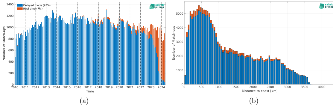
Figure 2: Number of match-ups between Argo and SMOS SSS L2Q v331 - No FLAG (CMEMS-CATDS-CPDC) SSS as a function of time (a) and as function of the distance to coast (b) over the South Pacific Ocean Pi-MEP region and for the full satellite product period.
