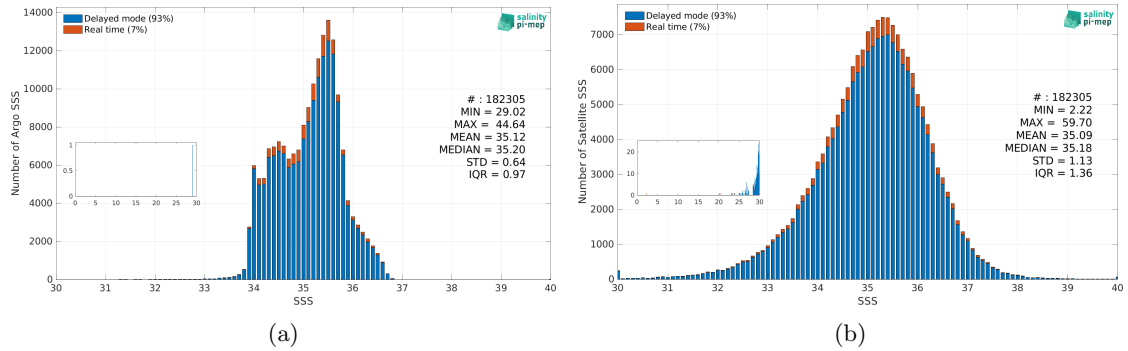
Figure 3: Histograms of SSS from Argo (a) and SMOS SSS L2Q v331 - No FLAG (CMEMS-CATDS-CPDC) (b) considering all match-up pairs per bins of 0.1 over the South Pacific Ocean Pi-MEP region and for the full satellite product period.
