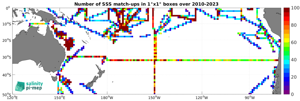
Figure 5: Number of SSS match-ups between TSG (SAMOS) SSS and the SMOS SSS L3 v9 - 9 Days (CATDS-CEC-LOCEAN) SSS product for the South Pacific Ocean Pi-MEP region over 1^\circ \times 1^\circ boxes and for the full satellite product period.
