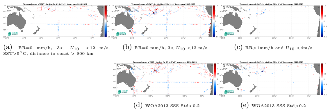
Figure 14: Temporal mean gridded over spatial boxes of size 1^\circ \times 1^\circ of \Delta\text{SSS} (SMOS SSS L3 v9 - 9 Days (CATDS-CEC-LOCEAN) - TSG (SAMOS)) for 5 different subdatasets corresponding to:RR=0 mm/h, 3 < U_{10} < 12 m/s, SST>5°C, distance to coast > 800 km (a), RR=0 mm/h, 3 < U_{10} < 12 m/s (b), RR>1mm/h and U_{10} < 4 m/s (c), WOA2013 SSS Std<0.2 (d), WOA2013 SSS Std>0.2 (e).
