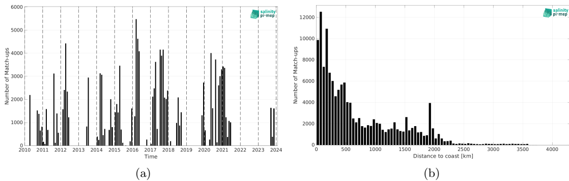
Figure 2: Number of match-ups between TSG (SAMOS) and SMOS SSS L3 v9 - 9 Days (CATDS-CEC-LOCEAN) SSS as a function of time (a) and as function of the distance to coast (b) over the South Pacific Ocean Pi-MEP region and for the full satellite product period.
