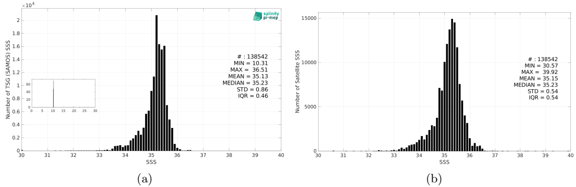
Figure 3: Histograms of SSS from TSG (SAMOS) (a) and SMOS SSS L3 v9 - 9 Days (CATDS-CEC-LOCEAN) (b) considering all match-up pairs per bins of 0.1 over the South Pacific Ocean Pi-MEP region and for the full satellite product period.
