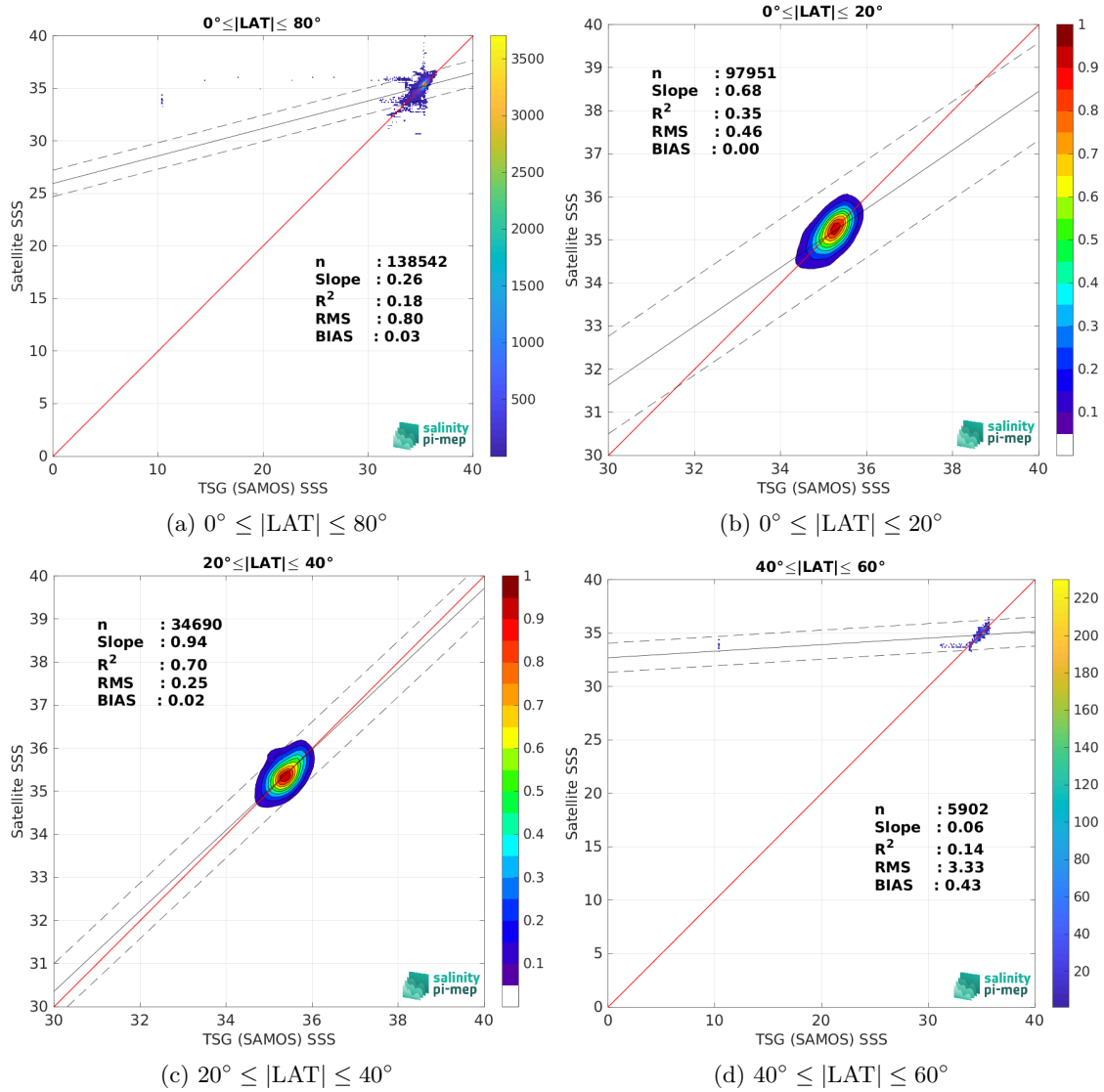
Figure 10: Contour maps of the concentration of SMOS SSS L3 v9 - 9 Days (CATDS-CEC-LOCEAN) SSS (y-axis) versus TSG (SAMOS) SSS (x-axis) at match-up pairs for different latitude bands. For each plot, the red line shows x=y . The black thin and dashed lines indicate a linear fit through the data cloud and the \pm 95\% confidence levels, respectively. The number match-up pairs n , the slope and R^2 coefficient of the linear fit, the root mean square (RMS) and the mean bias between satellite and in situ data are indicated for each latitude band in each plots.
