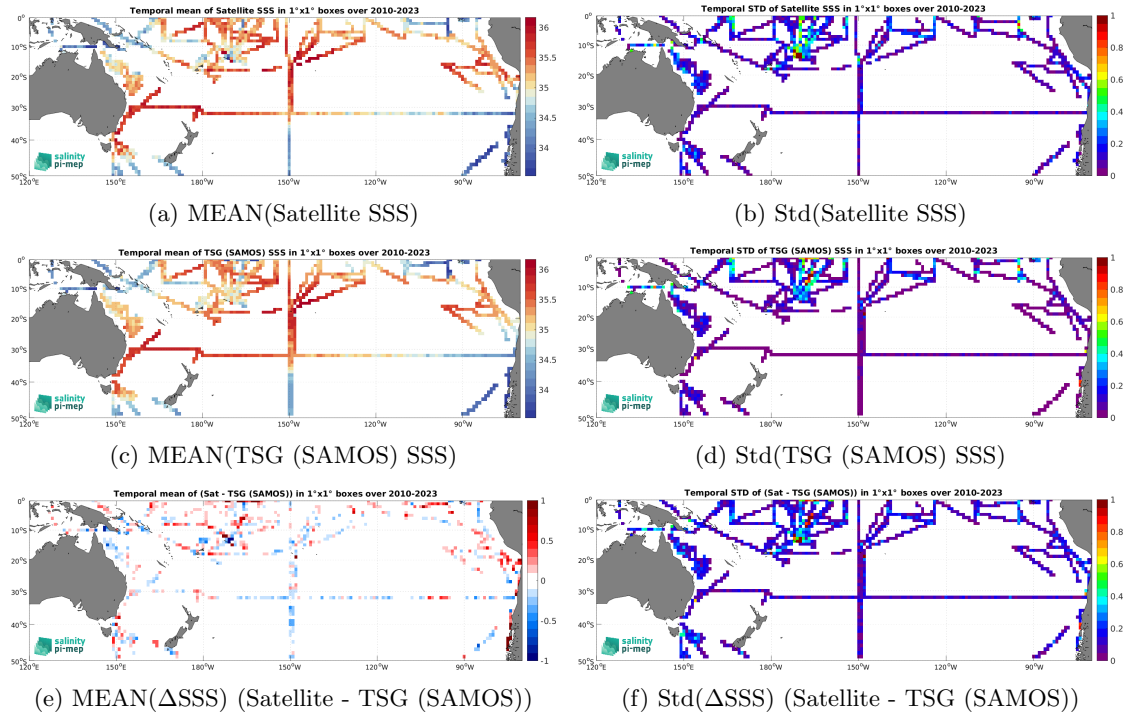
Figure 7: Temporal mean (left) and Std (right) of SSS from SMOS SSS L3 v9 - 9 Days (CATDS-CEC-LOCEAN) (top), TSG (SAMOS) (middle), and of \Delta SSS (Satellite - TSG (SAMOS)). Only match-up pairs are used to generate these maps.
