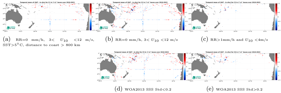
Figure 12: Temporal mean gridded over spatial boxes of size 1^\circ \times 1^\circ of \Delta SSS (SMOS SSS L3 v9 - 9 Days (CATDS-CEC-LOCEAN) - TSG (SAMOS)) for 5 different subdatasets corresponding to:RR=0 mm/h, 3 < U_{10} < 12 m/s, SST >5^\circ C, distance to coast > 800 km (a), RR=0 mm/h, 3 < U_{10} < 12 m/s (b), RR >1 mm/h and U_{10} < 4 m/s (c), WOA2013 SSS Std <0.2 (d), WOA2013 SSS Std >0.2 (e).
