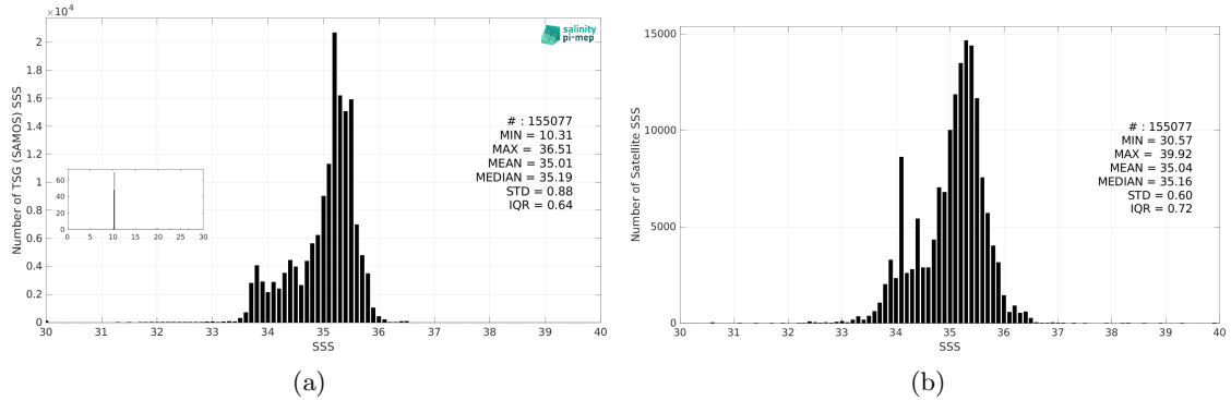
Figure 2: Histograms of SSS from TSG (SAMOS) (a) and SMOS SSS L3 v9 - 9 Days (CATDS-CEC-LOCEAN) (b) considering all match-up pairs per bins of 0.1 over the South Pacific Ocean Pi-MEP region and for the full satellite product period.
