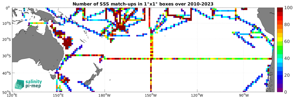
Figure 4: Number of SSS match-ups between TSG (SAMOS) SSS and the SMOS SSS L3 v9 - 9 Days (CATDS-CEC-LOCEAN) SSS product for the South Pacific Ocean Pi-MEP region over 1^\circ \times 1^\circ boxes and for the full satellite product period.
