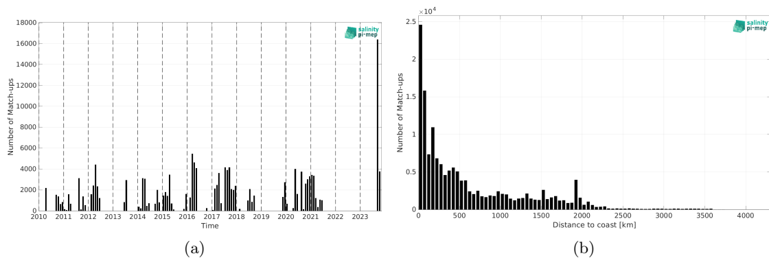
Figure 1: Number of match-ups between TSG (SAMOS) and SMOS SSS L3 v9 - 9 Days (CATDS-CEC-LOCEAN) SSS as a function of time (a) and as function of the distance to coast (b) over the South Pacific Ocean Pi-MEP region and for the full satellite product period.
