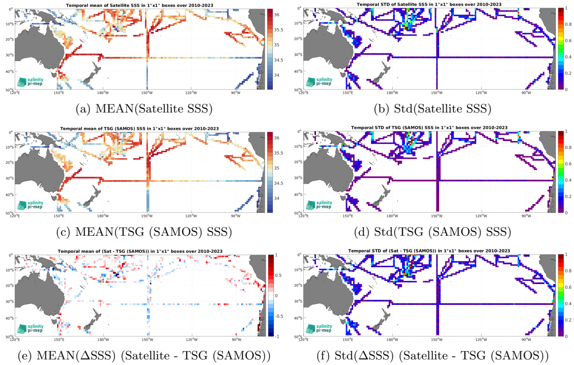
Figure 6: Temporal mean (left) and Std (right) of SSS from SMOS SSS L3 v9 - 9 Days (CATDS-CEC-LOCEAN) (top), TSG (SAMOS) (middle), and of \Delta SSS (Satellite - TSG (SAMOS)). Only match-up pairs are used to generate these maps.
