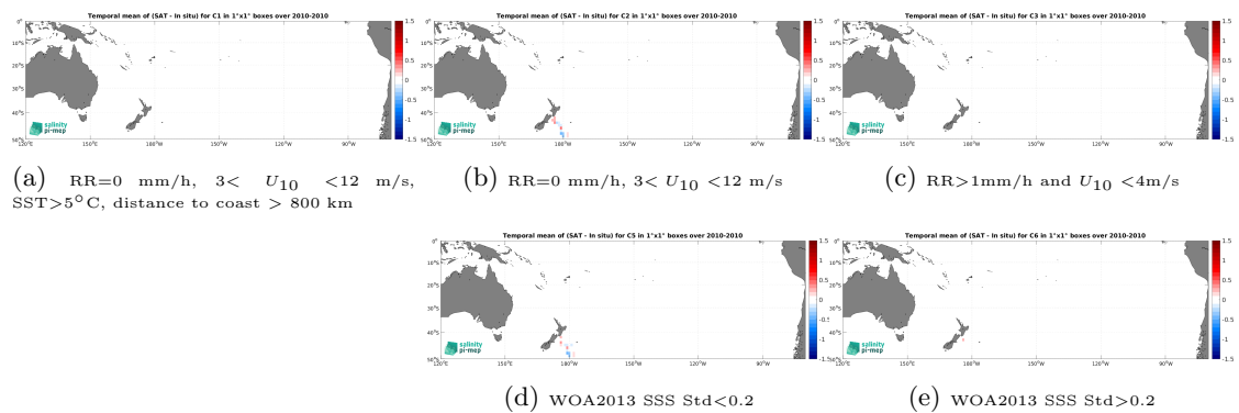
Figure 14: Temporal mean gridded over spatial boxes of size 1^\circ \times 1^\circ of \Delta\text{SSS} (SMOS SSS L3 v9 - 9 Days (CATDS-CEC-LOCEAN) - TSG (Polarstern)) for 5 different subdatasets corresponding to:RR=0 mm/h, 3 < U_{10} < 12 m/s, SST>5°C, distance to coast > 800 km (a), RR=0 mm/h, 3 < U_{10} < 12 m/s (b), RR>1mm/h and U_{10} < 4 m/s (c), WOA2013 SSS Std<0.2 (d), WOA2013 SSS Std>0.2 (e).
