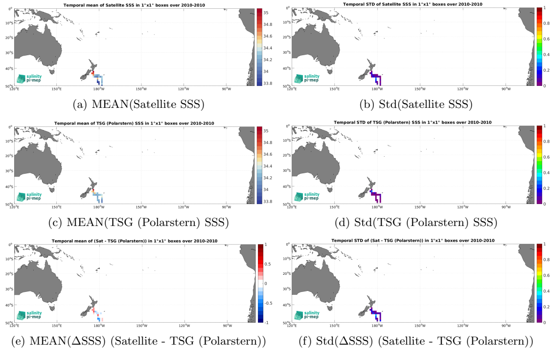
Figure 7: Temporal mean (left) and Std (right) of SSS from SMOS SSS L3 v9 - 9 Days (CATDS-CEC-LOCEAN) (top), TSG (Polarstern) (middle), and of \Delta SSS (Satellite - TSG (Polarstern)). Only match-up pairs are used to generate these maps.
