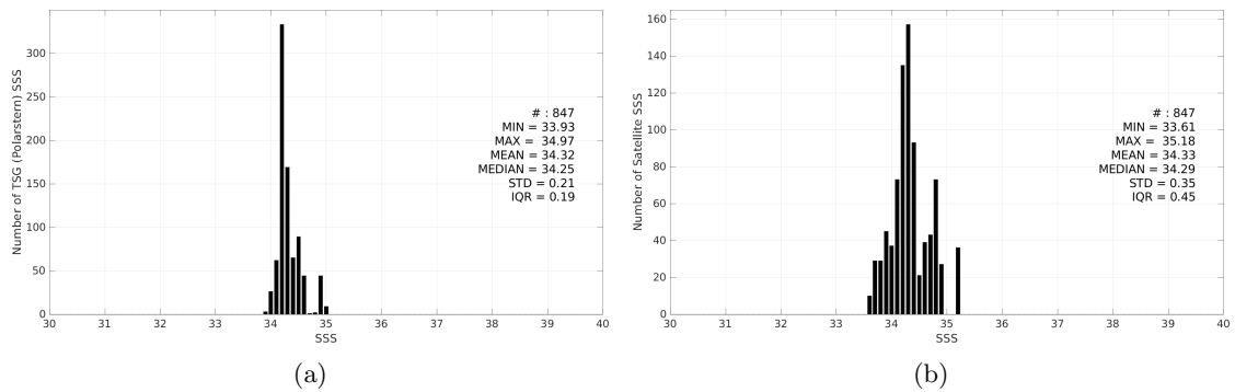
Figure 3: Histograms of SSS from TSG (Polarstern) (a) and SMOS SSS L3 v9 - 9 Days (CATDS-CEC-LOCEAN) (b) considering all match-up pairs per bins of 0.1 over the South Pacific Ocean Pi-MEP region and for the full satellite product period.
