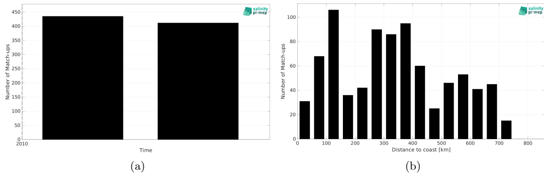
Figure 1: Number of match-ups between TSG (Polarstern) and SMOS SSS L3 v9 - 9 Days (CATDS-CEC-LOCEAN) SSS as a function of time (a) and as function of the distance to coast (b) over the South Pacific Ocean Pi-MEP region and for the full satellite product period.
