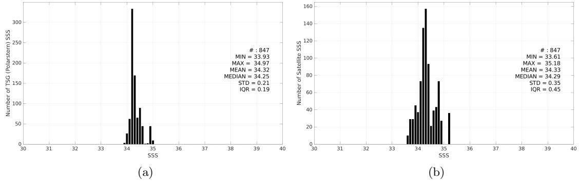
Figure 2: Histograms of SSS from TSG (Polarstern) (a) and SMOS SSS L3 v9 - 9 Days (CATDS-CEC-LOCEAN) (b) considering all match-up pairs per bins of 0.1 over the South Pacific Ocean Pi-MEP region and for the full satellite product period.
