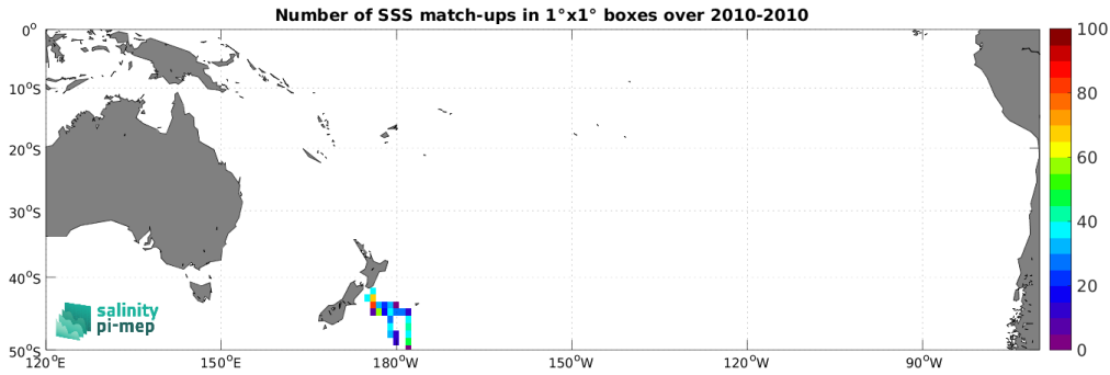
Figure 4: Number of SSS match-ups between TSG (Polarstern) SSS and the SMOS SSS L3 v9 - 9 Days (CATDS-CEC-LOCEAN) SSS product for the South Pacific Ocean Pi-MEP region over 1^\circ \times 1^\circ boxes and for the full satellite product period.
