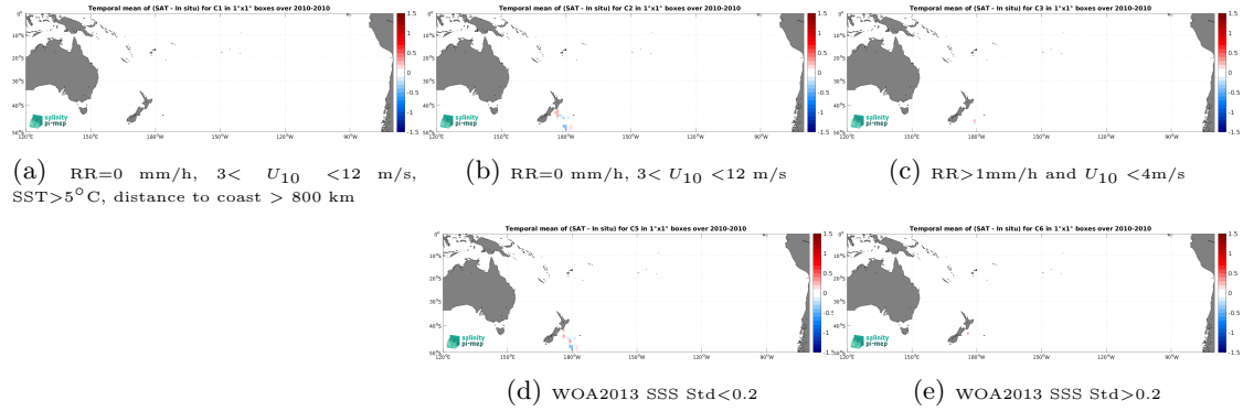
Figure 12: Temporal mean gridded over spatial boxes of size 1^{\circ}\times 1^{\circ} of \Delta\text{SSS} (SMOS SSS L3 v9 - 9 Days (CATDS-CEC-LOCEAN) - TSG (Polarstern)) for 5 different subdatasets corresponding to:RR=0 mm/h, 3 < U_{10} < 12 m/s, SST > 5^{\circ}\text{C} , distance to coast > 800 km (a), RR=0 mm/h, 3 < U_{10} < 12 m/s (b), RR > 1 mm/h and U_{10} < 4 m/s (c), WOA2013 SSS Std < 0.2 (d), WOA2013 SSS Std > 0.2 (e).
