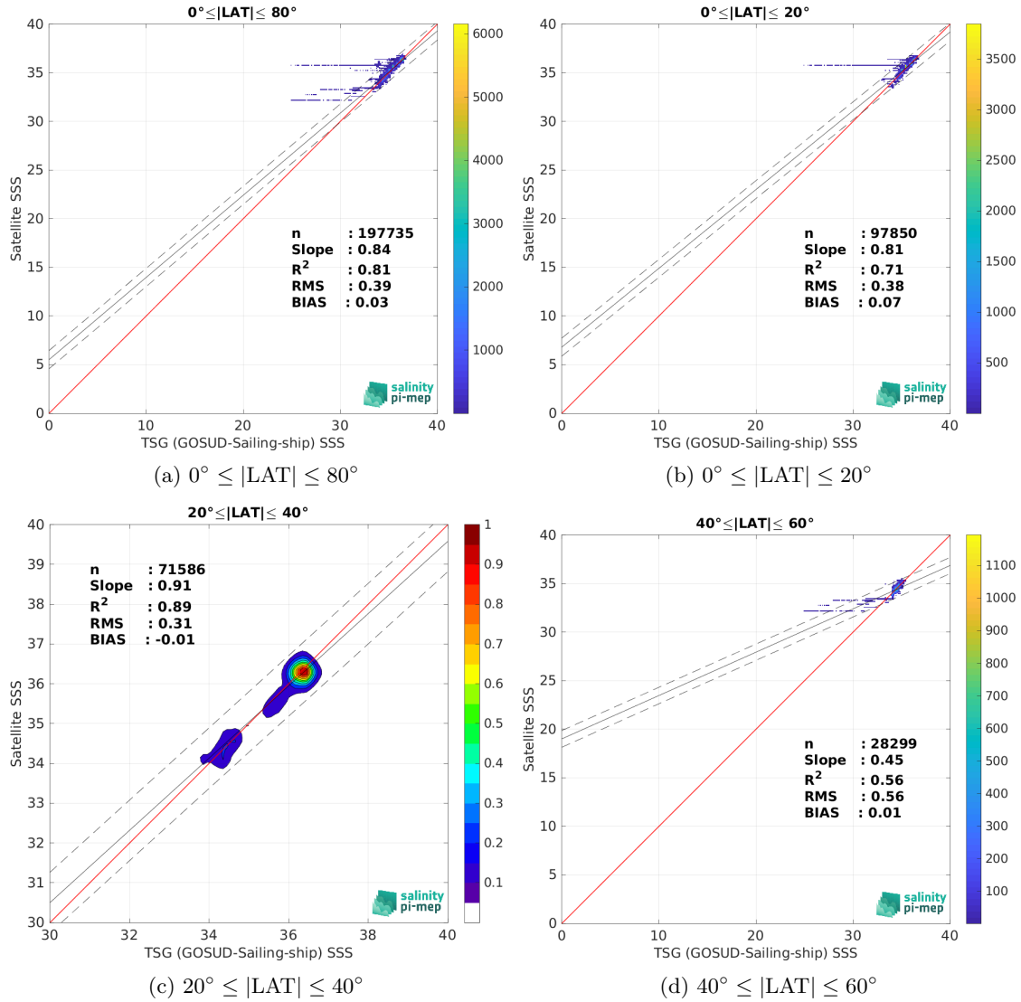
Figure 10: Contour maps of the concentration of SMOS SSS L3 v9 - 9 Days (CATDS-CEC-LOCEAN) SSS (y-axis) versus TSG (GOSUD-Sailing-ship) SSS (x-axis) at match-up pairs for different latitude bands. For each plot, the red line shows x=y . The black thin and dashed lines indicate a linear fit through the data cloud and the \pm 95\% confidence levels, respectively. The number match-up pairs n , the slope and R^2 coefficient of the linear fit, the root mean square (RMS) and the mean bias between satellite and in situ data are indicated for each latitude band in each plots.
