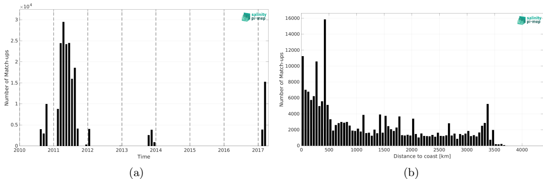
Figure 2: Number of match-ups between TSG (GOSUD-Sailing-ship) and SMOS SSS L3 v9 - 9 Days (CATDS-CEC-LOCEAN) SSS as a function of time (a) and as function of the distance to coast (b) over the South Pacific Ocean Pi-MEP region and for the full satellite product period.
