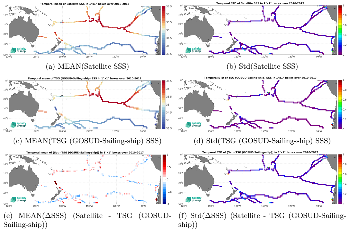
Figure 7: Temporal mean (left) and Std (right) of SSS from SMOS SSS L3 v9 - 9 Days (CATDS-CEC-LOCEAN) (top), TSG (GOSUD-Sailing-ship) (middle), and of \Delta SSS (Satellite - TSG (GOSUD-Sailing-ship)). Only match-up pairs are used to generate these maps.
