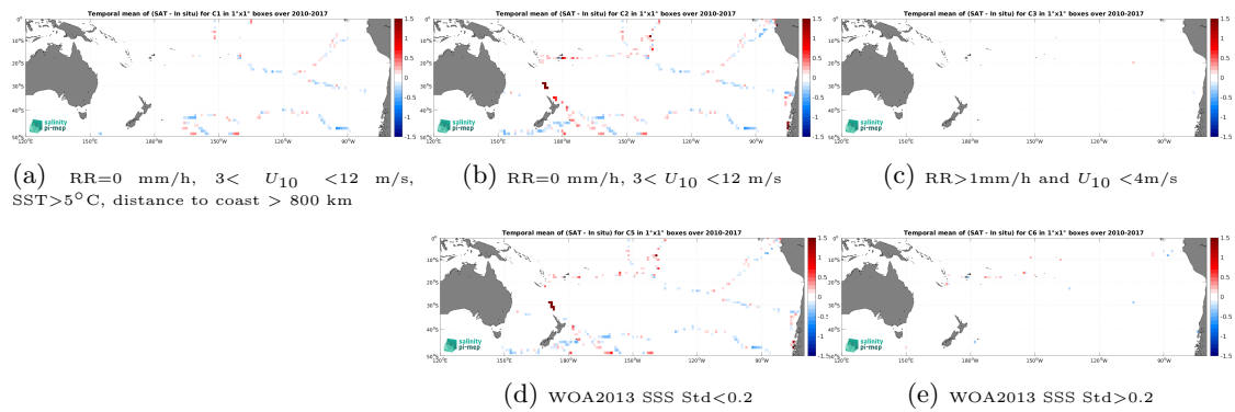
Figure 14: Temporal mean gridded over spatial boxes of size 1^\circ \times 1^\circ of \Delta\text{SSS} (SMOS SSS L3 v9 - 9 Days (CATDS-CEC-LOCEAN) - TSG (GOSUD-Sailing-ship)) for 5 different subdatasets corresponding to:RR=0 mm/h, 3 < U_{10} < 12 m/s, SST>5°C, distance to coast > 800 km (a), RR=0 mm/h, 3 < U_{10} < 12 m/s (b), RR>1mm/h and U_{10} < 4 m/s (c), WOA2013 SSS Std<0.2 (d), WOA2013 SSS Std>0.2 (e).
