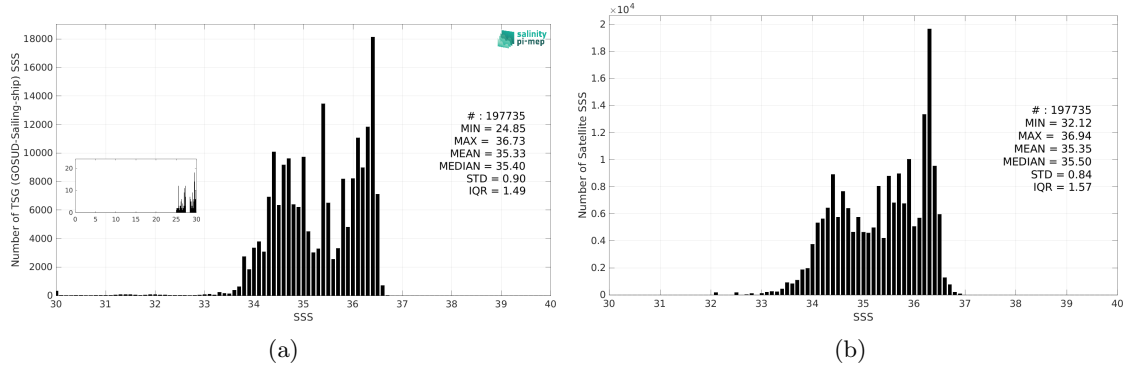
Figure 2: Histograms of SSS from TSG (GOSUD-Sailing-ship) (a) and SMOS SSS L3 v9 - 9 Days (CATDS-CEC-LOCEAN) (b) considering all match-up pairs per bins of 0.1 over the South Pacific Ocean Pi-MEP region and for the full satellite product period.
