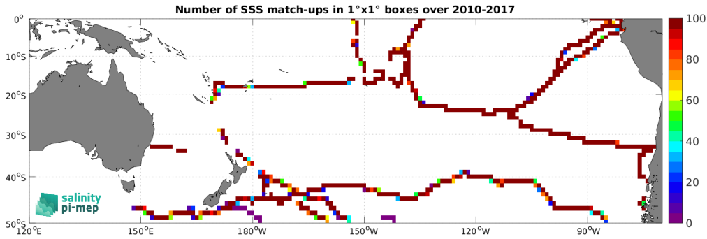
Figure 4: Number of SSS match-ups between TSG (GOSUD-Sailing-ship) SSS and the SMOS SSS L3 v9 - 9 Days (CATDS-CEC-LOCEAN) SSS product for the South Pacific Ocean Pi-MEP region over 1^\circ \times 1^\circ boxes and for the full satellite product period.
