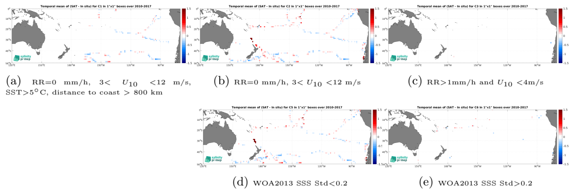
Figure 12: Temporal mean gridded over spatial boxes of size 1^\circ \times 1^\circ of \Delta SSS (SMOS SSS L3 v9 - 9 Days (CATDS-CEC-LOCEAN) - TSG (GOSUD-Sailing-ship)) for 5 different subdatasets corresponding to:RR=0 mm/h, 3 < U_{10} < 12 m/s, SST >5^\circ\text{C} , distance to coast > 800 km (a), RR=0 mm/h, 3 < U_{10} < 12 m/s (b), RR >1 mm/h and U_{10} < 4 m/s (c), WOA2013 SSS Std <0.2 (d), WOA2013 SSS Std >0.2 (e).
