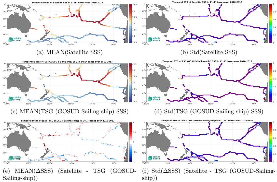
Figure 6: Temporal mean (left) and Std (right) of SSS from SMOS SSS L3 v9 - 9 Days (CATDS-CEC-LOCEAN) (top), TSG (GOSUD-Sailing-ship) (middle), and of \Delta SSS (Satellite - TSG (GOSUD-Sailing-ship)). Only match-up pairs are used to generate these maps.
