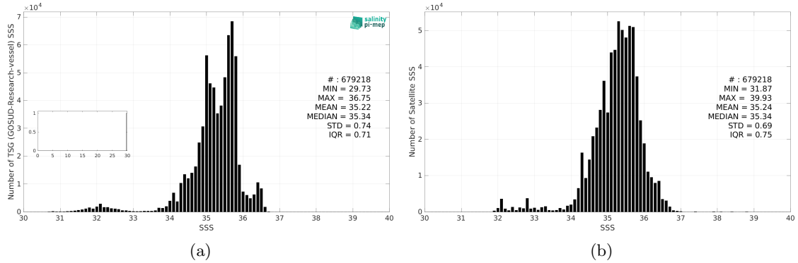
Figure 2: Histograms of SSS from TSG (GOSUD-Research-vessel) (a) and SMOS SSS L3 v9 - 9 Days (CATDS-CEC-LOCEAN) (b) considering all match-up pairs per bins of 0.1 over the South Pacific Ocean Pi-MEP region and for the full satellite product period.
