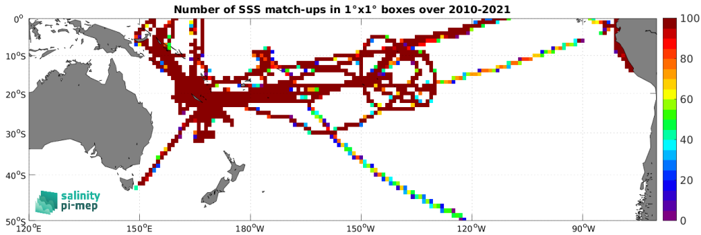
Figure 4: Number of SSS match-ups between TSG (GOSUD-Research-vessel) SSS and the SMOS SSS L3 v9 - 9 Days (CATDS-CEC-LOCEAN) SSS product for the South Pacific Ocean Pi-MEP region over 1^\circ \times 1^\circ boxes and for the full satellite product period.
