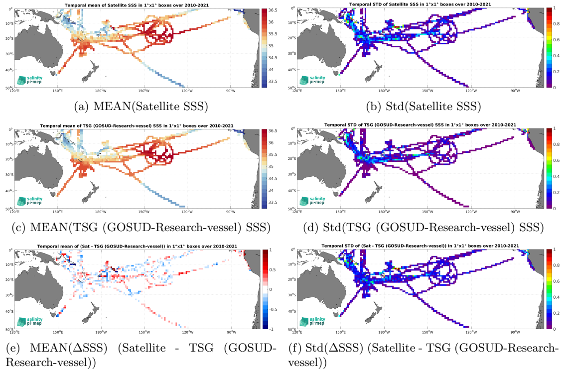
Figure 6: Temporal mean (left) and Std (right) of SSS from SMOS SSS L3 v9 - 9 Days (CATDS-CEC-LOCEAN) (top), TSG (GOSUD-Research-vessel) (middle), and of \Delta SSS (Satellite - TSG (GOSUD-Research-vessel)). Only match-up pairs are used to generate these maps.
