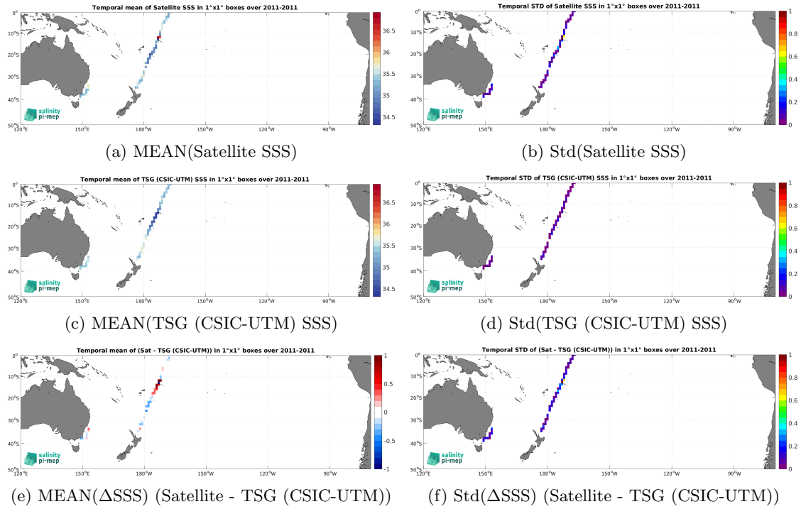
Figure 7: Temporal mean (left) and Std (right) of SSS from SMOS SSS L3 v9 - 9 Days (CATDS-CEC-LOCEAN) (top), TSG (CSIC-UTM) (middle), and of \Delta SSS (Satellite - TSG (CSIC-UTM)). Only match-up pairs are used to generate these maps.
