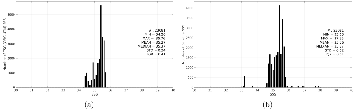
Figure 3: Histograms of SSS from TSG (CSIC-UTM) (a) and SMOS SSS L3 v9 - 9 Days (CATDS-CEC-LOCEAN) (b) considering all match-up pairs per bins of 0.1 over the South Pacific Ocean Pi-MEP region and for the full satellite product period.
