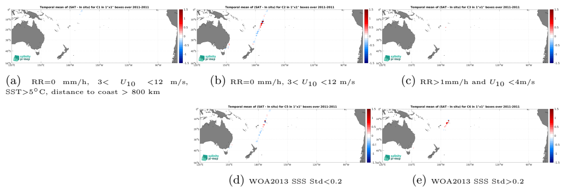
Figure 14: Temporal mean gridded over spatial boxes of size 1^\circ \times 1^\circ of \Delta\text{SSS} (SMOS SSS L3 v9 - 9 Days (CATDS-CEC-LOCEAN) - TSG (CSIC-UTM)) for 5 different subdatasets corresponding to:RR=0 mm/h, 3 < U_{10} < 12 m/s, SST>5°C, distance to coast > 800 km (a), RR=0 mm/h, 3 < U_{10} < 12 m/s (b), RR>1mm/h and U_{10} < 4 m/s (c), WOA2013 SSS Std<0.2 (d), WOA2013 SSS Std>0.2 (e).
