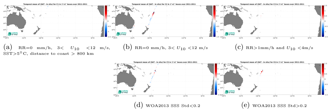
Figure 14: Temporal mean gridded over spatial boxes of size 1^\circ \times 1^\circ of \Delta SSS (SMOS SSS L3 v9 - 9 Days (CATDS-CEC-LOCEAN) - TSG (CSIC-UTM)) for 5 different subdatasets corresponding to:RR=0 mm/h, 3 < U_{10} < 12 m/s, SST >5^\circ\text{C} , distance to coast > 800 km (a), RR=0 mm/h, 3 < U_{10} < 12 m/s (b), RR >1 mm/h and U_{10} < 4 m/s (c), WOA2013 SSS Std <0.2 (d), WOA2013 SSS Std >0.2 (e).
