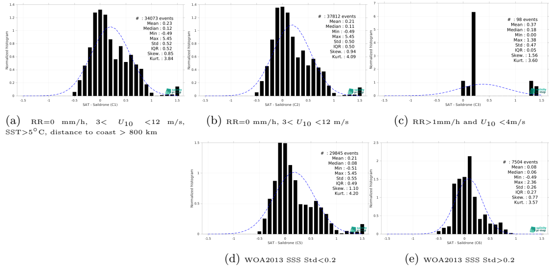
Figure 13: Normalized histogram of \Delta SSS (SMOS SSS L3 v9 - 9 Days (CATDS-CEC-LOCEAN) - Sailability) for 5 different subdatasets corresponding to: RR=0 mm/h, 3 < U_{10} < 12 m/s, SST > 5°C, distance to coast > 800 km (a), RR=0 mm/h, 3 < U_{10} < 12 m/s (b), RR > 1mm/h and U_{10} < 4 m/s (c), WOA2013 SSS Std < 0.2 (d), WOA2013 SSS Std > 0.2 (e).
