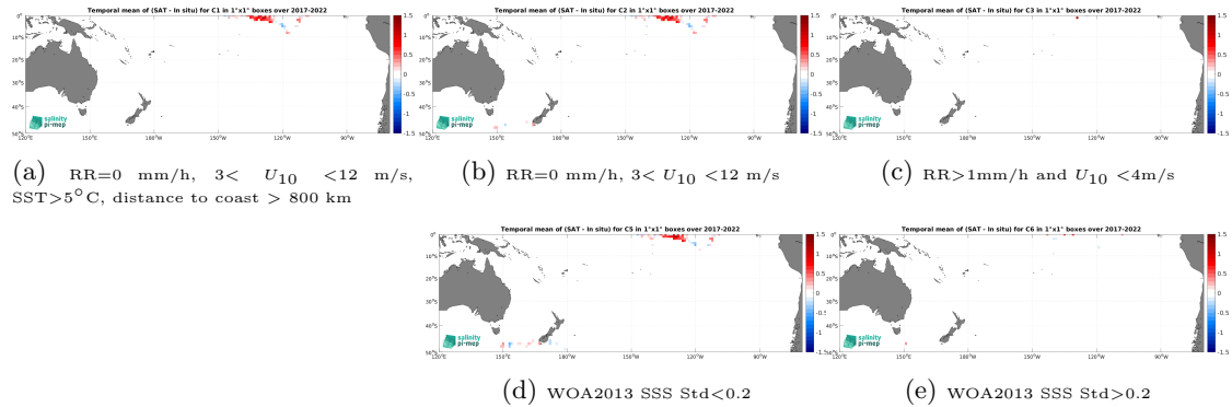
Figure 12: Temporal mean gridded over spatial boxes of size 1^\circ \times 1^\circ of \Delta SSS (SMOS SSS L3 v9 - 9 Days (CATDS-CEC-LOCEAN) - Saildrone) for 5 different subdatasets corresponding to:RR=0 mm/h, 3 < U_{10} < 12 m/s, SST >5^\circ\text{C} , distance to coast > 800 km (a), RR=0 mm/h, 3 < U_{10} < 12 m/s (b), RR >1 mm/h and U_{10} < 4 m/s (c), WOA2013 SSS Std <0.2 (d), WOA2013 SSS Std >0.2 (e).
