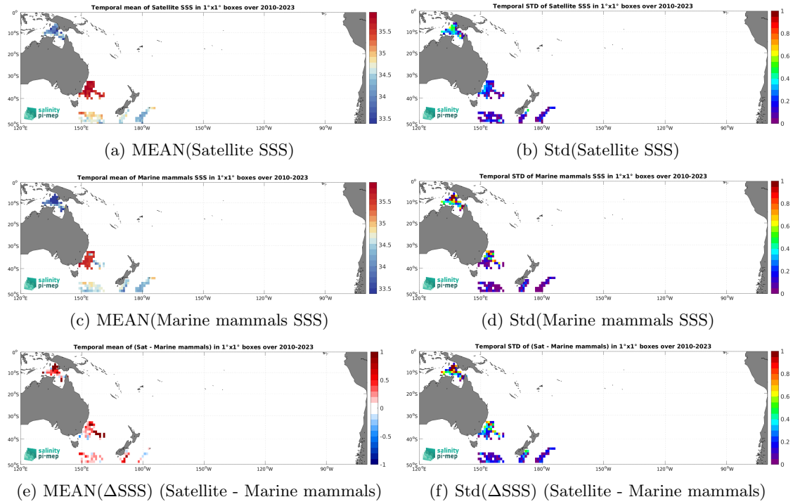
Figure 7: Temporal mean (left) and Std (right) of SSS from SMOS SSS L3 v9 - 9 Days (CATDS-CEC-LOCEAN) (top), Marine mammals (middle), and of \Delta SSS (Satellite - Marine mammals). Only match-up pairs are used to generate these maps.
