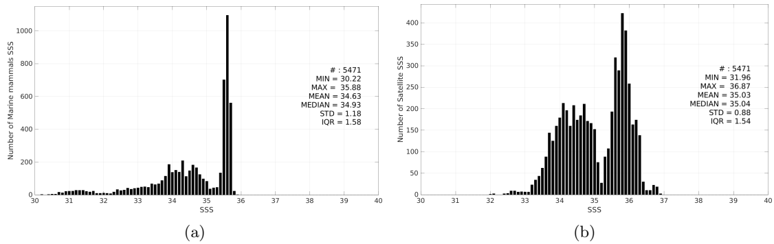
Figure 3: Histograms of SSS from Marine mammals (a) and SMOS SSS L3 v9 - 9 Days (CATDS-CEC-LOCEAN) (b) considering all match-up pairs per bins of 0.1 over the South Pacific Ocean Pi-MEP region and for the full satellite product period.
