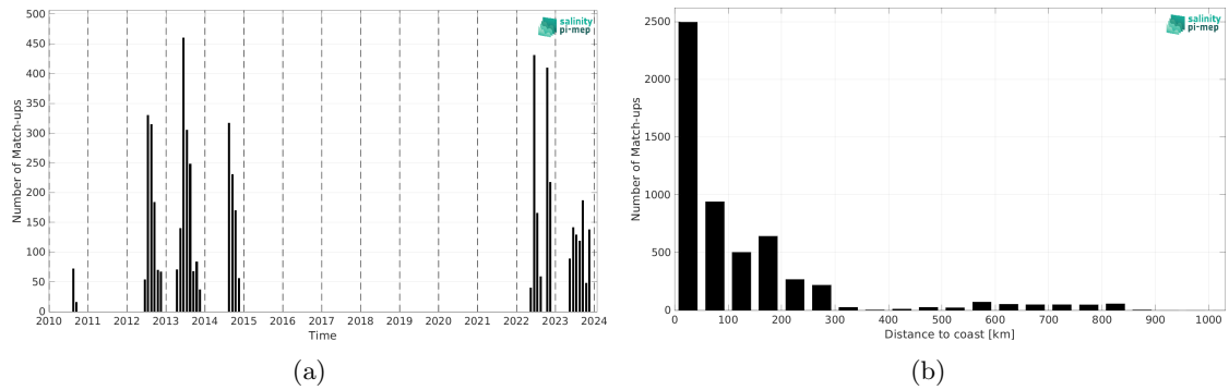
Figure 2: Number of match-ups between Marine mammals and SMOS SSS L3 v9 - 9 Days (CATDS-CEC-LOCEAN) SSS as a function of time (a) and as function of the distance to coast (b) over the South Pacific Ocean Pi-MEP region and for the full satellite product period.
