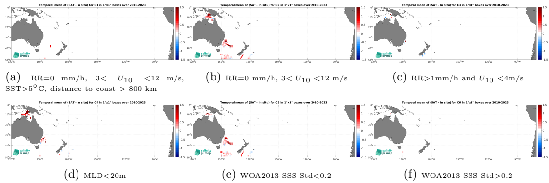
Figure 14: Temporal mean gridded over spatial boxes of size 1^\circ \times 1^\circ of \Delta SSS (SMOS SSS L3 v9 - 9 Days (CATDS-CEC-LOCEAN) - Marine mammals) for 6 different subdatasets corresponding to:RR=0 mm/h, 3 < U_{10} < 12 m/s, SST>5°C, distance to coast > 800 km (a), RR=0 mm/h, 3 < U_{10} < 12 m/s (b), RR>1mm/h and U_{10} < 4 m/s (c),MLD<20m (d),WOA2013 SSS Std<0.2 (e),WOA2013 SSS Std>0.2 (f).
