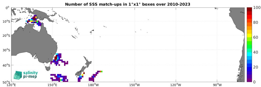
Figure 5: Number of SSS match-ups between Marine mammals SSS and the SMOS SSS L3 v9 - 9 Days (CATDS-CEC-LOCEAN) SSS product for the South Pacific Ocean Pi-MEP region over 1^\circ \times 1^\circ boxes and for the full satellite product period.
