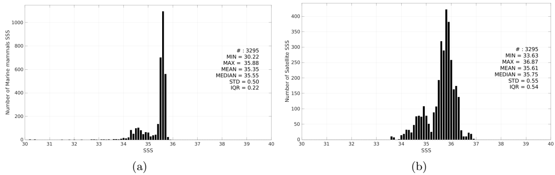
Figure 2: Histograms of SSS from Marine mammals (a) and SMOS SSS L3 v9 - 9 Days (CATDS-CEC-LOCEAN) (b) considering all match-up pairs per bins of 0.1 over the South Pacific Ocean Pi-MEP region and for the full satellite product period.
