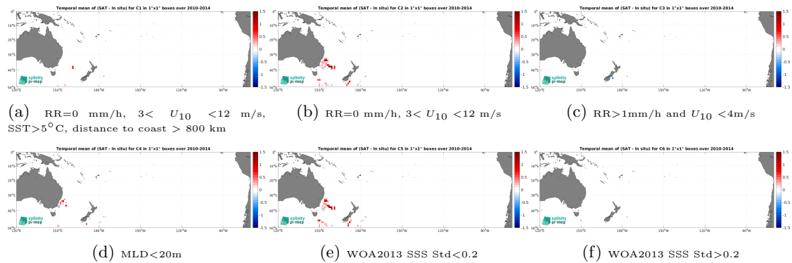
Figure 12: Temporal mean gridded over spatial boxes of size 1^{\circ}\times 1^{\circ} of \Delta\text{SSS} (SMOS SSS L3 v9 - 9 Days (CATDS-CEC-LOCEAN) - Marine mammals) for 6 different subdatasets corresponding to: RR=0 mm/h, 3 < U_{10} < 12 m/s, SST > 5^{\circ}\text{C} , distance to coast > 800 km (a), RR=0 mm/h, 3 < U_{10} < 12 m/s (b), RR > 1 mm/h and U_{10} < 4 m/s (c), MLD < 20\text{m} (d), WOA2013 SSS Std < 0.2 (e), WOA2013 SSS Std > 0.2 (f).
