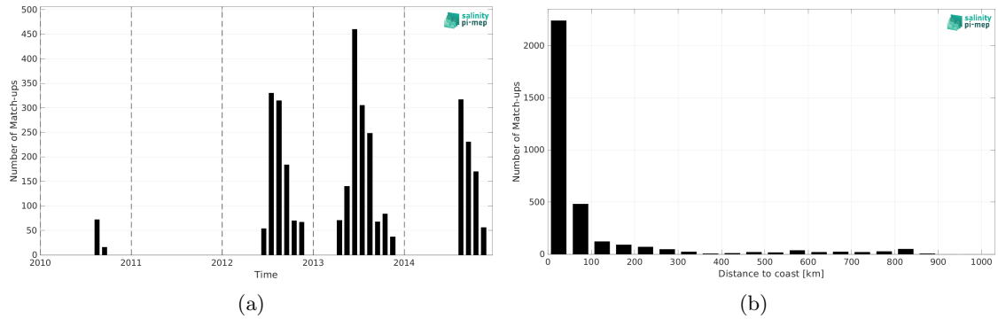
Figure 1: Number of match-ups between Marine mammals and SMOS SSS L3 v9 - 9 Days (CATDS-CEC-LOCEAN) SSS as a function of time (a) and as function of the distance to coast (b) over the South Pacific Ocean Pi-MEP region and for the full satellite product period.
