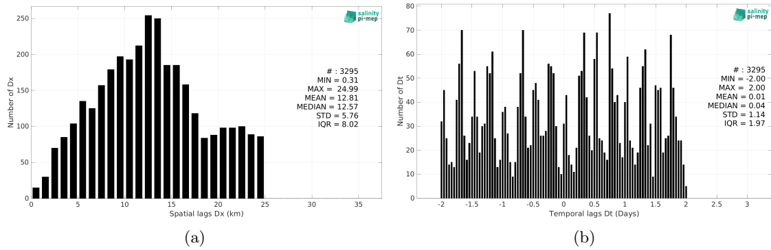
Figure 5: Histograms of the spatial (a) and temporal (b) lags between the location/time of the Marine mammals measurement and the date of the corresponding SMOS SSS L3 v9 - 9 Days (CATDS-CEC-LOCEAN) SSS pixel.
