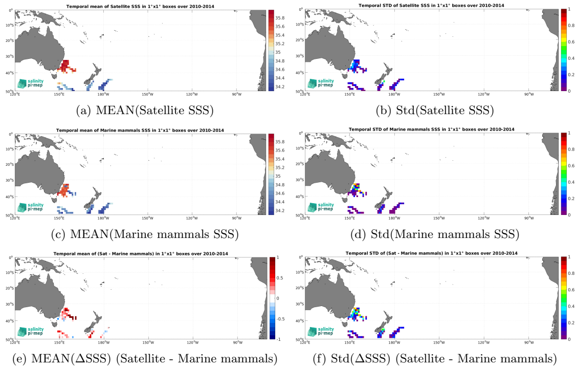
Figure 6: Temporal mean (left) and Std (right) of SSS from SMOS SSS L3 v9 - 9 Days (CATDS-CEC-LOCEAN) (top), Marine mammals (middle), and of \Delta SSS (Satellite - Marine mammals). Only match-up pairs are used to generate these maps.
