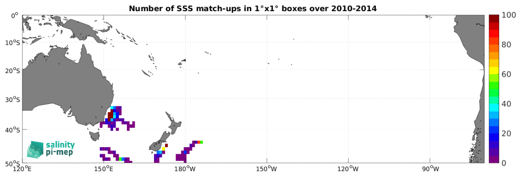
Figure 4: Number of SSS match-ups between Marine mammals SSS and the SMOS SSS L3 v9 - 9 Days (CATDS-CEC-LOCEAN) SSS product for the South Pacific Ocean Pi-MEP region over 1^\circ \times 1^\circ boxes and for the full satellite product period.
