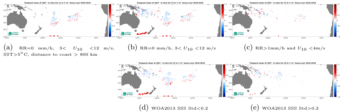
Figure 13: Temporal mean gridded over spatial boxes of size 1^\circ \times 1^\circ of \Delta\text{SSS} (SMOS SSS L3 v9 - 9 Days (CATDS-CEC-LOCEAN) - Surface drifters) for 5 different subdatasets corresponding to:RR=0 mm/h, 3 < U_{10} < 12 m/s, SST >5^\circ\text{C} , distance to coast > 800 km (a), RR=0 mm/h, 3 < U_{10} < 12 m/s (b), RR >1 mm/h and U_{10} < 4 m/s (c), WOA2013 SSS Std <0.2 (d), WOA2013 SSS Std >0.2 (e).
