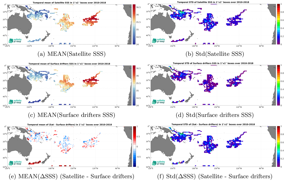
Figure 5: Temporal mean (left) and Std (right) of SSS from SMOS SSS L3 v9 - 9 Days (CATDS-CEC-LOCEAN) (top), Surface drifters (middle), and of \Delta SSS (Satellite - Surface drifters). Only match-up pairs are used to generate these maps.
