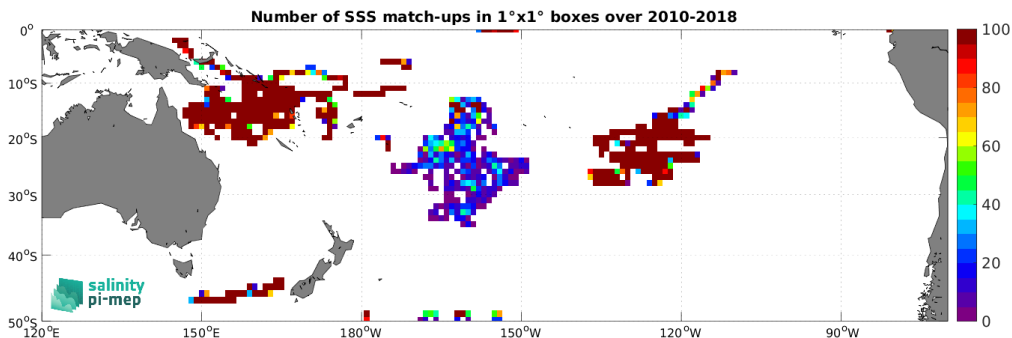
Figure 3: Number of SSS match-ups between Surface drifters SSS and the SMOS SSS L3 v9 - 9 Days (CATDS-CEC-LOCEAN) SSS product for the South Pacific Ocean Pi-MEP region over 1^\circ \times 1^\circ boxes and for the full satellite product period.
