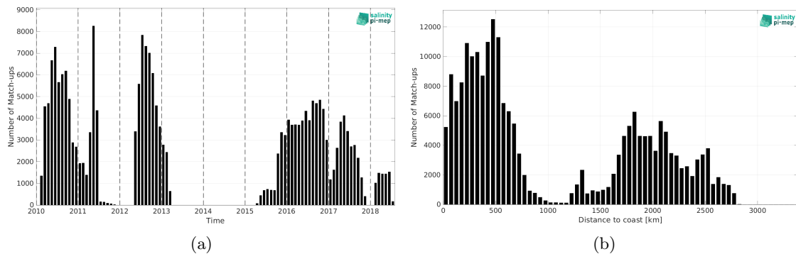
Figure 1: Number of match-ups between Surface drifters and SMOS SSS L3 v9 - 9 Days (CATDS-CEC-LOCEAN) SSS as a function of time (a) and as function of the distance to coast (b) over the South Pacific Ocean Pi-MEP region and for the full satellite product period.
