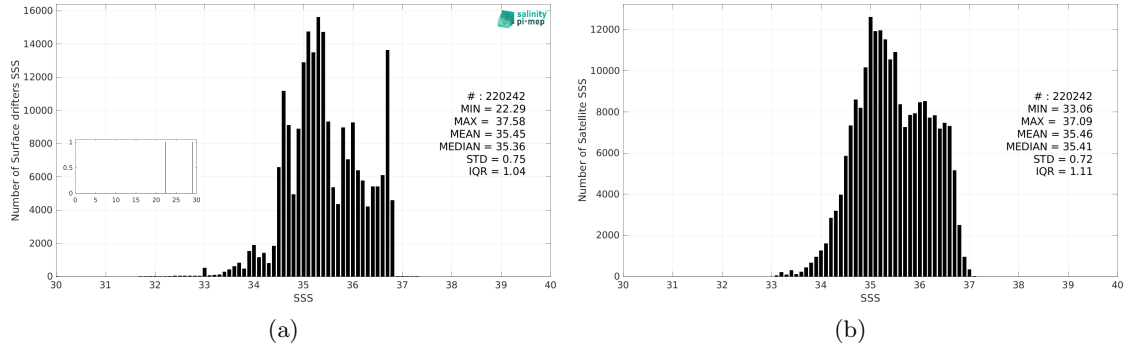
Figure 2: Histograms of SSS from Surface drifters (a) and SMOS SSS L3 v9 - 9 Days (CATDS-CEC-LOCEAN) (b) considering all match-up pairs per bins of 0.1 over the South Pacific Ocean Pi-MEP region and for the full satellite product period.
