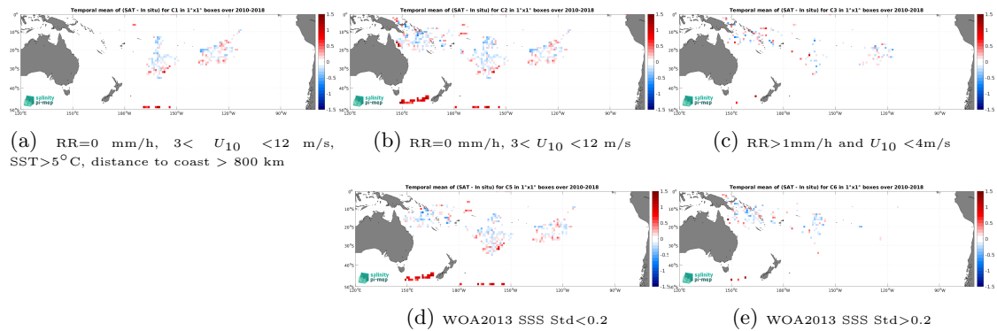
Figure 11: Temporal mean gridded over spatial boxes of size 1^\circ \times 1^\circ of \Delta SSS (SMOS SSS L3 v9 - 9 Days (CATDS-CEC-LOCEAN) - Surface drifters) for 5 different subdatasets corresponding to:RR=0 mm/h, 3 < U_{10} < 12 m/s, SST >5^\circ\text{C} , distance to coast > 800 km (a), RR=0 mm/h, 3 < U_{10} < 12 m/s (b), RR >1 mm/h and U_{10} < 4 m/s (c), WOA2013 SSS Std <0.2 (d), WOA2013 SSS Std >0.2 (e).
