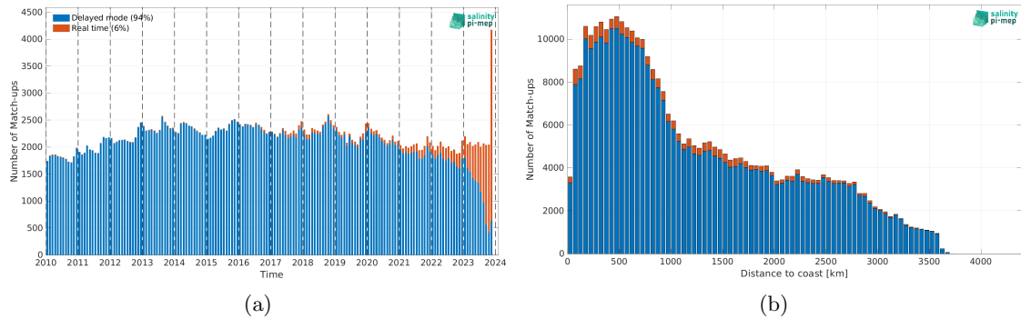
Figure 2: Number of match-ups between Argo and SMOS SSS L3 v9 - 9 Days (CATDS-CEC-LOCEAN) SSS as a function of time (a) and as function of the distance to coast (b) over the South Pacific Ocean Pi-MEP region and for the full satellite product period.
