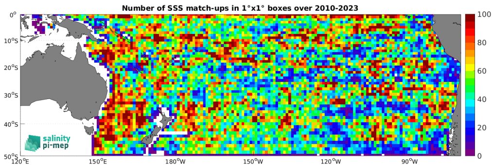
Figure 5: Number of SSS match-ups between Argo SSS and the SMOS SSS L3 v9 - 9 Days (CATDS-CEC-LOCEAN) SSS product for the South Pacific Ocean Pi-MEP region over 1^\circ \times 1^\circ boxes and for the full satellite product period.
