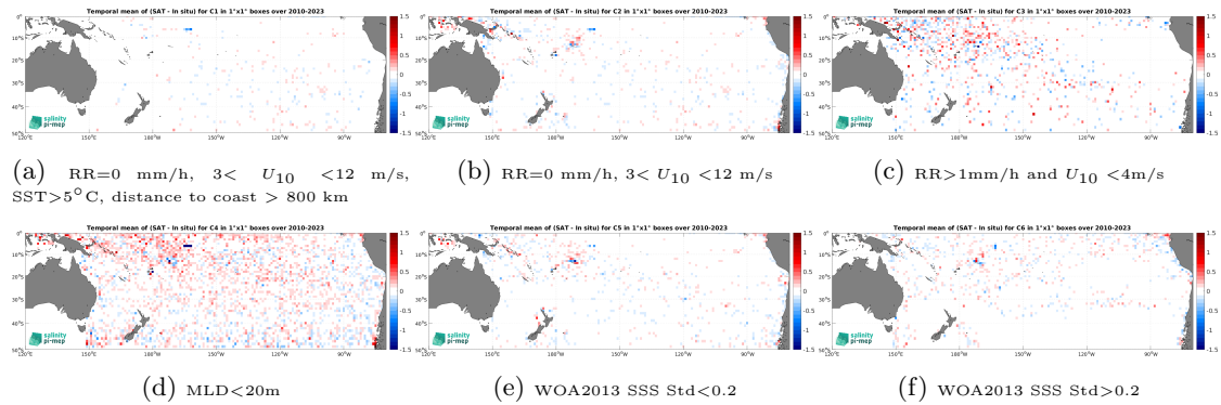
Figure 14: Temporal mean gridded over spatial boxes of size 1^\circ \times 1^\circ of \Delta SSS (SMOS SSS L3 v9 - 9 Days (CATDS-CEC-LOCEAN) - Argo) for 6 different subdatasets corresponding to:RR=0 mm/h, 3 < U_{10} < 12 m/s, SST >5^\circ C, distance to coast > 800 km (a), RR=0 mm/h, 3 < U_{10} < 12 m/s (b), RR >1 mm/h and U_{10} < 4 m/s (c),MLD <20 m (d),WOA2013 SSS Std <0.2 (e),WOA2013 SSS Std >0.2 (f).
