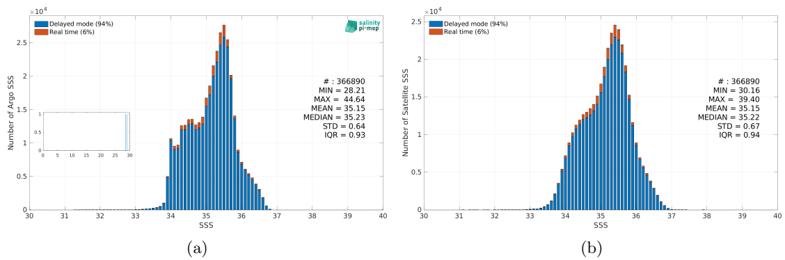
Figure 3: Histograms of SSS from Argo (a) and SMOS SSS L3 v9 - 9 Days (CATDS-CEC-LOCEAN) (b) considering all match-up pairs per bins of 0.1 over the South Pacific Ocean Pi-MEP region and for the full satellite product period.
