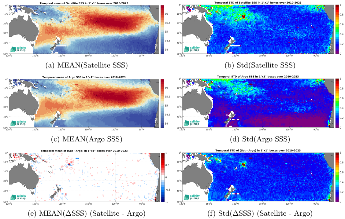
Figure 7: Temporal mean (left) and Std (right) of SSS from SMOS SSS L3 v9 - 9 Days (CATDS-CEC-LOCEAN) (top), Argo (middle), and of \Delta SSS (Satellite - Argo). Only match-up pairs are used to generate these maps.
