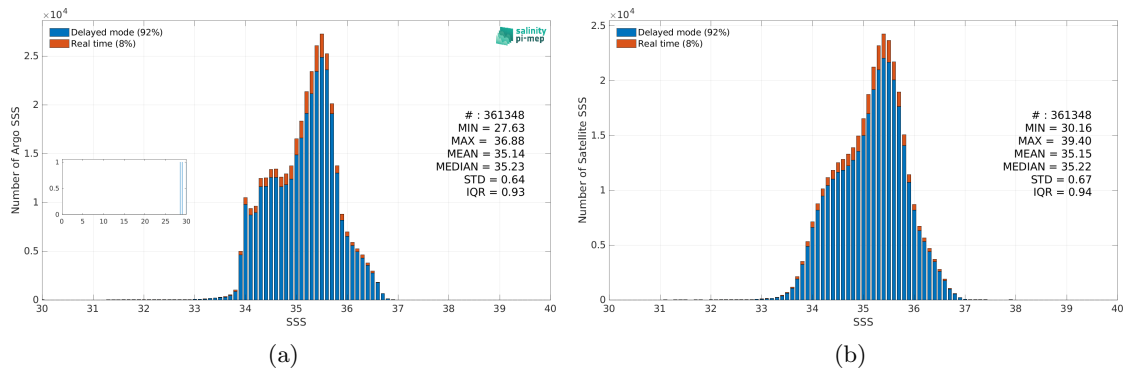
Figure 2: Histograms of SSS from Argo (a) and SMOS SSS L3 v9 - 9 Days (CATDS-CEC-LOCEAN) (b) considering all match-up pairs per bins of 0.1 over the South Pacific Ocean Pi-MEP region and for the full satellite product period.
