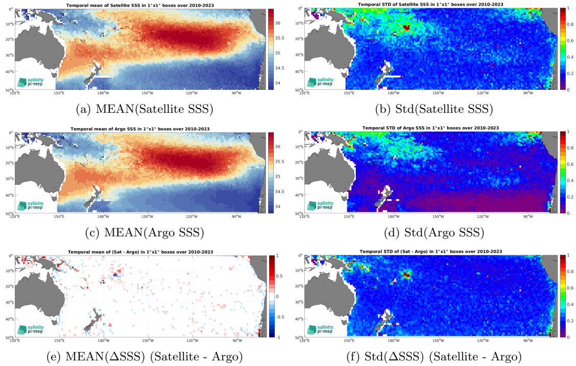
Figure 6: Temporal mean (left) and Std (right) of SSS from SMOS SSS L3 v9 - 9 Days (CATDS-CEC-LOCEAN) (top), Argo (middle), and of \Delta SSS (Satellite - Argo). Only match-up pairs are used to generate these maps.
