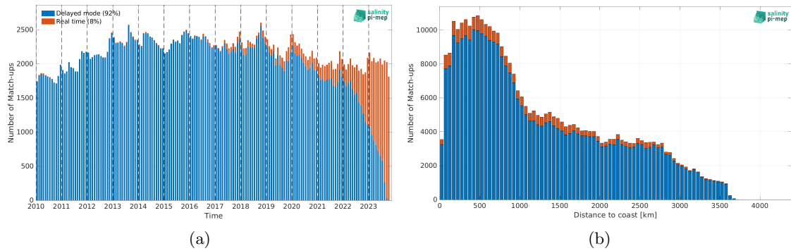
Figure 1: Number of match-ups between Argo and SMOS SSS L3 v9 - 9 Days (CATDS-CEC-LOCEAN) SSS as a function of time (a) and as function of the distance to coast (b) over the South Pacific Ocean Pi-MEP region and for the full satellite product period.
