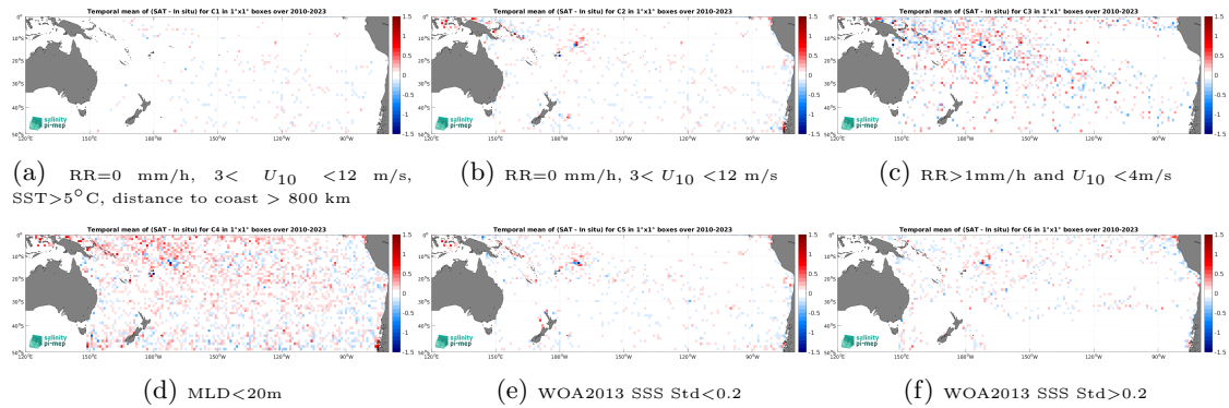
Figure 12: Temporal mean gridded over spatial boxes of size 1^\circ \times 1^\circ of \Delta SSS (SMOS SSS L3 v9 - 9 Days (CATDS-CEC-LOCEAN) - Argo) for 6 different subdatasets corresponding to:RR=0 mm/h, 3 < U_{10} < 12 m/s, SST >5^\circ\text{C} , distance to coast > 800 km (a), RR=0 mm/h, 3 < U_{10} < 12 m/s (b), RR >1 mm/h and U_{10} < 4 m/s (c),MLD <20 m (d),WOA2013 SSS Std <0.2 (e),WOA2013 SSS Std >0.2 (f).
