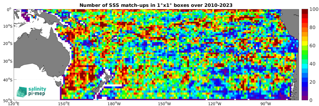
Figure 4: Number of SSS match-ups between Argo SSS and the SMOS SSS L3 v9 - 9 Days (CATDS-CEC-LOCEAN) SSS product for the South Pacific Ocean Pi-MEP region over 1^\circ \times 1^\circ boxes and for the full satellite product period.
