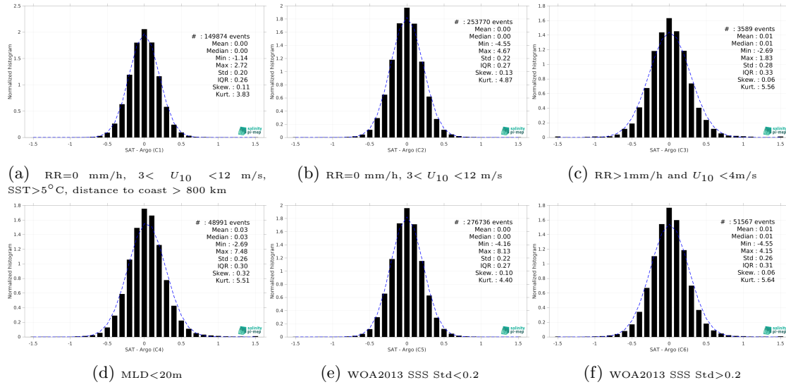
Figure 13: Normalized histogram of \Delta SSS (SMOS SSS L3 v9 - 9 Days (CATDS-CEC-LOCEAN) - Argo) for 6 different subdatasets corresponding to: RR=0 mm/h, 3 < U_{10} < 12 m/s, SST > 5°C, distance to coast > 800 km (a), RR=0 mm/h, 3 < U_{10} < 12 m/s (b), RR > 1mm/h and U_{10} < 4 m/s (c), MLD < 20m (d), WOA2013 SSS Std < 0.2 (e), WOA2013 SSS Std > 0.2 (f).
