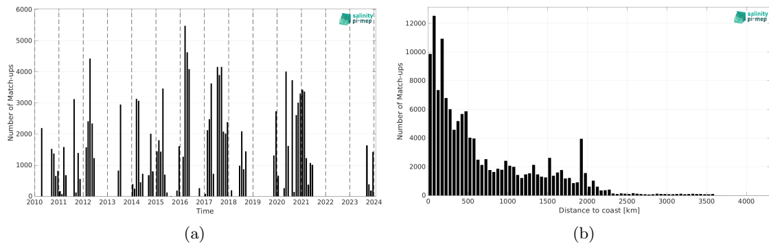
Figure 2: Number of match-ups between TSG (SAMOS) and SMOS SSS L3 v9 - 18 Days (CATDS-CEC-LOCEAN) SSS as a function of time (a) and as function of the distance to coast (b) over the South Pacific Ocean Pi-MEP region and for the full satellite product period.
