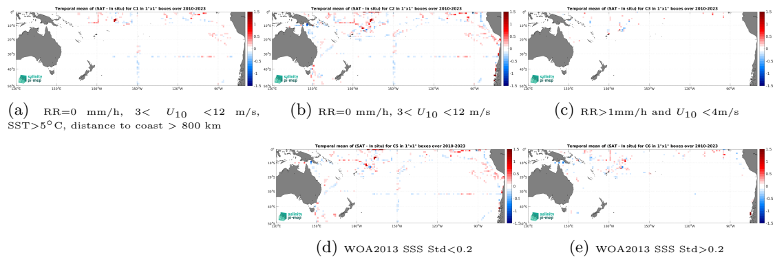
Figure 14: Temporal mean gridded over spatial boxes of size 1^\circ \times 1^\circ of \Delta SSS (SMOS SSS L3 v9 - 18 Days (CATDS-CEC-LOCEAN) - TSG (SAMOS)) for 5 different subdatasets corresponding to:RR=0 mm/h, 3 < U_{10} < 12 m/s, SST >5^\circ C, distance to coast > 800 km (a), RR=0 mm/h, 3 < U_{10} < 12 m/s (b), RR >1 mm/h and U_{10} < 4 m/s (c), WOA2013 SSS Std <0.2 (d), WOA2013 SSS Std >0.2 (e).
