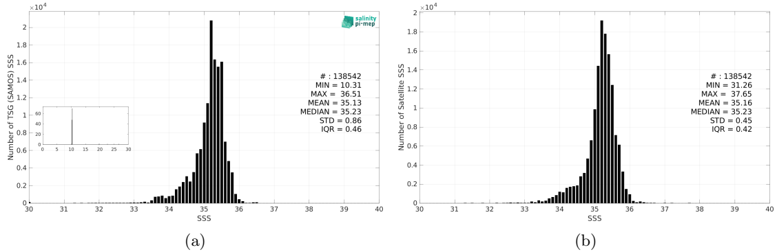
Figure 3: Histograms of SSS from TSG (SAMOS) (a) and SMOS SSS L3 v9 - 18 Days (CATDS-CEC-LOCEAN) (b) considering all match-up pairs per bins of 0.1 over the South Pacific Ocean Pi-MEP region and for the full satellite product period.
