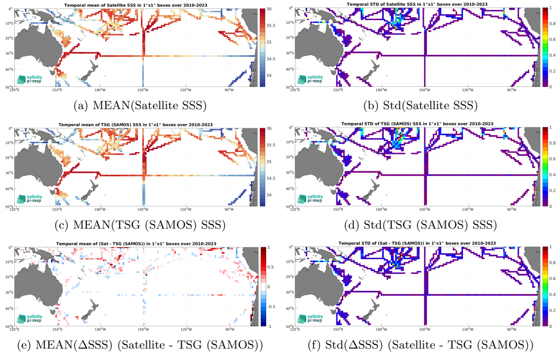
Figure 7: Temporal mean (left) and Std (right) of SSS from SMOS SSS L3 v9 - 18 Days (CATDS-CEC-LOCEAN) (top), TSG (SAMOS) (middle), and of \Delta SSS (Satellite - TSG (SAMOS)). Only match-up pairs are used to generate these maps.
