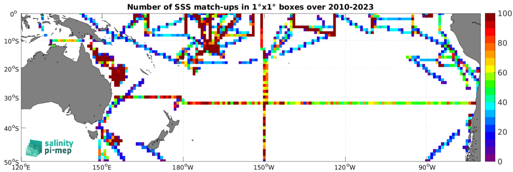
Figure 5: Number of SSS match-ups between TSG (SAMOS) SSS and the SMOS SSS L3 v9 - 18 Days (CATDS-CEC-LOCEAN) SSS product for the South Pacific Ocean Pi-MEP region over 1^\circ \times 1^\circ boxes and for the full satellite product period.
