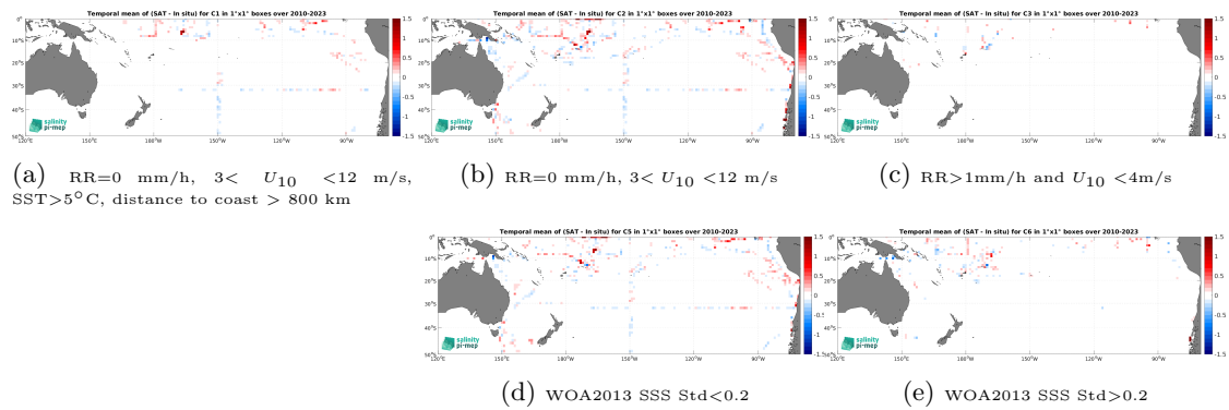
Figure 14: Temporal mean gridded over spatial boxes of size 1^\circ \times 1^\circ of \Delta\text{SSS} (SMOS SSS L3 v9 - 18 Days (CATDS-CEC-LOCEAN) - TSG (SAMOS)) for 5 different subdatasets corresponding to:RR=0 mm/h, 3 < U_{10} < 12 m/s, SST>5°C, distance to coast > 800 km (a), RR=0 mm/h, 3 < U_{10} < 12 m/s (b), RR>1mm/h and U_{10} < 4 m/s (c), WOA2013 SSS Std<0.2 (d), WOA2013 SSS Std>0.2 (e).
