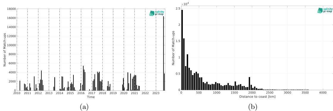
Figure 1: Number of match-ups between TSG (SAMOS) and SMOS SSS L3 v9 - 18 Days (CATDS-CEC-LOCEAN) SSS as a function of time (a) and as function of the distance to coast (b) over the South Pacific Ocean Pi-MEP region and for the full satellite product period.
