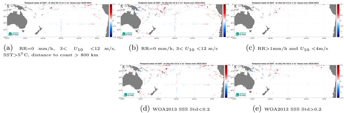
Figure 12: Temporal mean gridded over spatial boxes of size 1^\circ \times 1^\circ of \Delta SSS (SMOS SSS L3 v9 - 18 Days (CATDS-CEC-LOCEAN) - TSG (SAMOS)) for 5 different subdatasets corresponding to:RR=0 mm/h, 3 < U_{10} < 12 m/s, SST >5^\circ C, distance to coast > 800 km (a), RR=0 mm/h, 3 < U_{10} < 12 m/s (b), RR >1 mm/h and U_{10} < 4 m/s (c), WOA2013 SSS Std <0.2 (d), WOA2013 SSS Std >0.2 (e).
