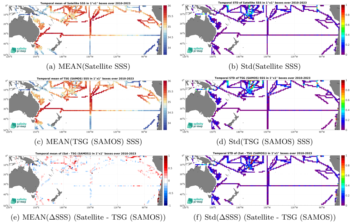
Figure 6: Temporal mean (left) and Std (right) of SSS from SMOS SSS L3 v9 - 18 Days (CATDS-CEC-LOCEAN) (top), TSG (SAMOS) (middle), and of \Delta SSS (Satellite - TSG (SAMOS)). Only match-up pairs are used to generate these maps.
