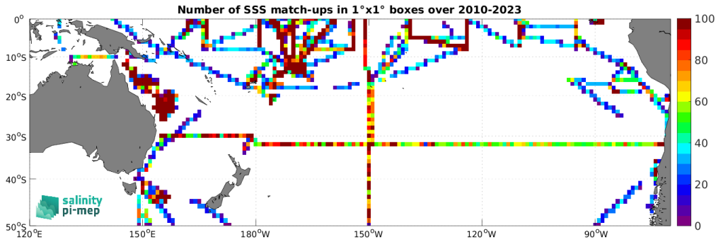
Figure 4: Number of SSS match-ups between TSG (SAMOS) SSS and the SMOS SSS L3 v9 - 18 Days (CATDS-CEC-LOCEAN) SSS product for the South Pacific Ocean Pi-MEP region over 1^\circ \times 1^\circ boxes and for the full satellite product period.
