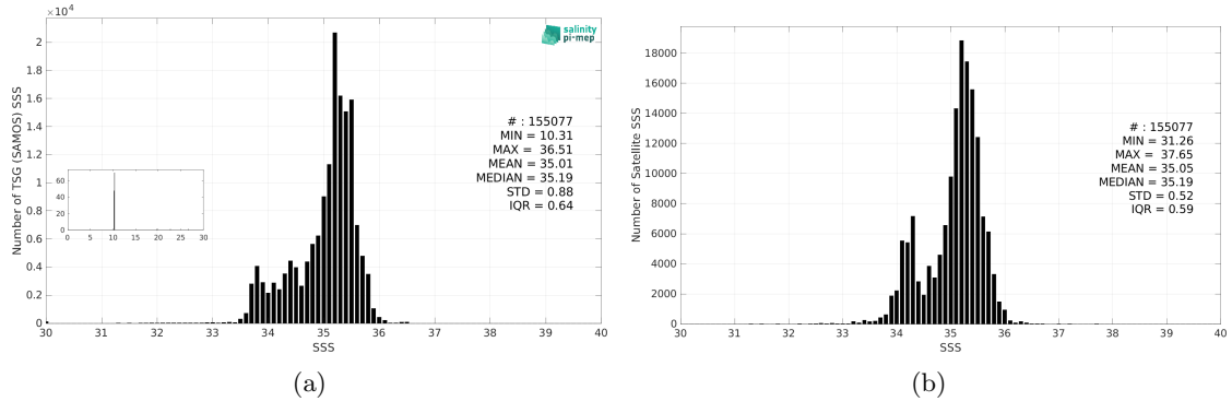
Figure 2: Histograms of SSS from TSG (SAMOS) (a) and SMOS SSS L3 v9 - 18 Days (CATDS-CEC-LOCEAN) (b) considering all match-up pairs per bins of 0.1 over the South Pacific Ocean Pi-MEP region and for the full satellite product period.
