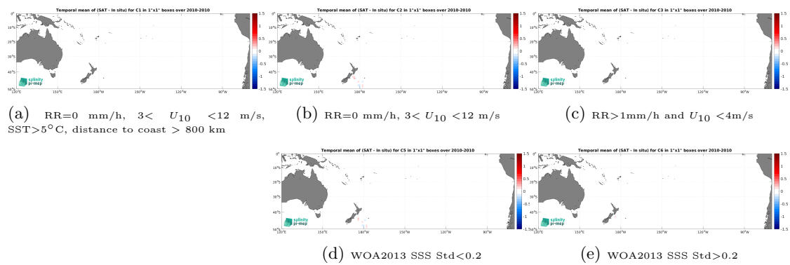
Figure 14: Temporal mean gridded over spatial boxes of size 1^\circ \times 1^\circ of \Delta SSS (SMOS SSS L3 v9 - 18 Days (CATDS-CEC-LOCEAN) - TSG (Polarstern)) for 5 different subdatasets corresponding to:RR=0 mm/h, 3 < U_{10} < 12 m/s, SST >5^\circ C, distance to coast > 800 km (a), RR=0 mm/h, 3 < U_{10} < 12 m/s (b), RR >1 mm/h and U_{10} < 4 m/s (c), WOA2013 SSS Std <0.2 (d), WOA2013 SSS Std >0.2 (e).
