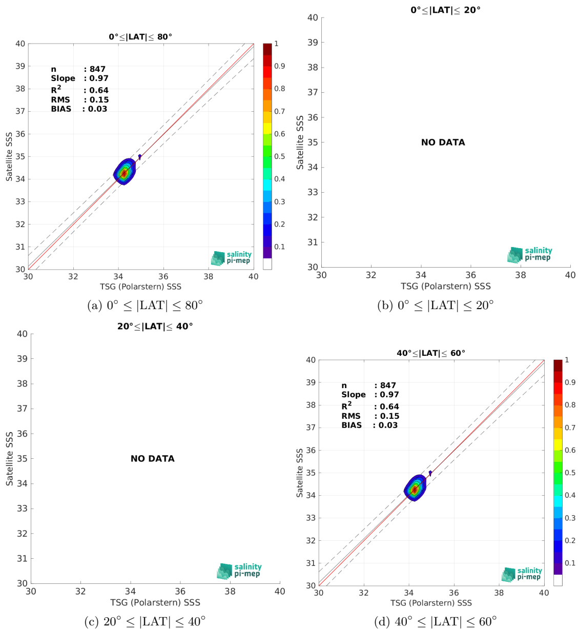
Figure 10: Contour maps of the concentration of SMOS SSS L3 v9 - 18 Days (CATDS-CEC-LOCEAN) SSS (y-axis) versus TSG (Polarstern) SSS (x-axis) at match-up pairs for different latitude bands. For each plot, the red line shows x=y . The black thin and dashed lines indicate a linear fit through the data cloud and the \pm 95\% confidence levels, respectively. The number match-up pairs n , the slope and R^2 coefficient of the linear fit, the root mean square (RMS) and the mean bias between satellite and in situ data are indicated for each latitude band in each plots.
