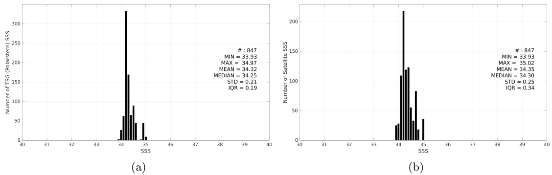
Figure 3: Histograms of SSS from TSG (Polarstern) (a) and SMOS SSS L3 v9 - 18 Days (CATDS-CEC-LOCEAN) (b) considering all match-up pairs per bins of 0.1 over the South Pacific Ocean Pi-MEP region and for the full satellite product period.
