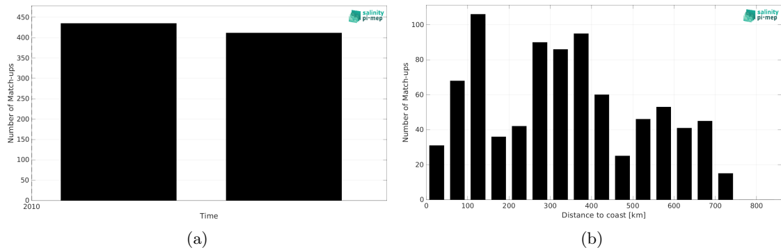
Figure 2: Number of match-ups between TSG (Polarstern) and SMOS SSS L3 v9 - 18 Days (CATDS-CEC-LOCEAN) SSS as a function of time (a) and as function of the distance to coast (b) over the South Pacific Ocean Pi-MEP region and for the full satellite product period.
