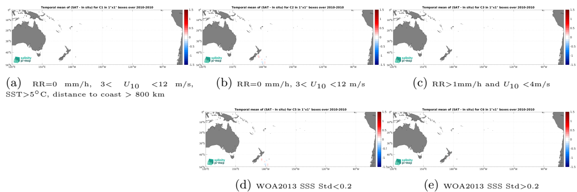
Figure 14: Temporal mean gridded over spatial boxes of size 1^\circ \times 1^\circ of \Delta\text{SSS} (SMOS SSS L3 v9 - 18 Days (CATDS-CEC-LOCEAN) - TSG (Polarstern)) for 5 different subdatasets corresponding to:RR=0 mm/h, 3 < U_{10} < 12 m/s, SST>5°C, distance to coast > 800 km (a), RR=0 mm/h, 3 < U_{10} < 12 m/s (b), RR>1mm/h and U_{10} < 4 m/s (c), WOA2013 SSS Std<0.2 (d), WOA2013 SSS Std>0.2 (e).
